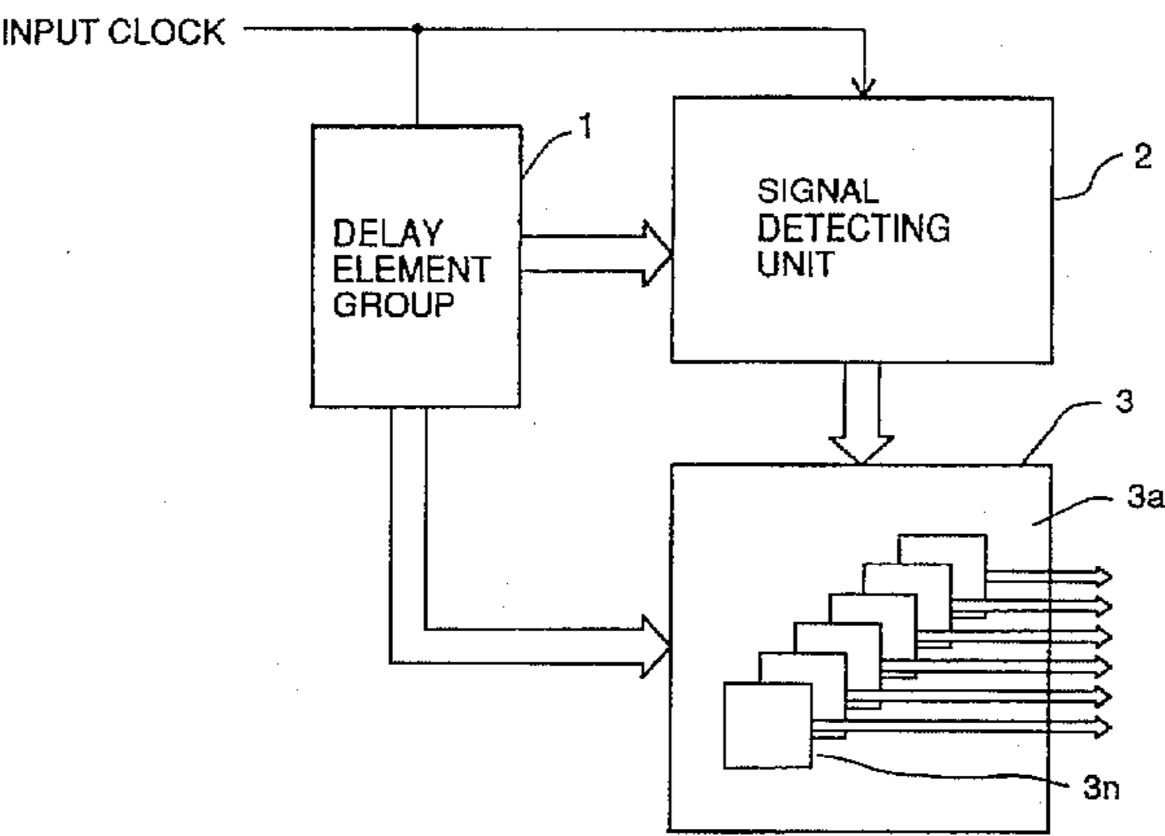
3a-3n : OUTPUT SIGNAL DETERMINING UNIT
