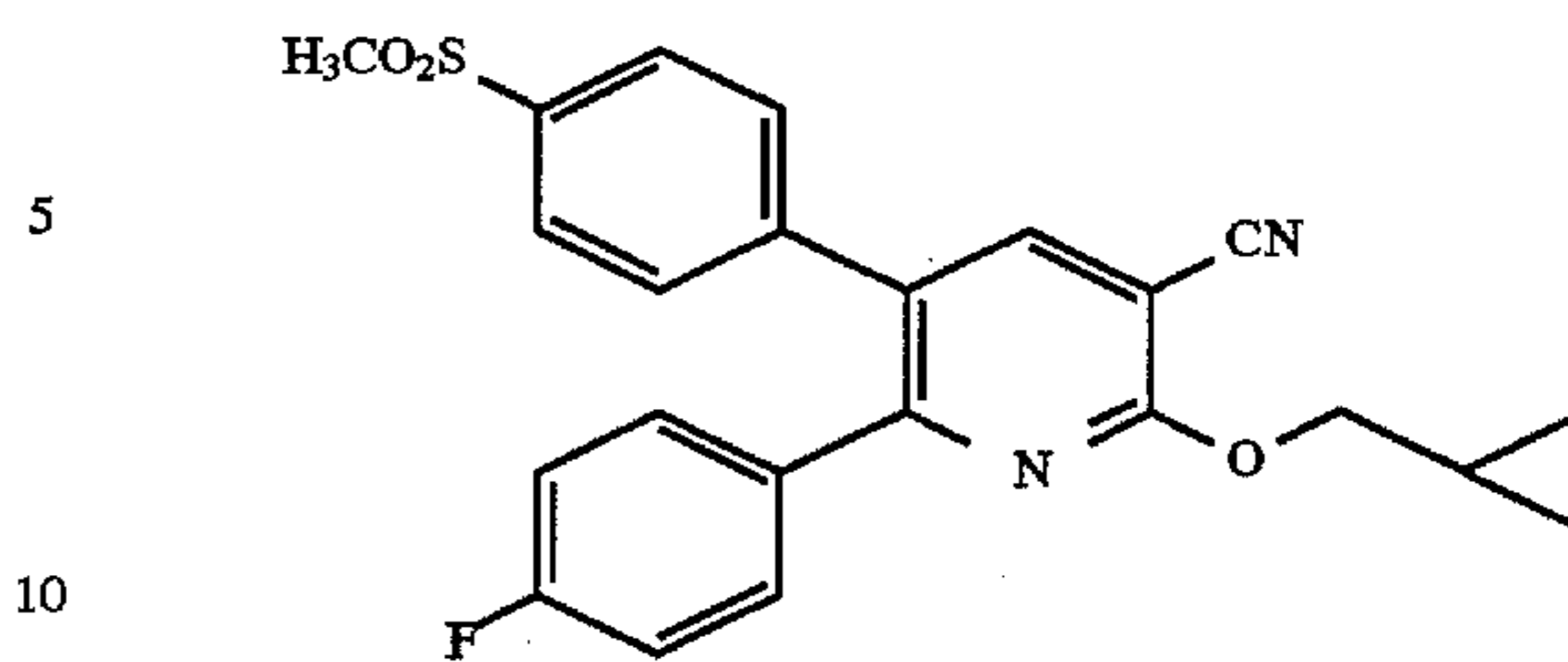
2-Cyclopropylmethoxy-6-(4-fluorophenyl)-5-[4-(methylsulfonyl)phenyl]pyridine-3-carbonitrile
