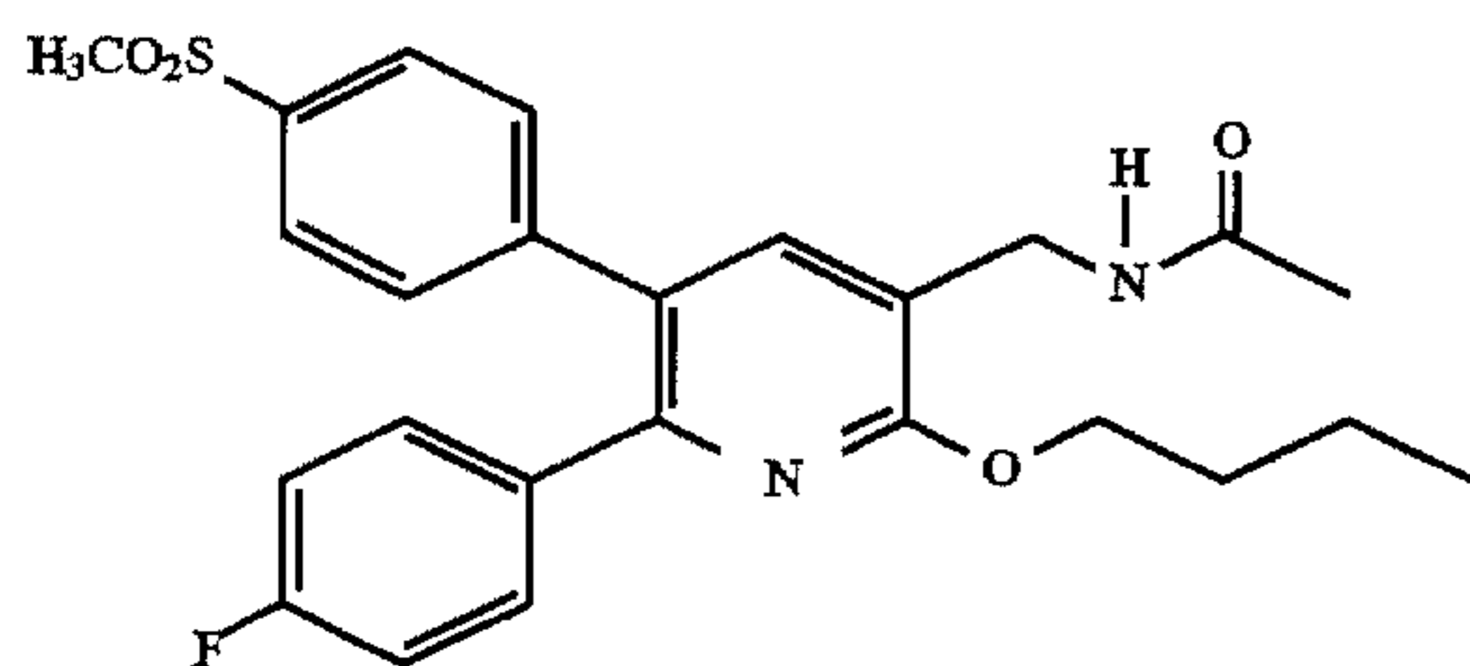
2-Butoxy-6-(4-fluorophenyl)-3-(N-methylcarbonylamino)methyl-5-[4-(methylsulfonyl)phenyl]pyridine
