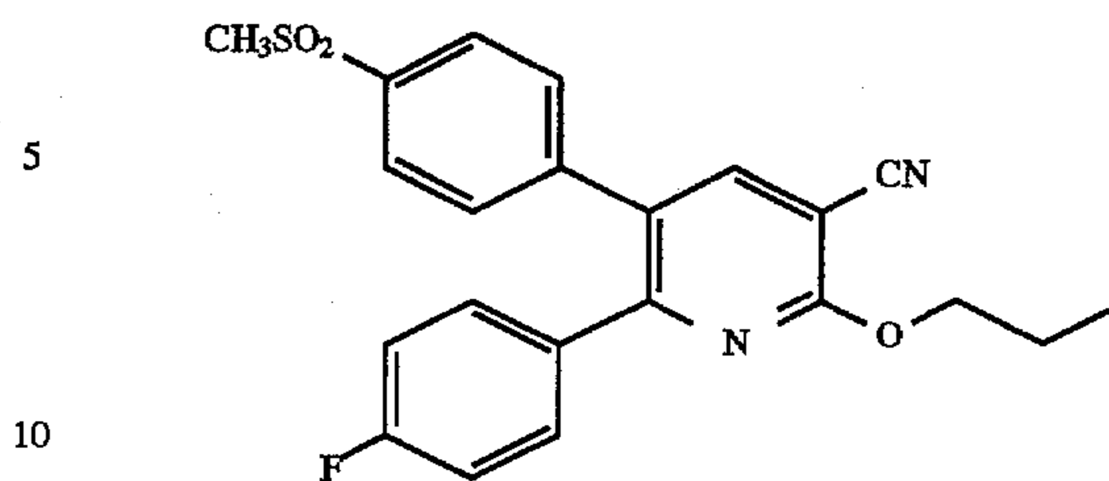
6-(4-Fluorophenyl)-5-[4-(methylsulfonyl)phenyl]-2-propoxypyridine-3-carbonitrile
