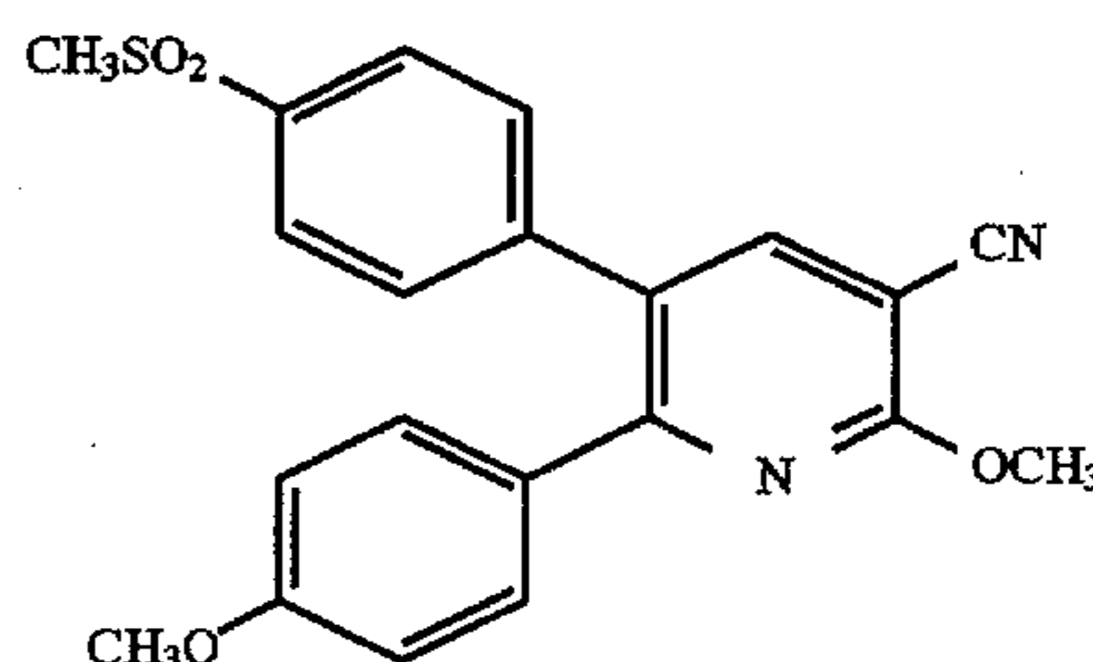
2-Methoxy-6-(4-methoxyphenyl)-5-[4-(methylsulfonyl)phenyl]pyridine-3-carbonitrile
