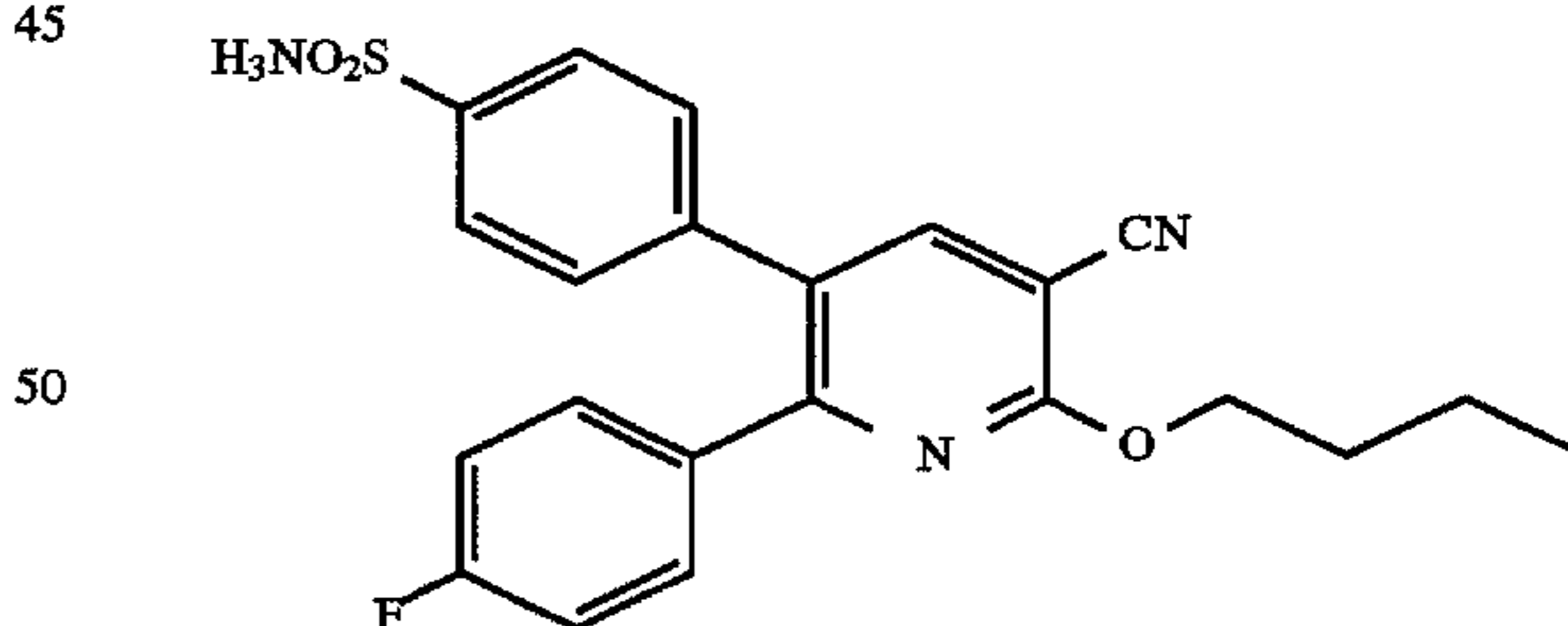
4-[6-butoxy-4-cyano-2-(4-Fluorophenyl)-3-pyridine] benzenesulfonamide
