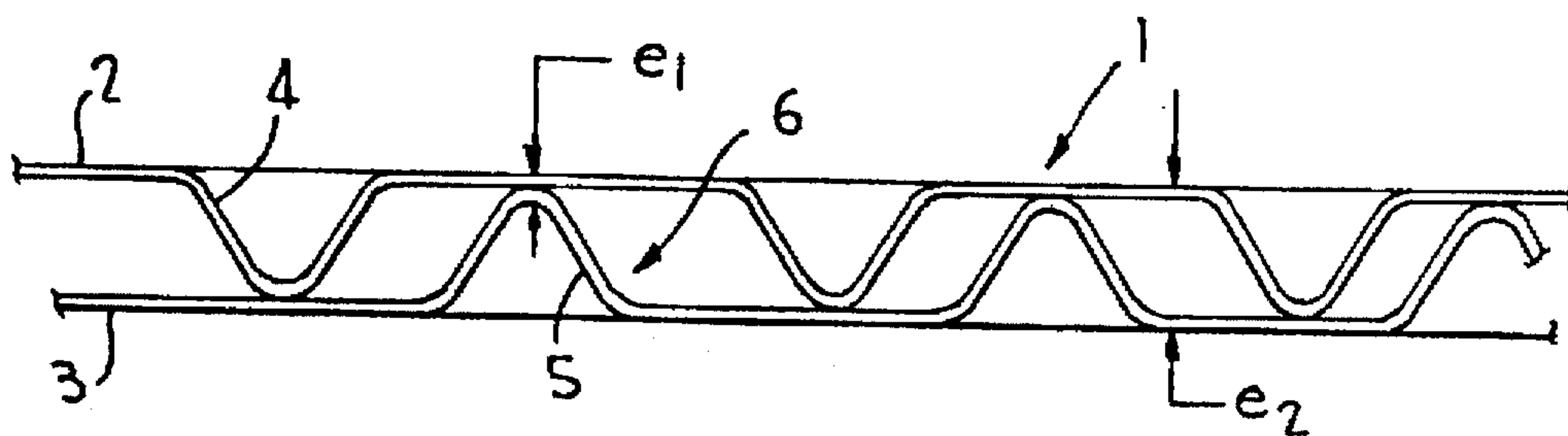
FIG. 2 (PRIOR ART)
