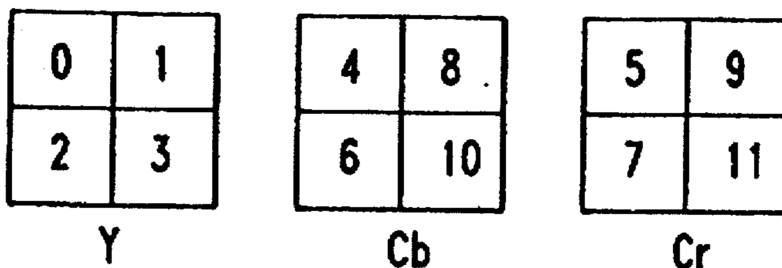
4:4:4 Macroblock structure
