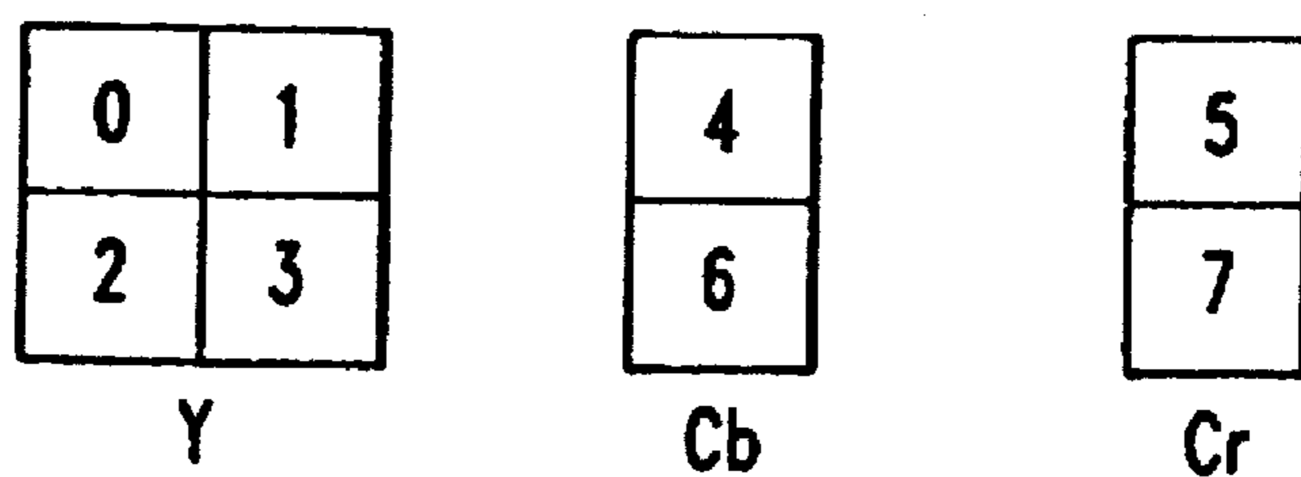
4:2:2 Macroblock structure
