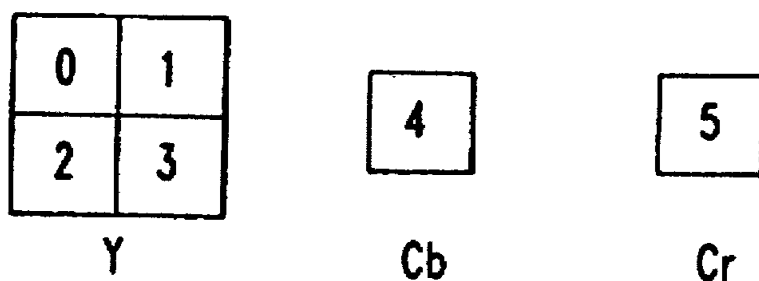
4:2:0 Macroblock structure
