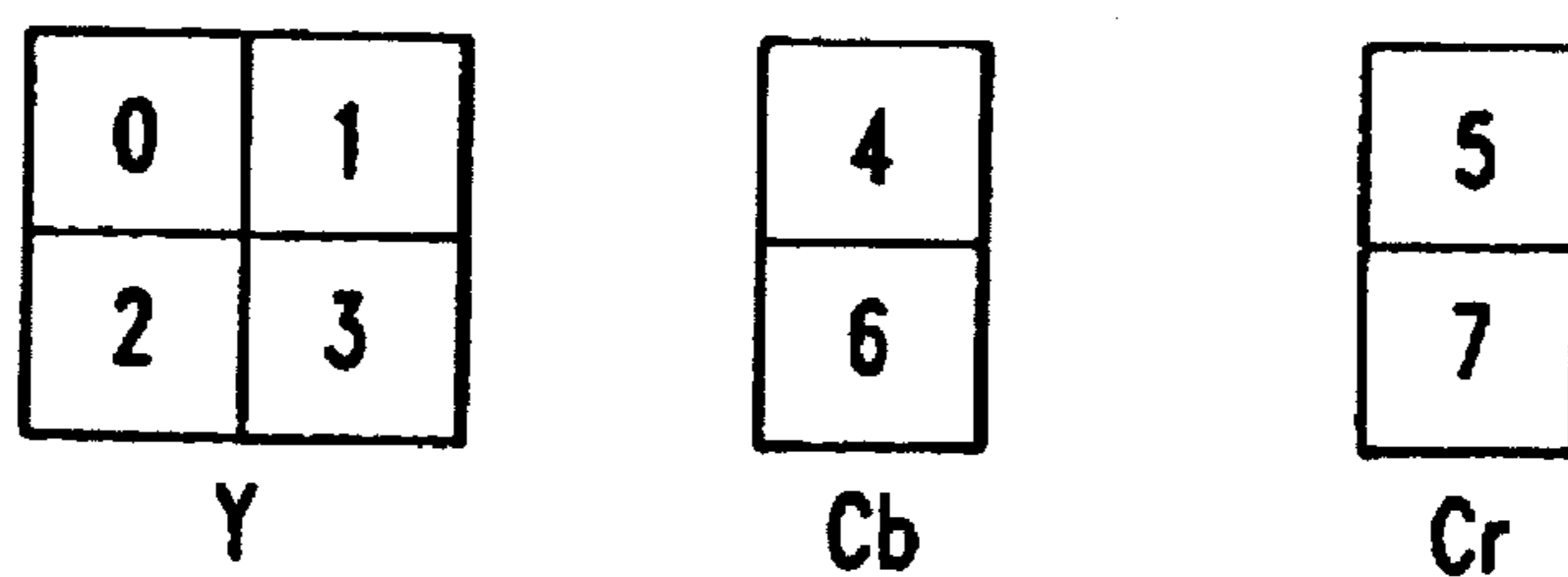
4:2:2 Macroblock structure
