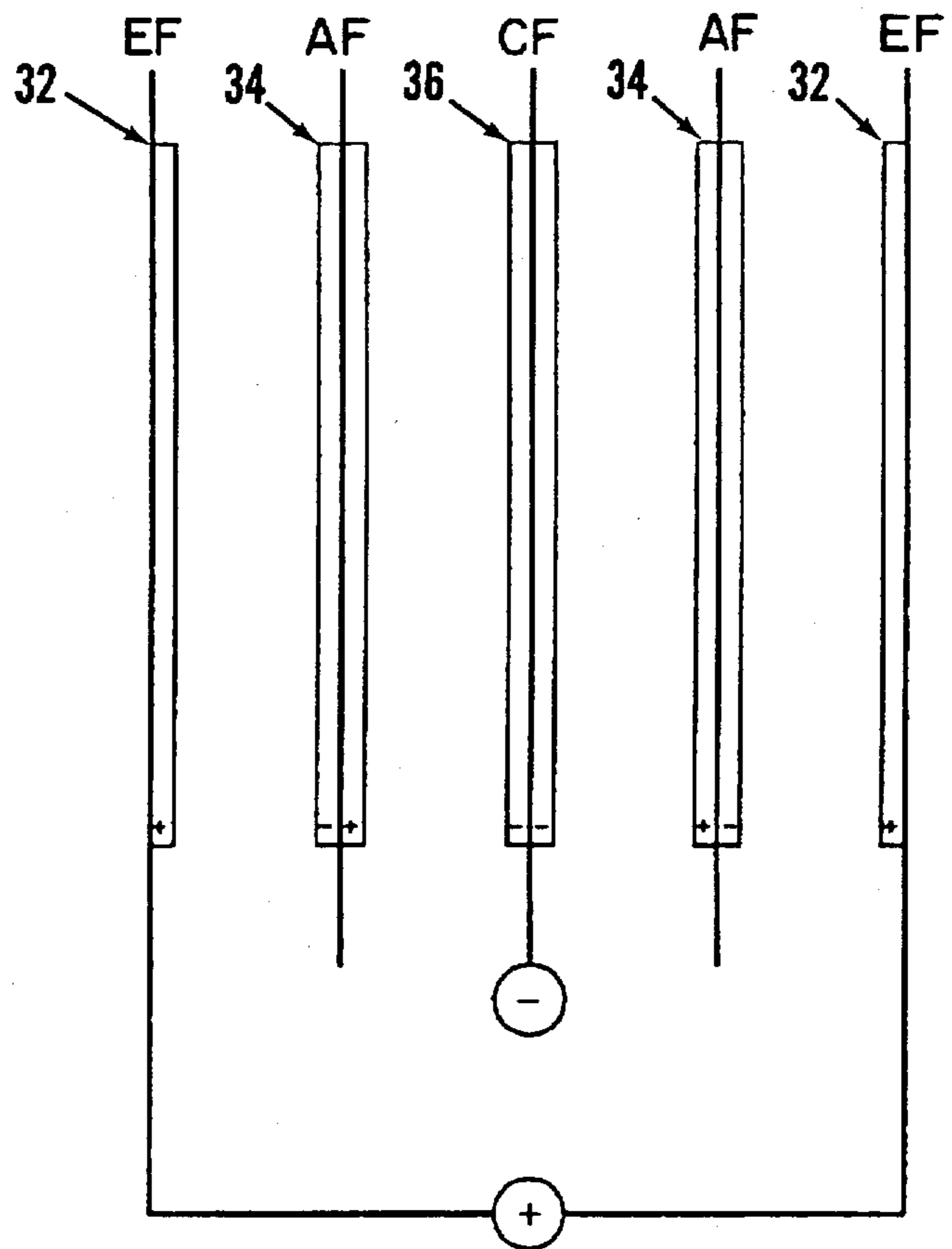
SERIES/PARALLEL
