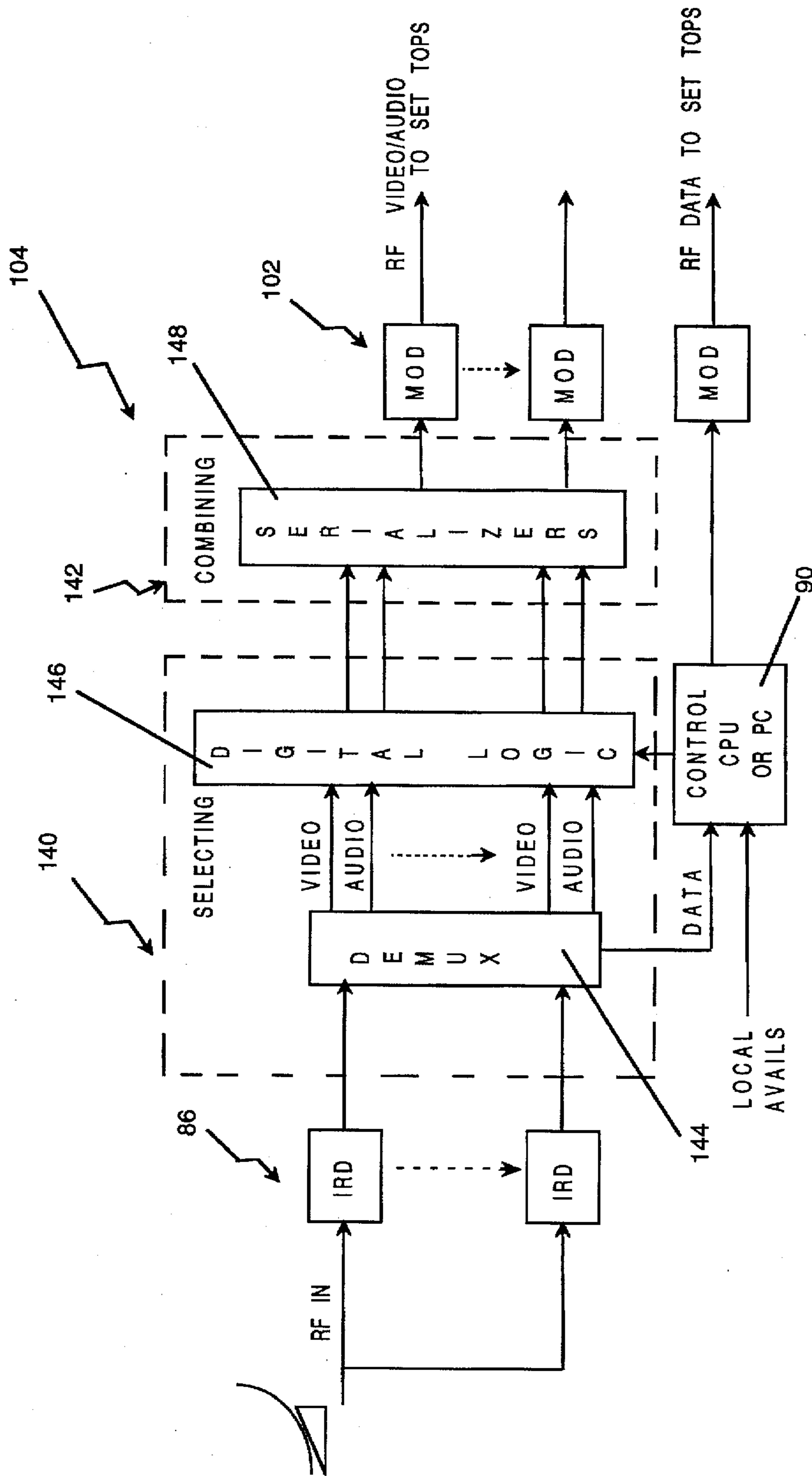
DIGITAL CABLE HEADEND WITH COMBINER
