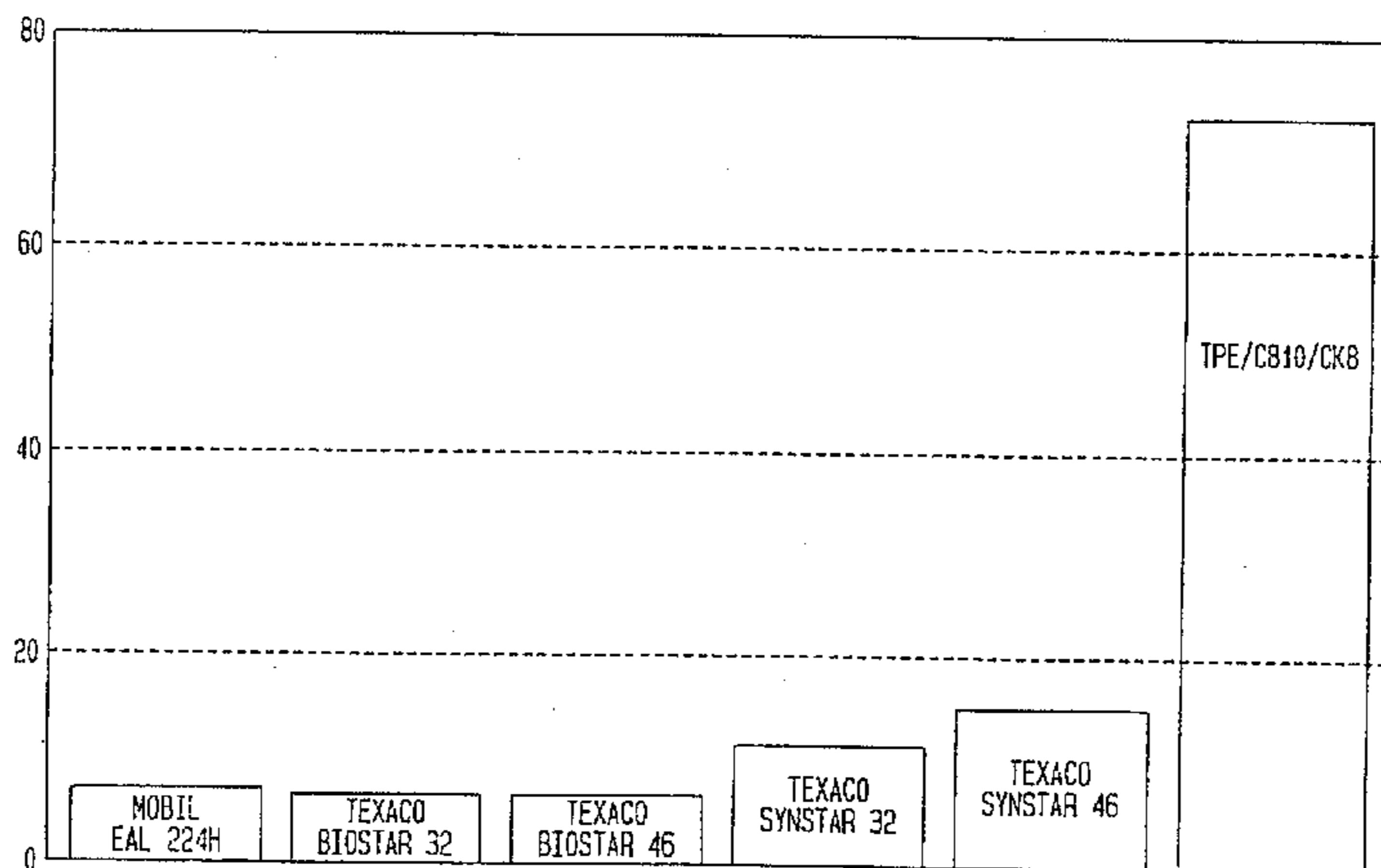
STABILITY OF FORMULATED OILS, HPDSC @ 200°C
