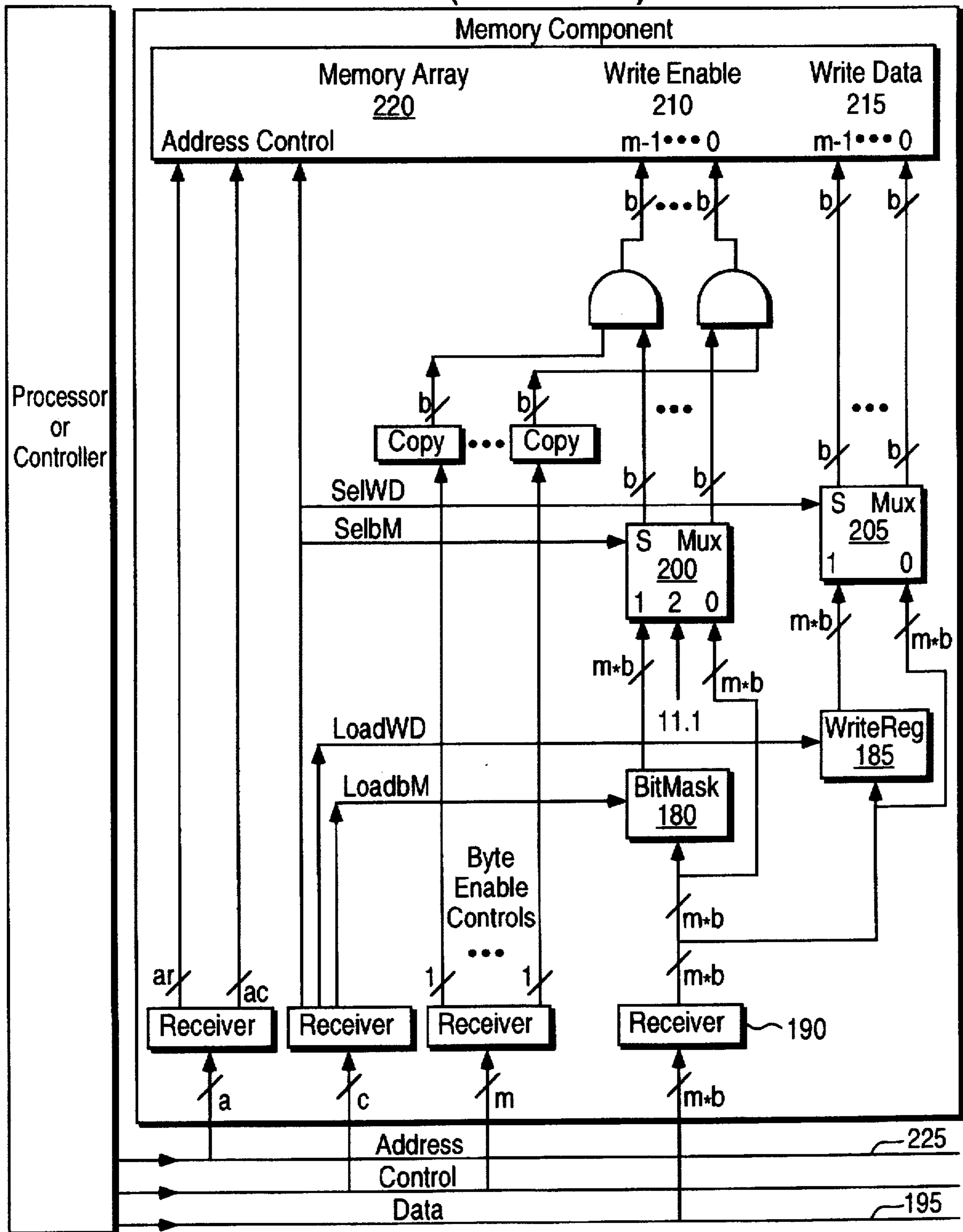
FIG. 5 (Prior Art)
