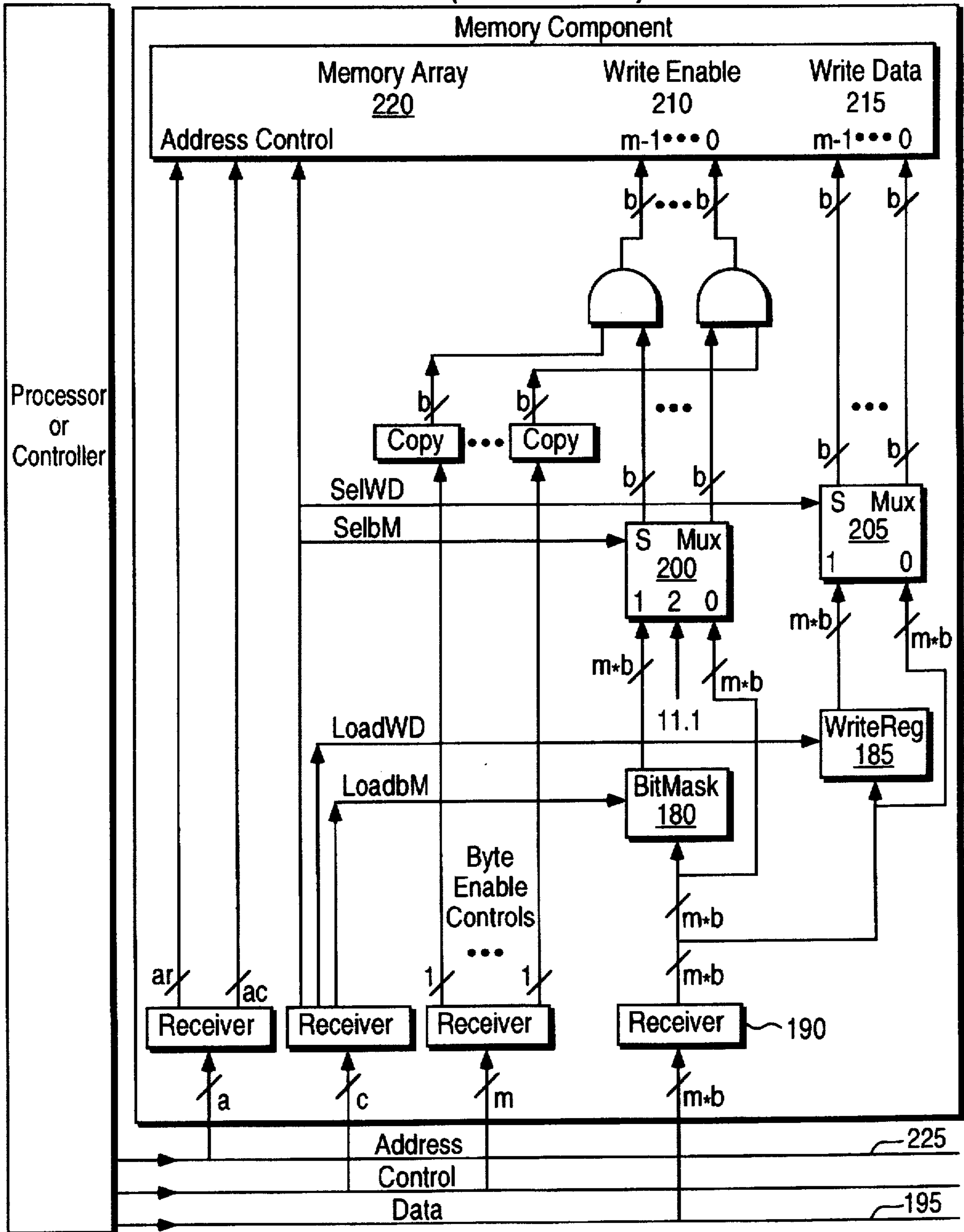
FIG. 5 (Prior Art)
