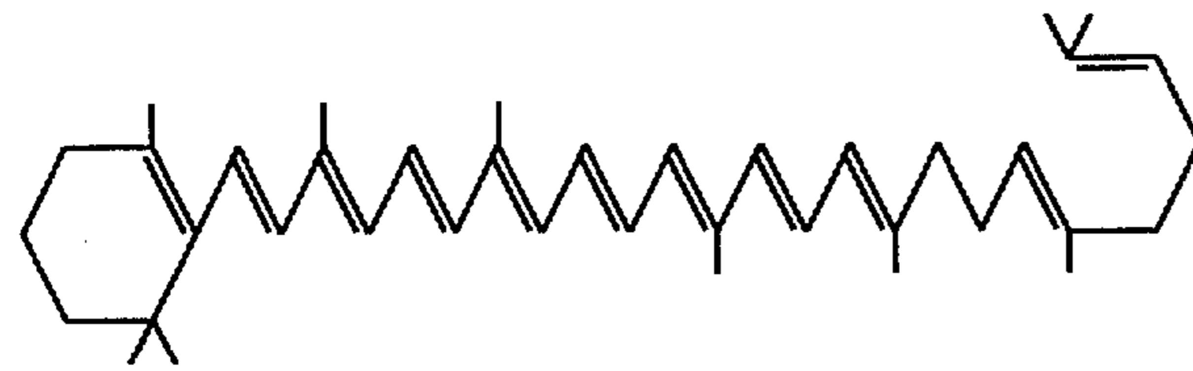
λ-ZEAXANTHIN
