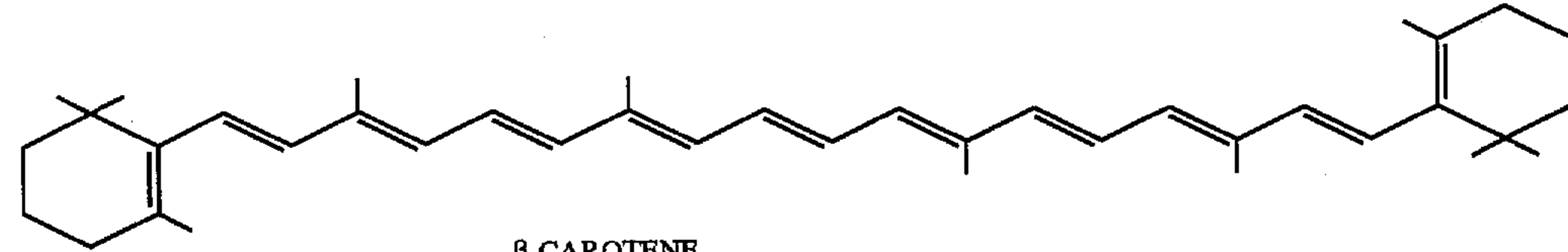
β-CAROTENE
