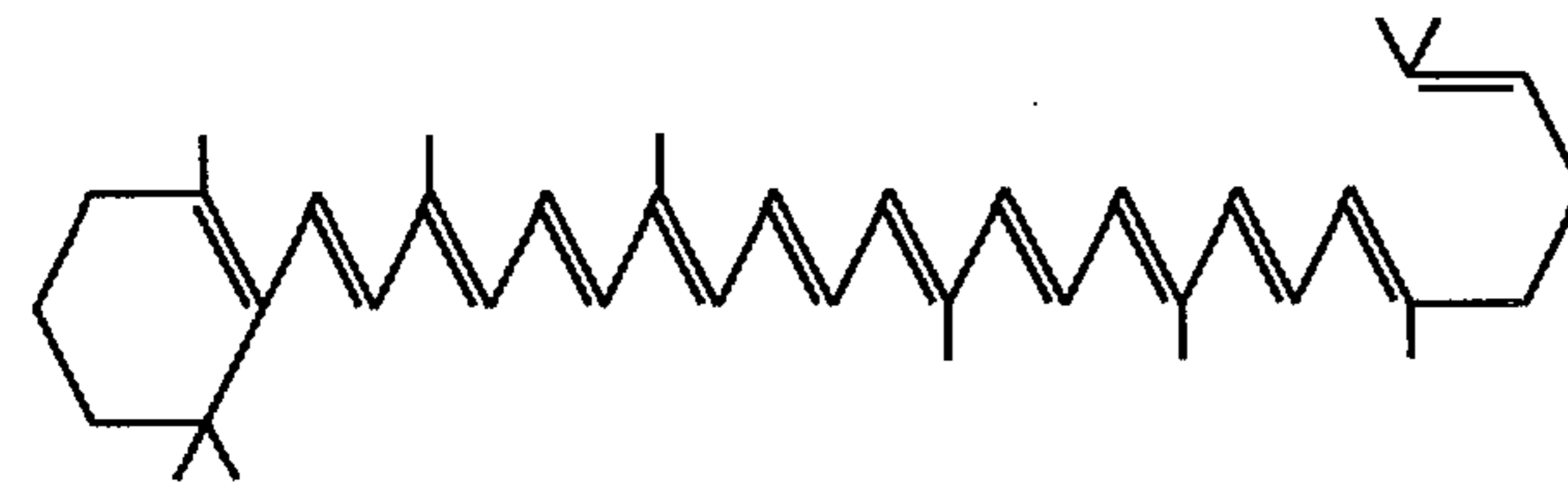
ν-CAROTENE
