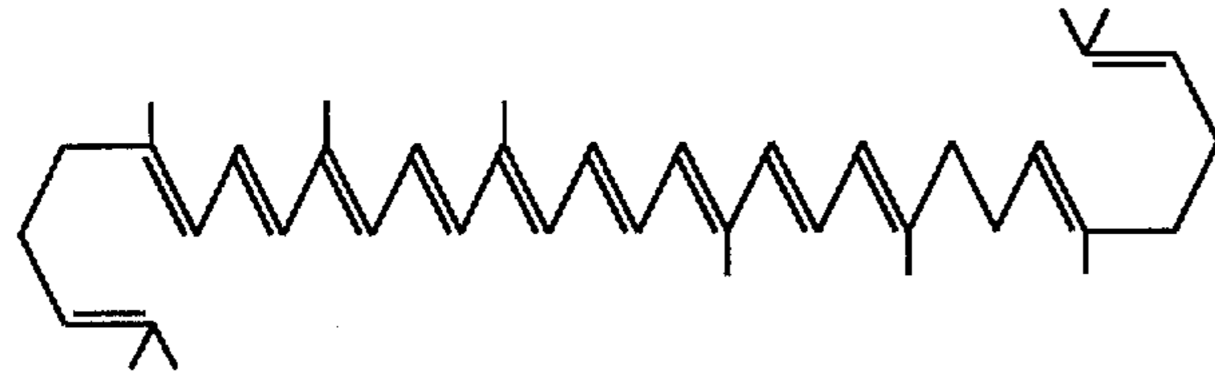
NEUROSPORENE
