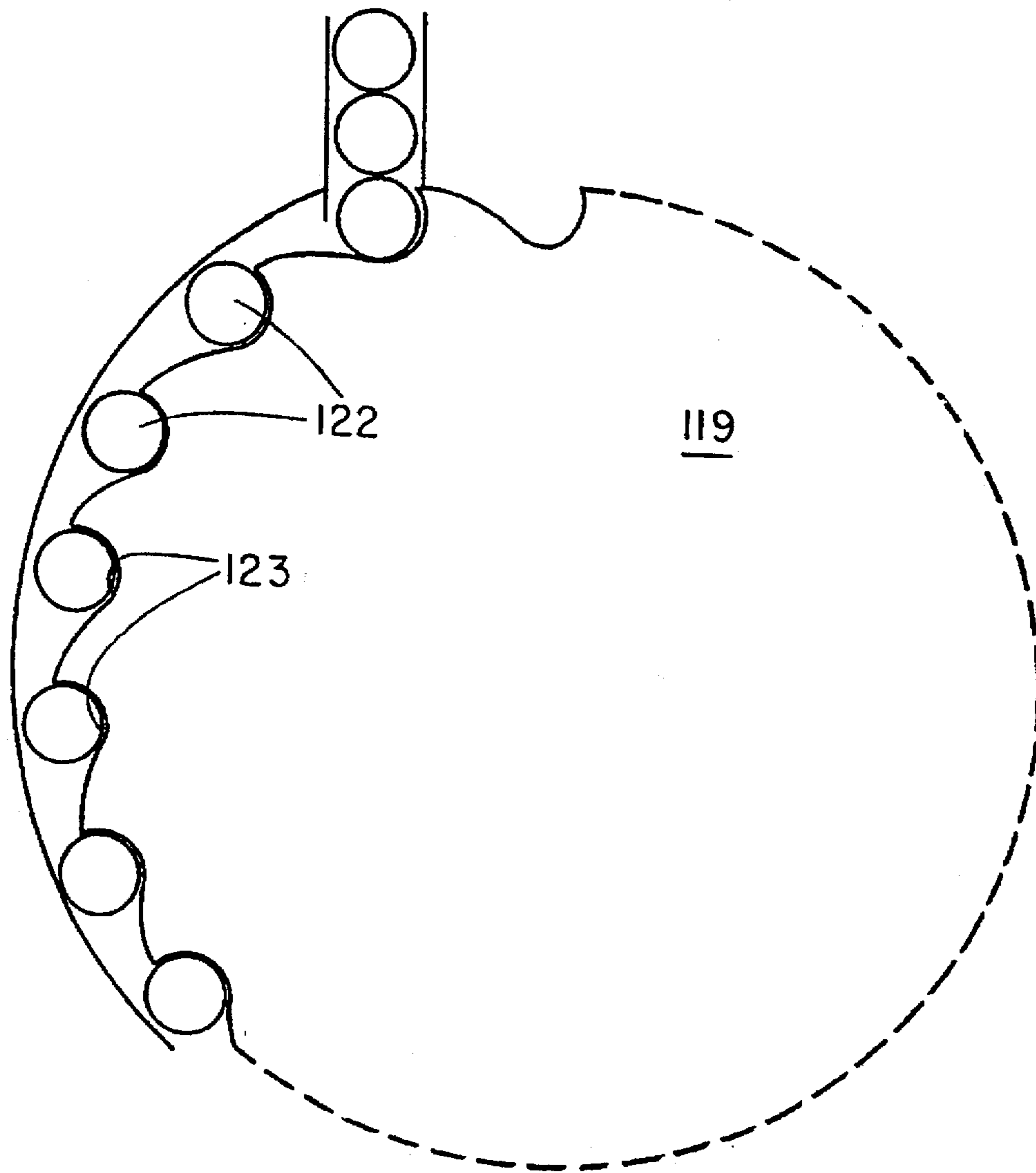
FIG. 9 (PRIOR ART)
