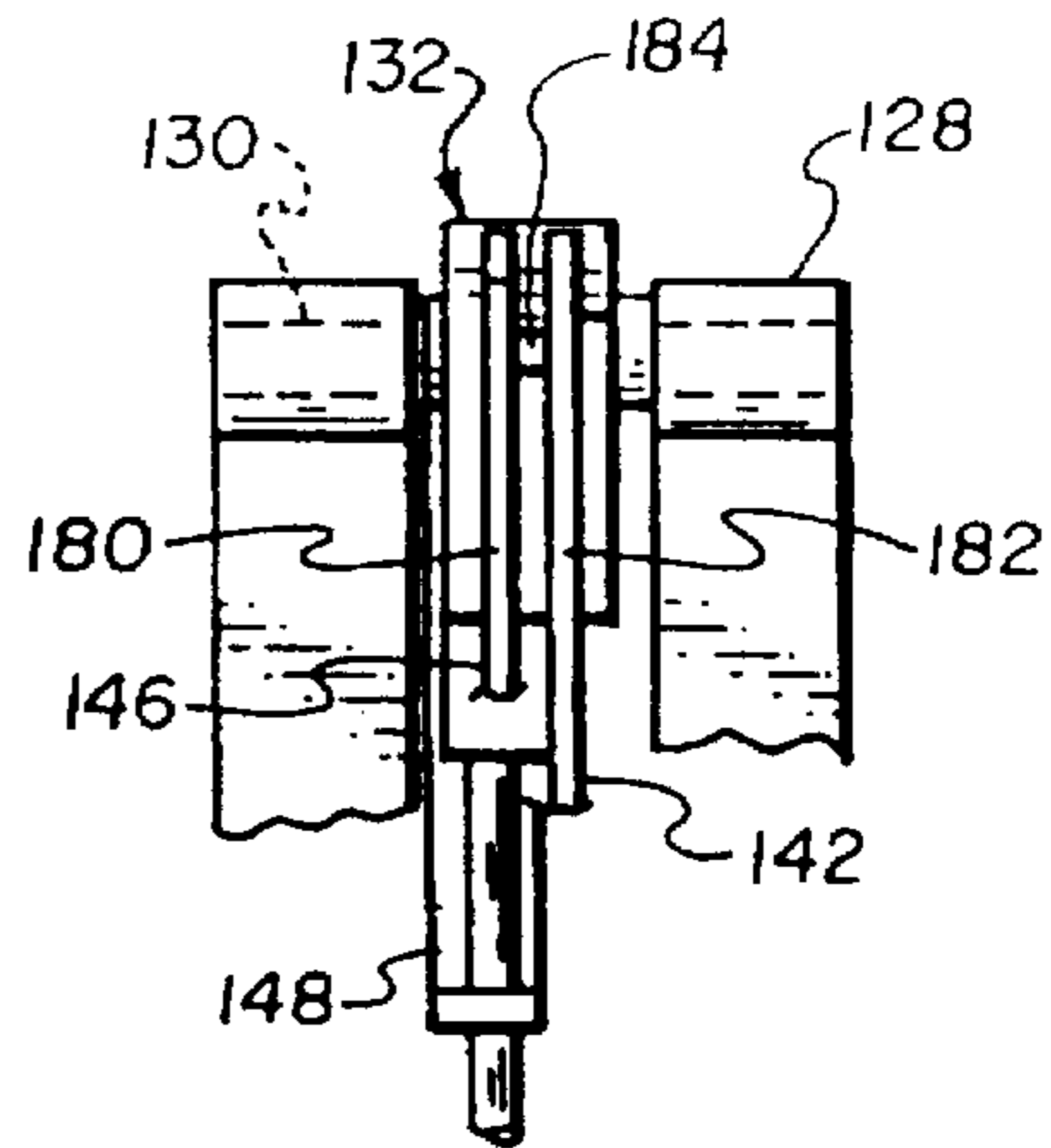
Fig. 5 (PRIOR ART)
