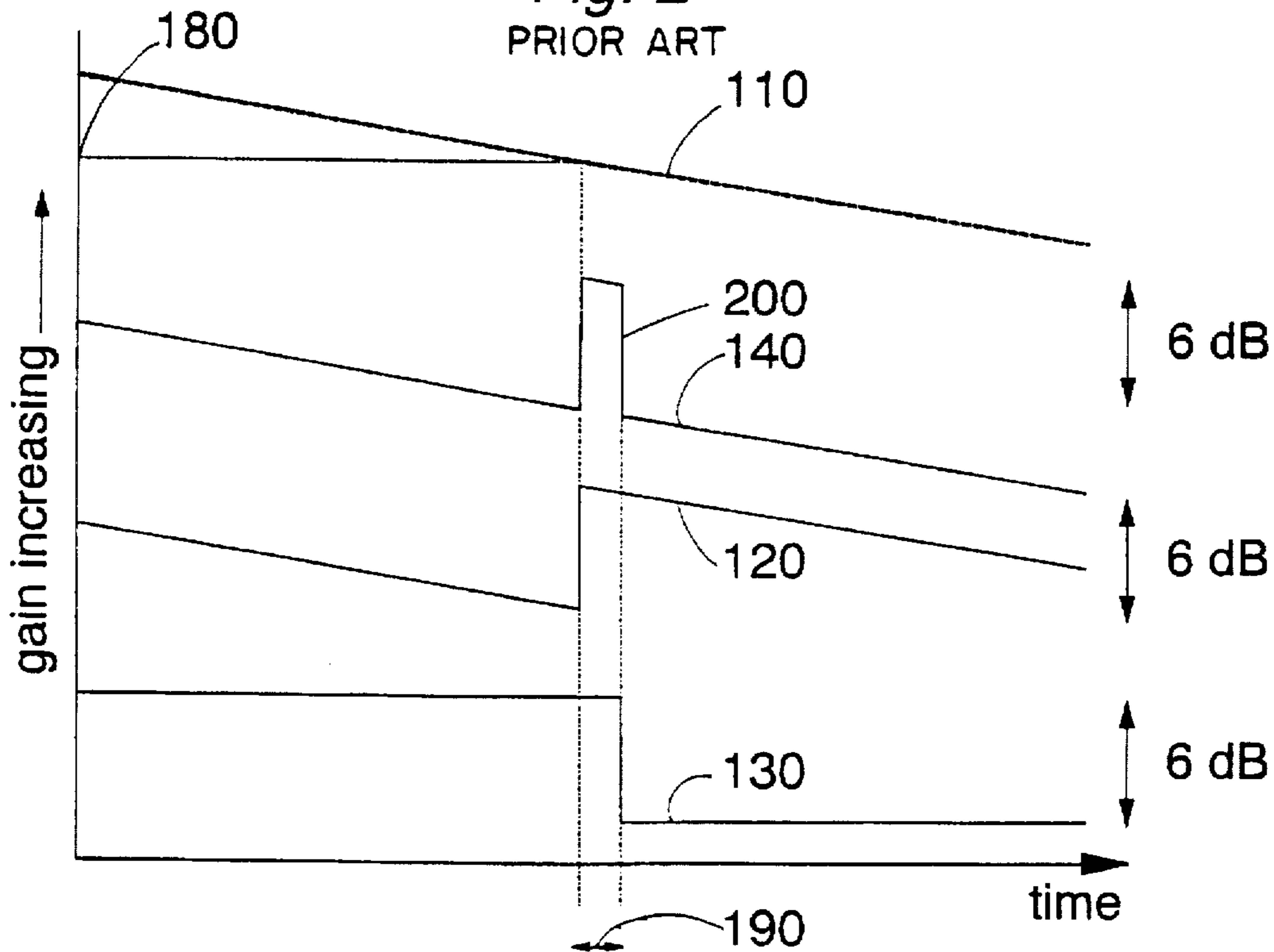
Fig. 3 PRIOR ART
