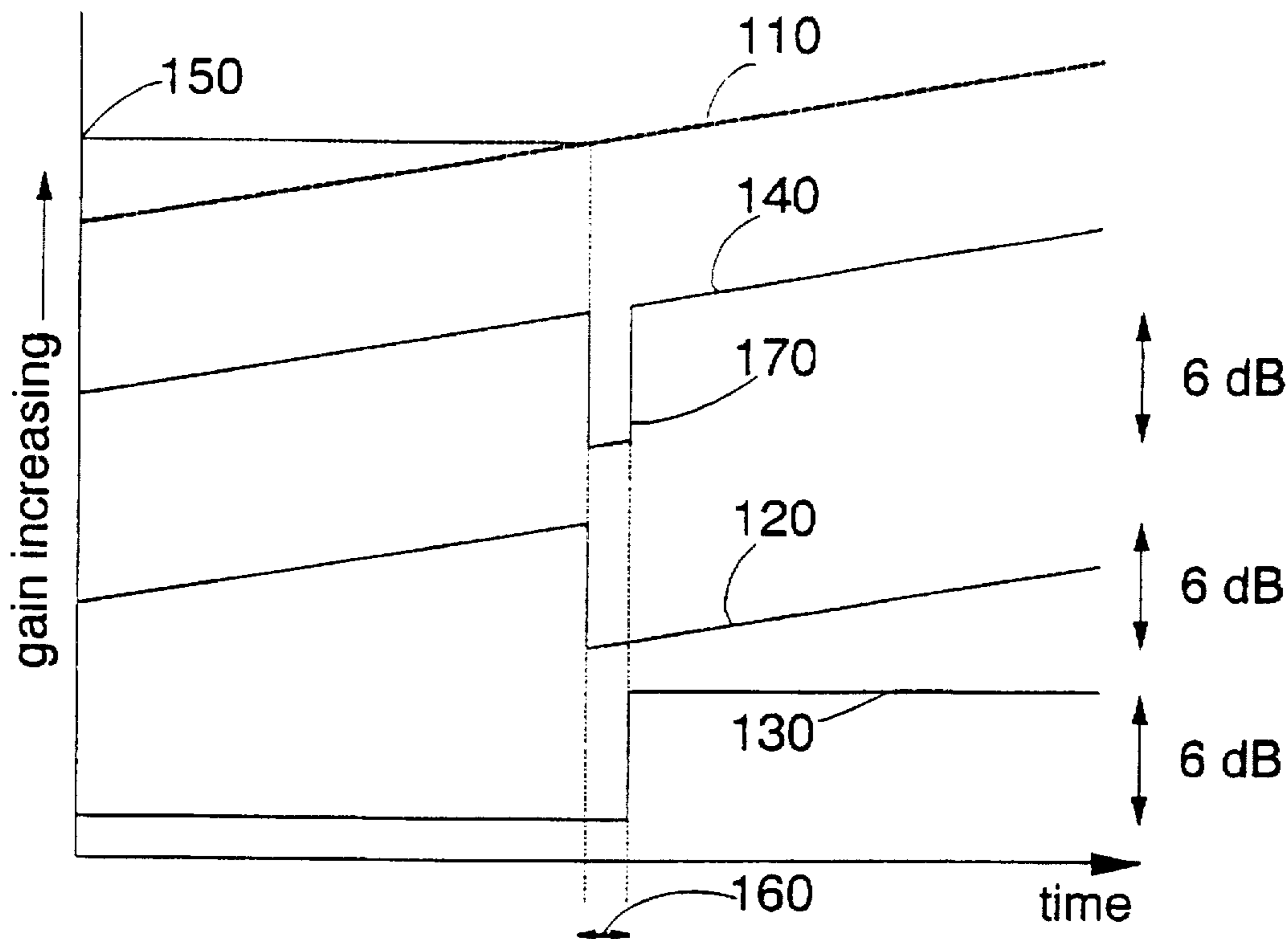
Fig. 2 PRIOR ART
