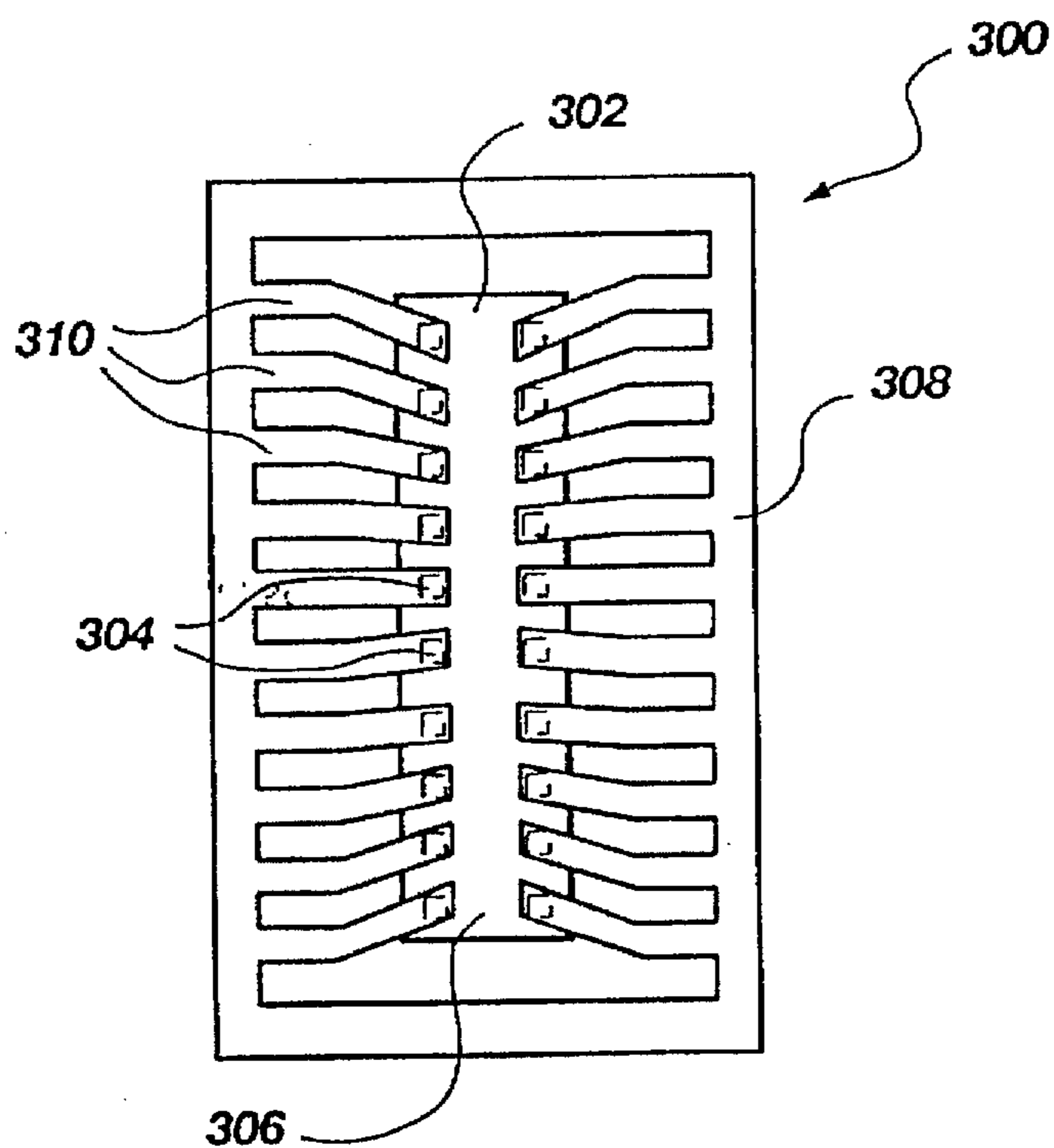
Fig. 3 PRIOR ART
