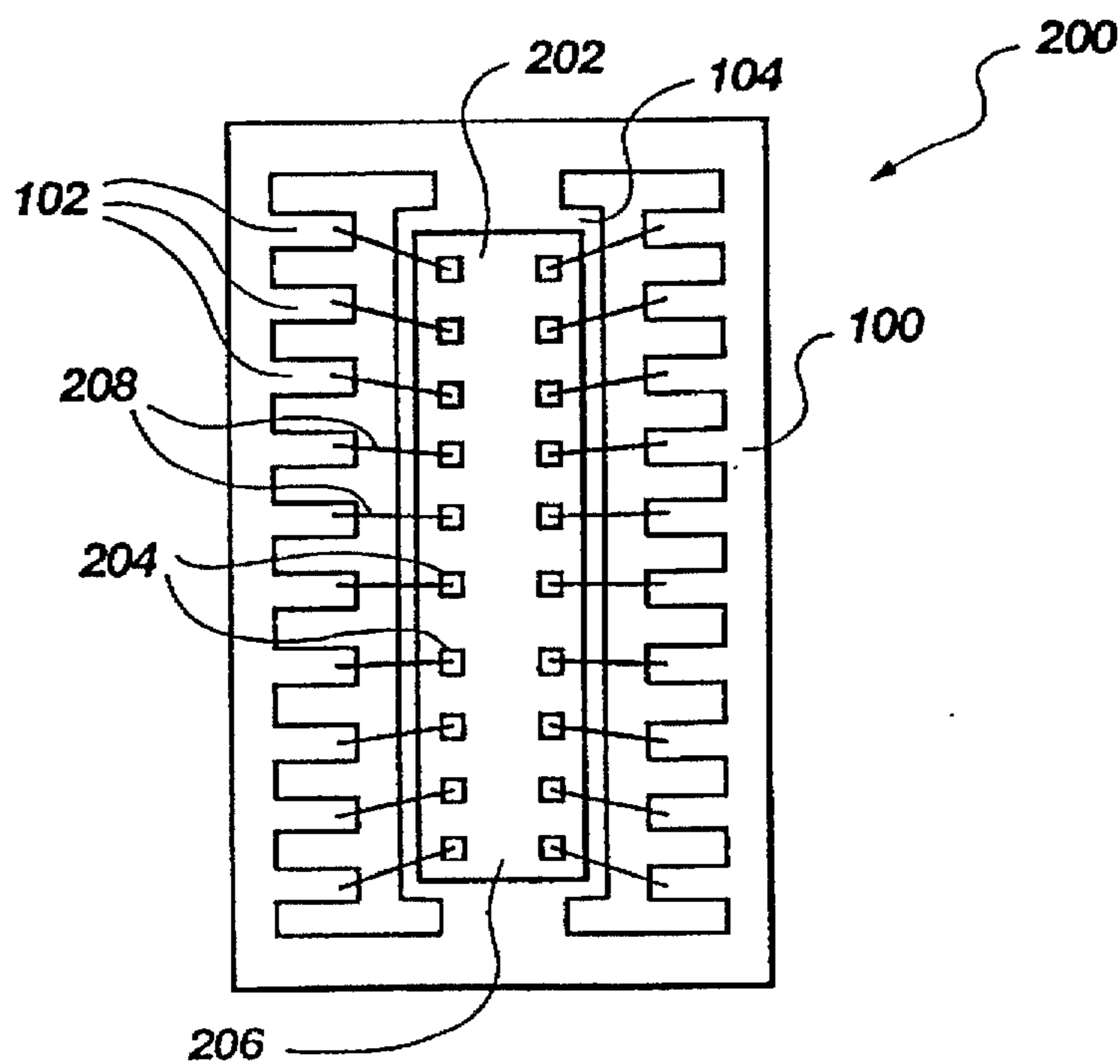
Fig. 2 PRIOR ART
