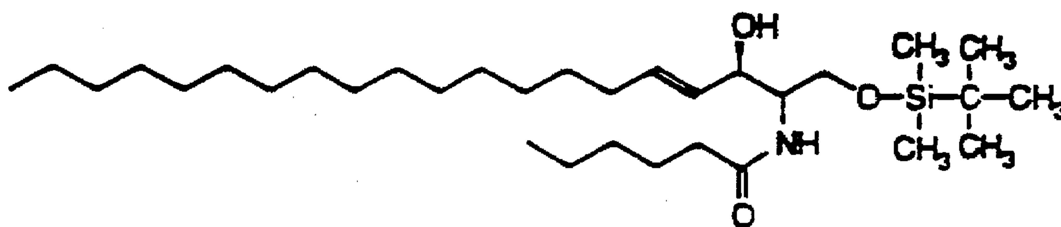
C6 Cer-1-TBDMS
