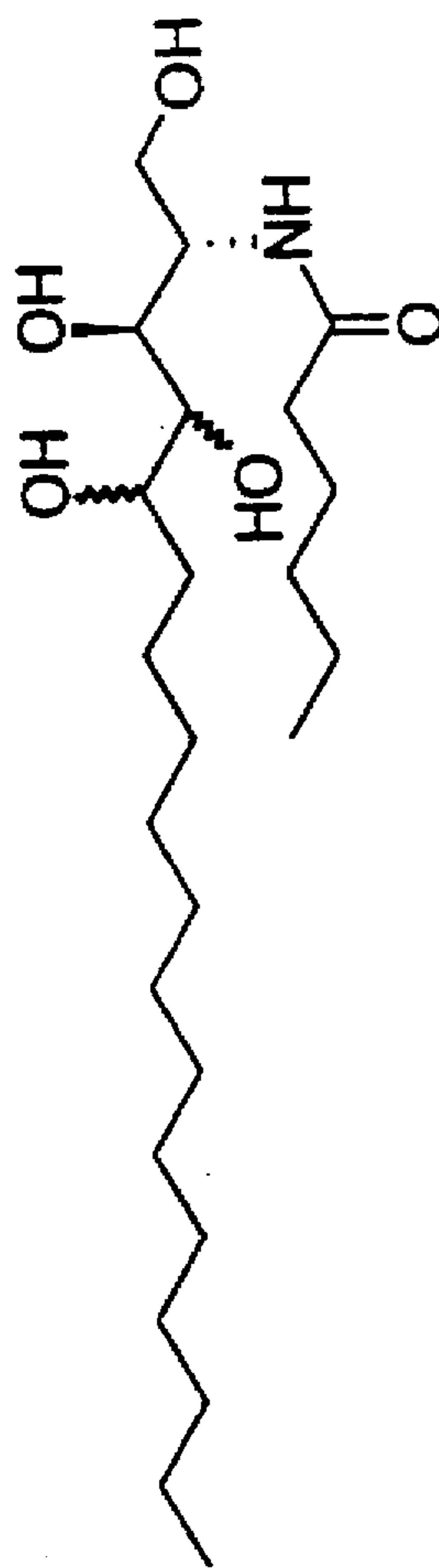
4,5-Diol C6-Cer
