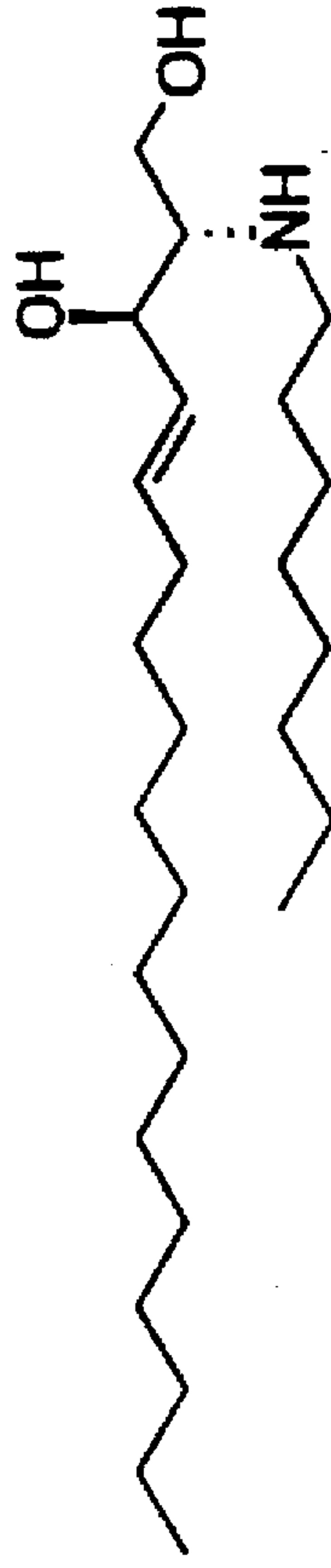
N-C8 Sphingosine
