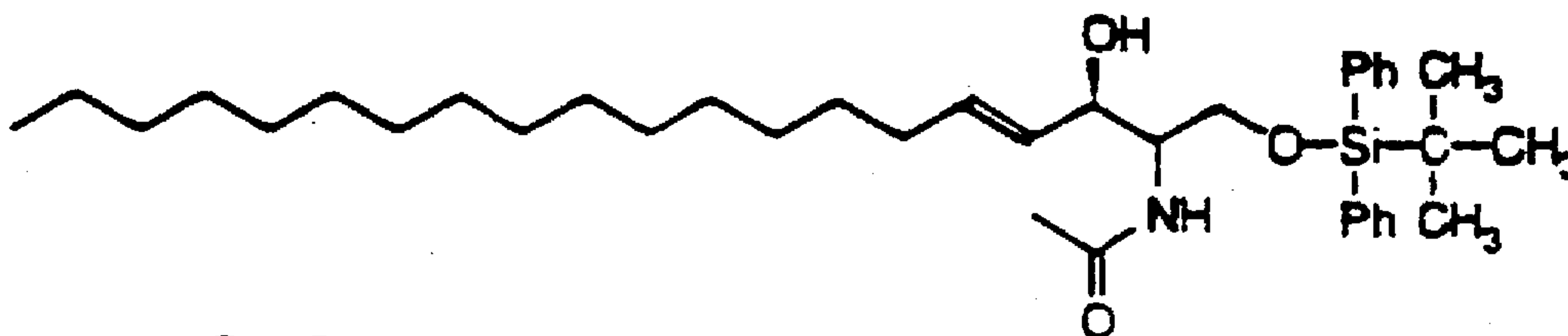
C2 Cer-1-TBDPS
