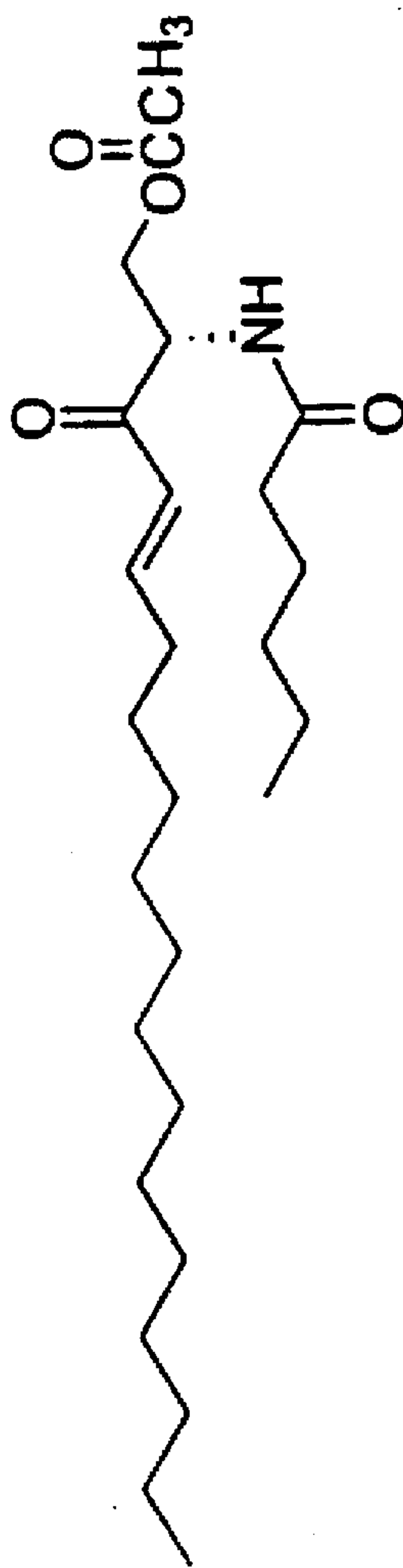
1-Acetate-3-one C6-Cer
