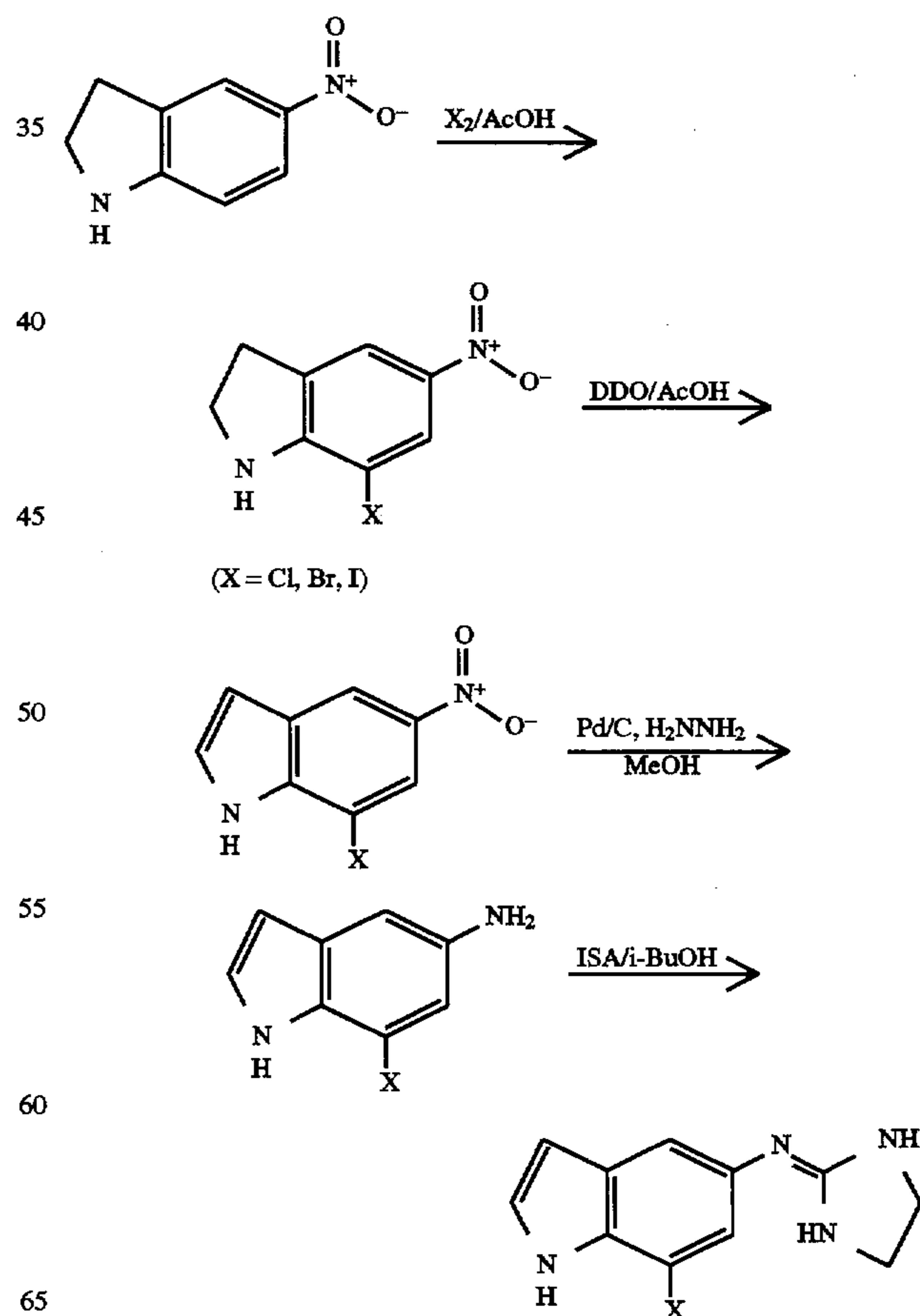
Scheme 1 illustrates schematically the synthesis of 7-substituted derivatives of 5-(2-imidazolin-2ylamino) indole.
