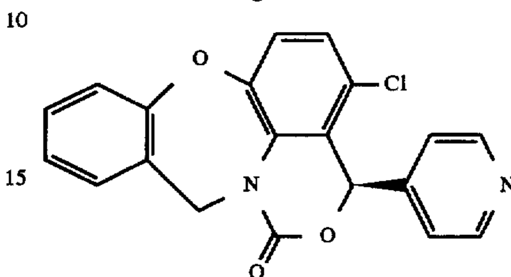
Compound 6
