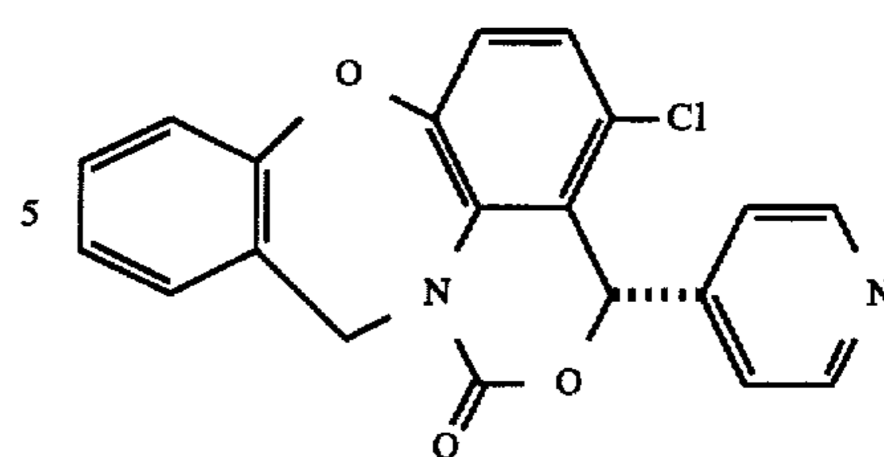
Compound 5
