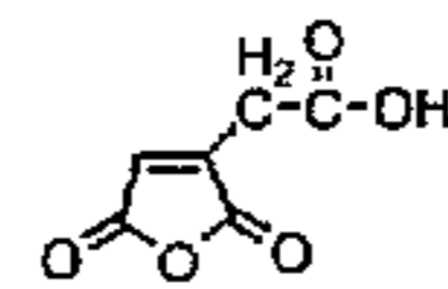
cis-aconitic anhydride
