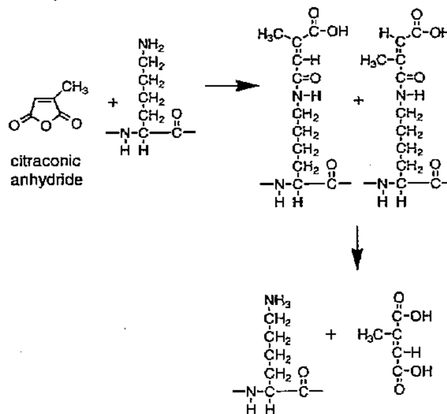
A scheme for the reversible reaction of citraconic anhydride with lysine residues
