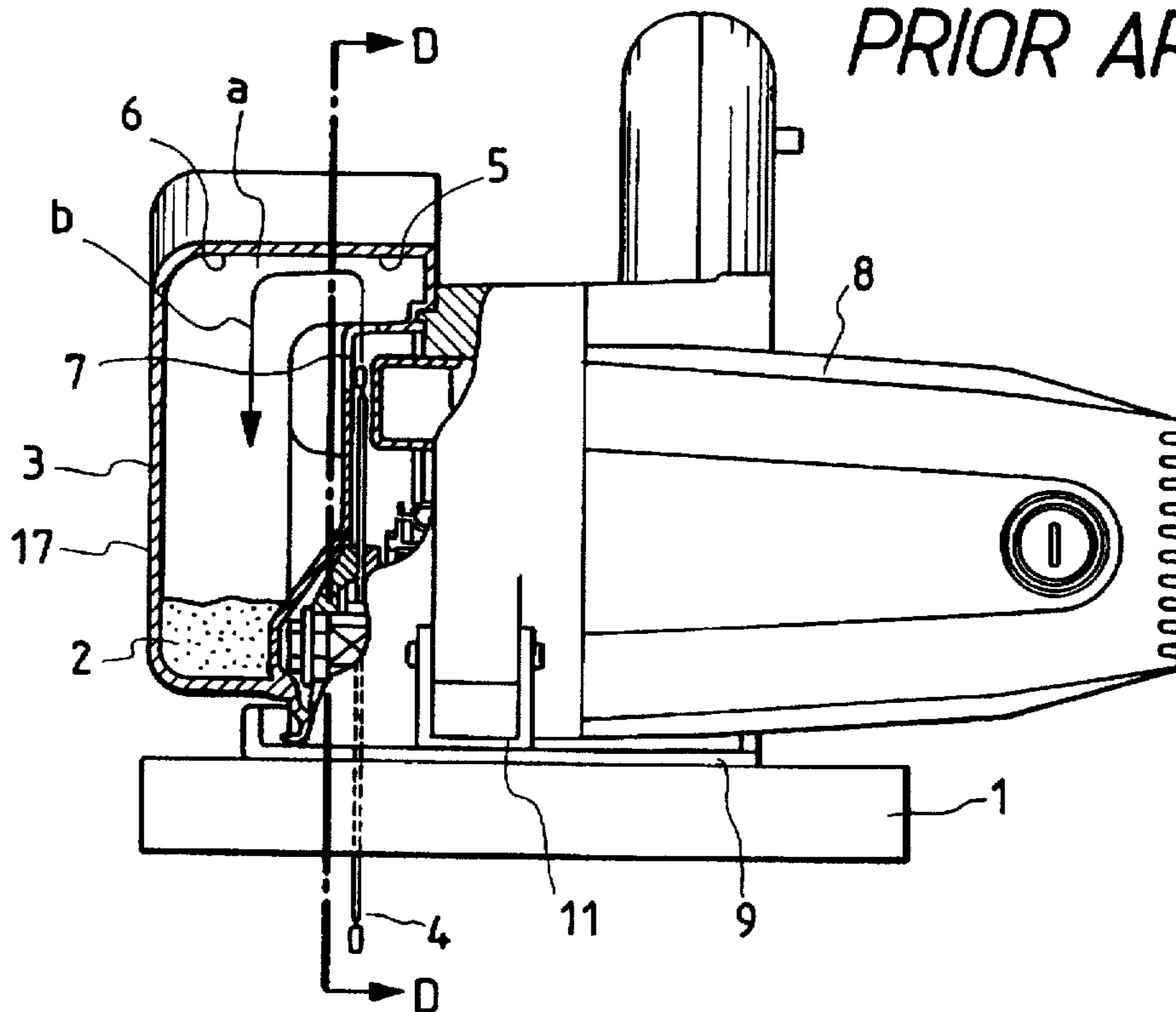
FIG. 8 PRIOR ART
