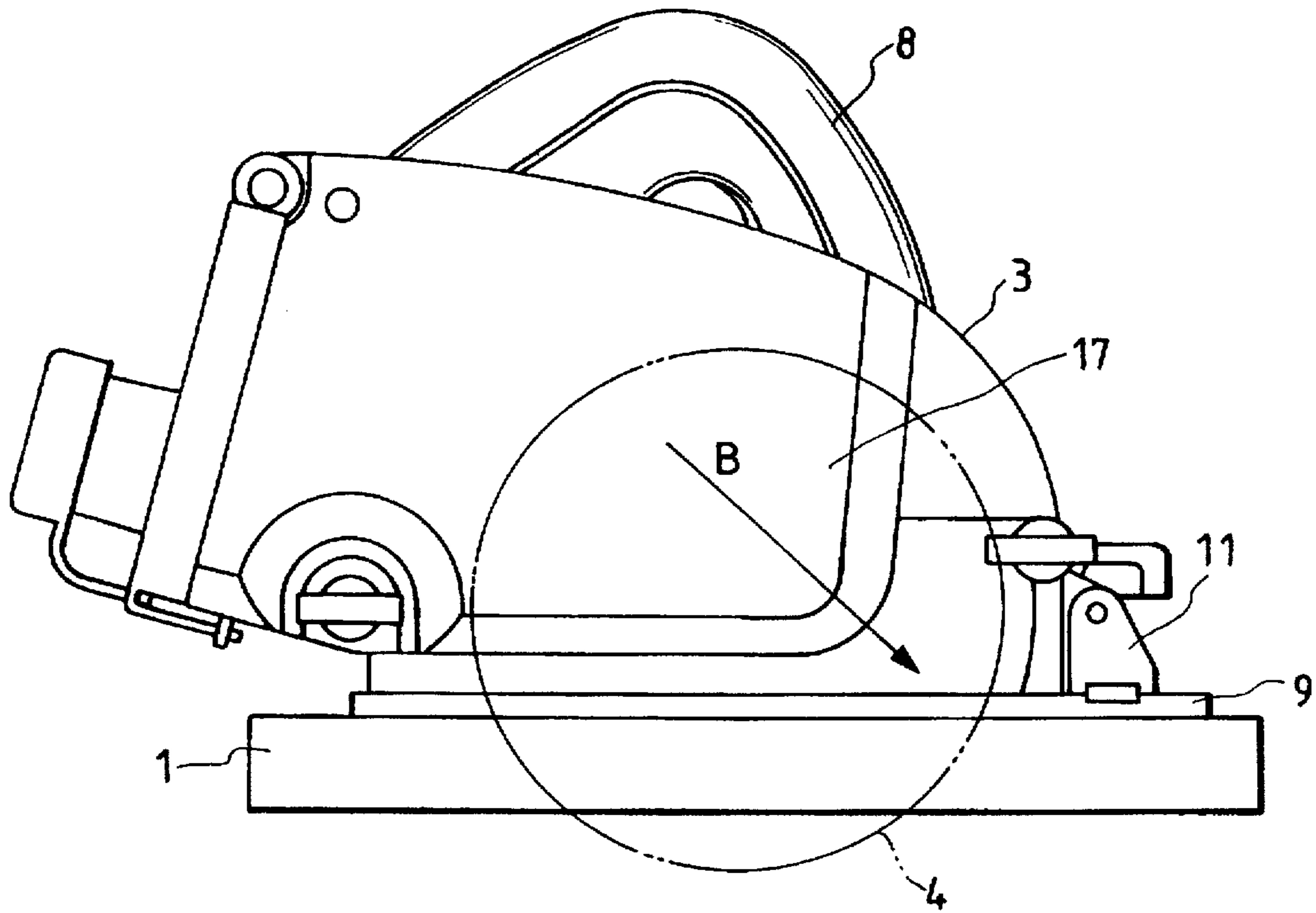
FIG. 6 PRIOR ART
