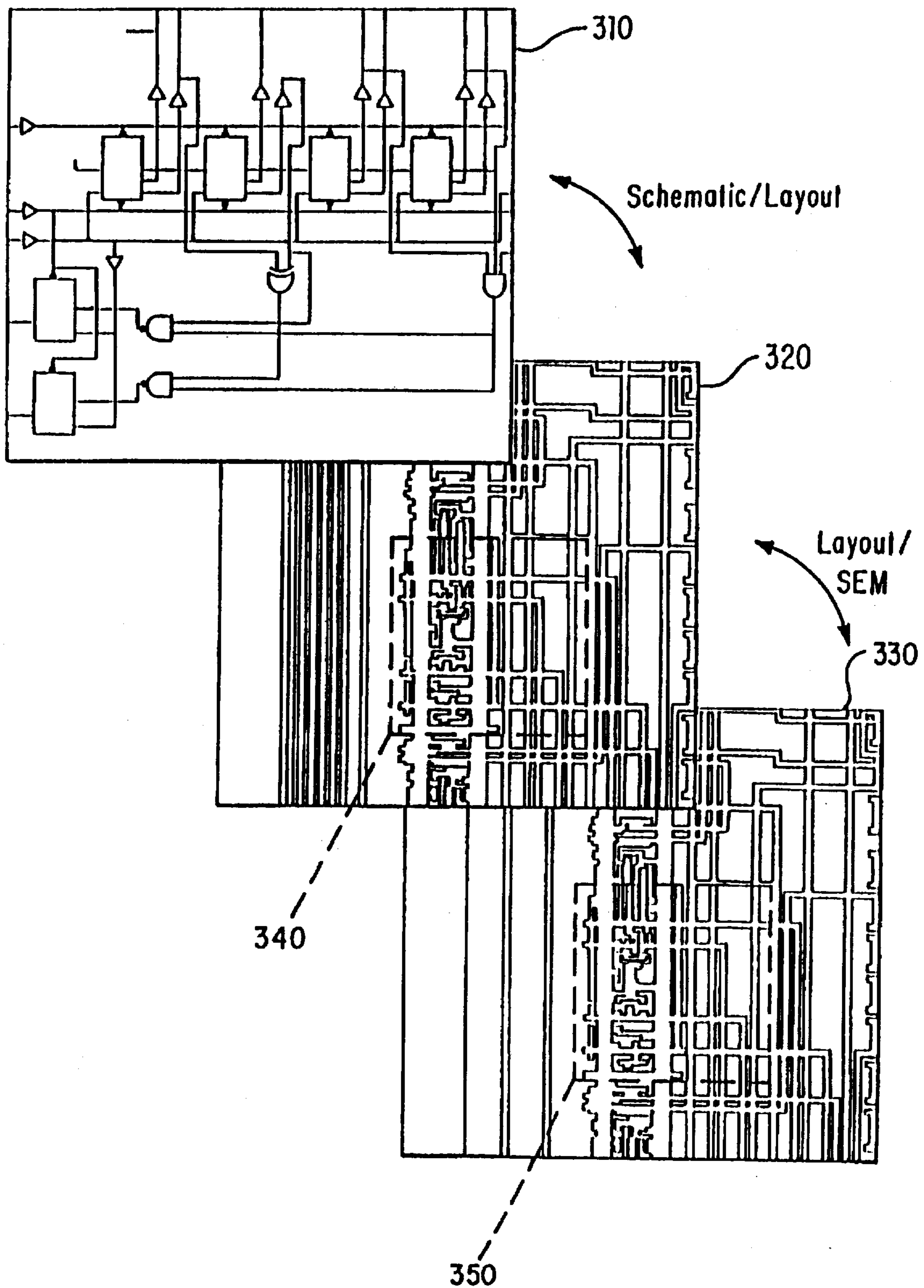
FIG. 3 PRIOR ART
