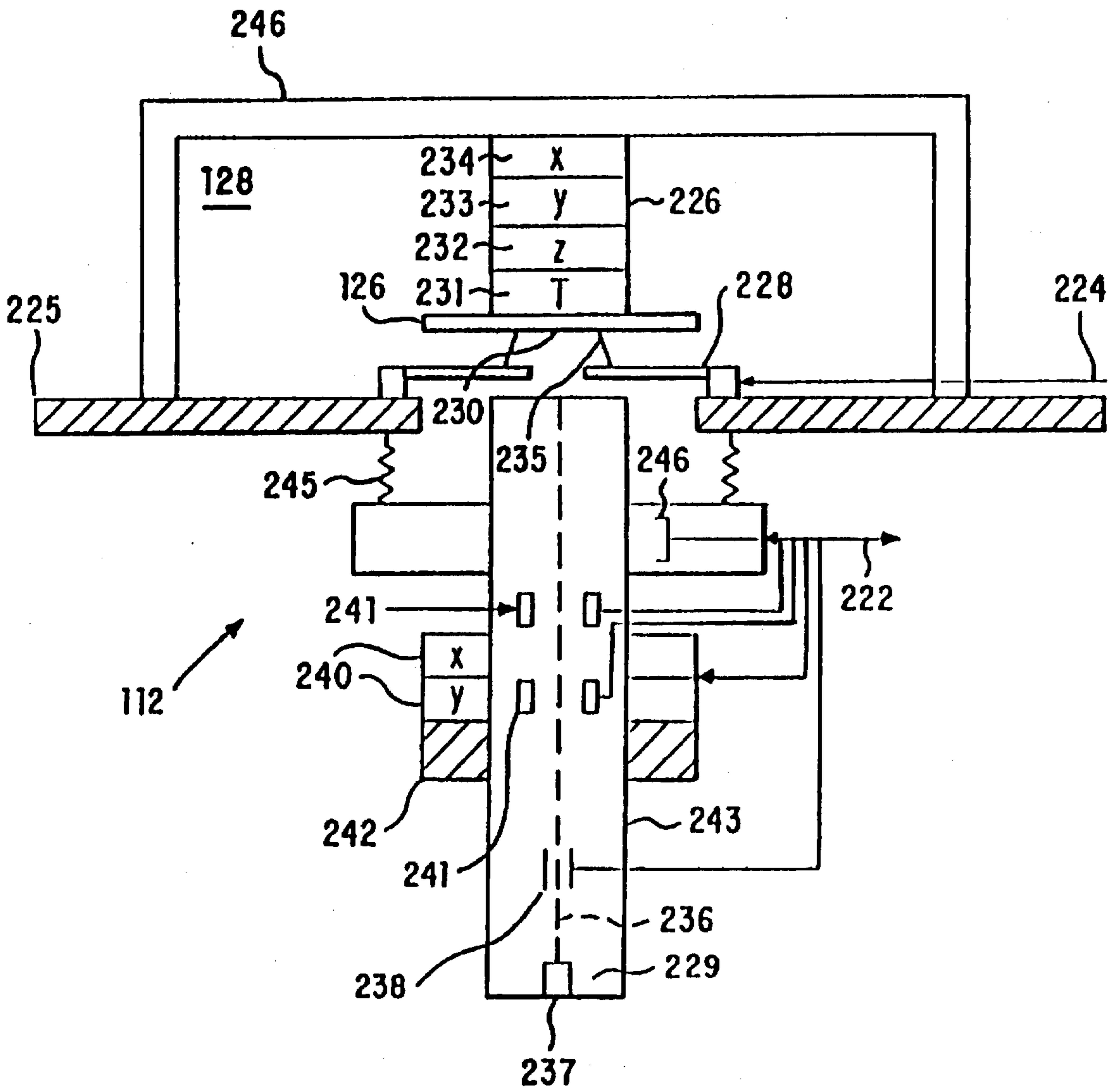
FIG. 2 PRIOR ART
