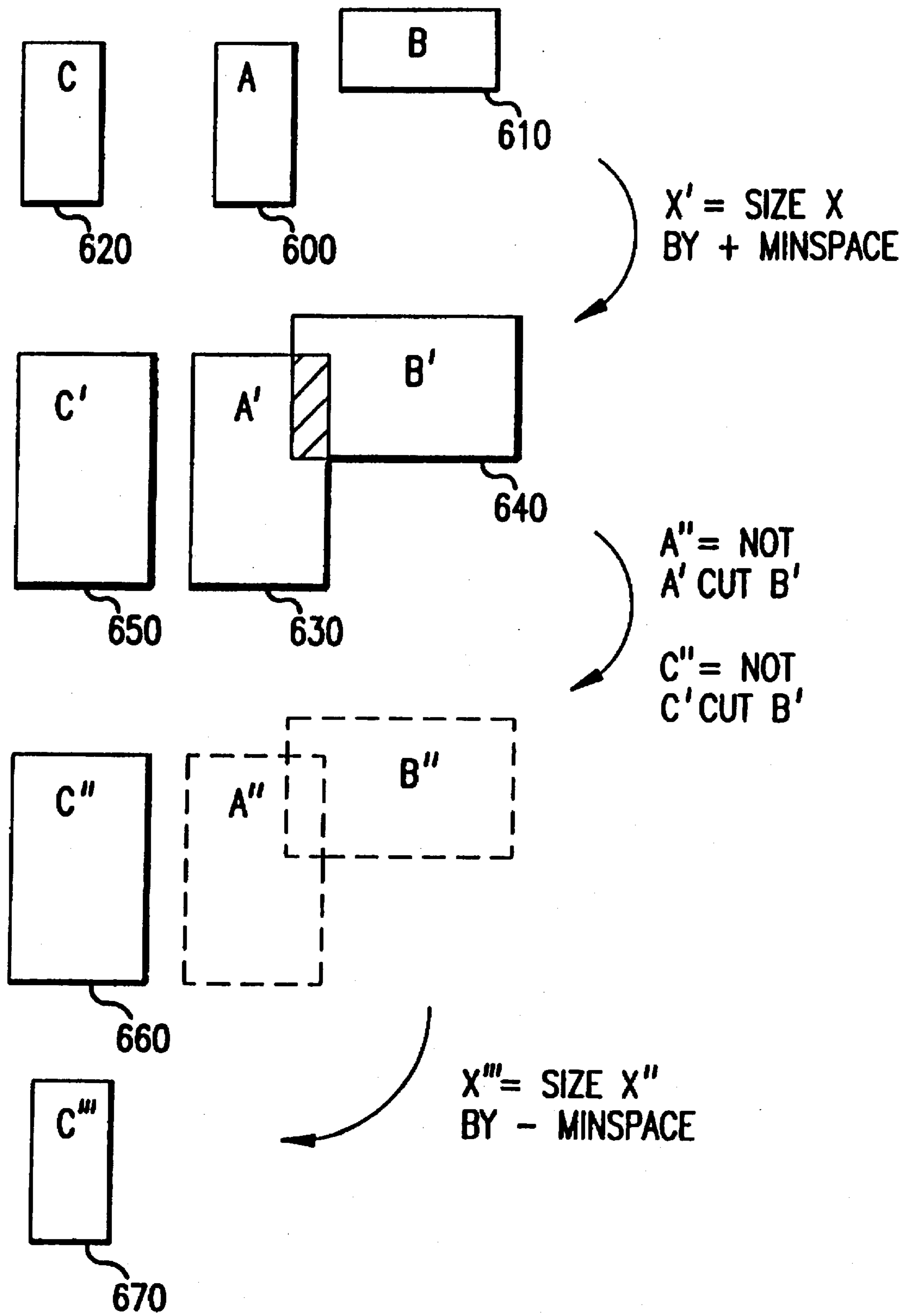
FIG.6 PRIOR ART
