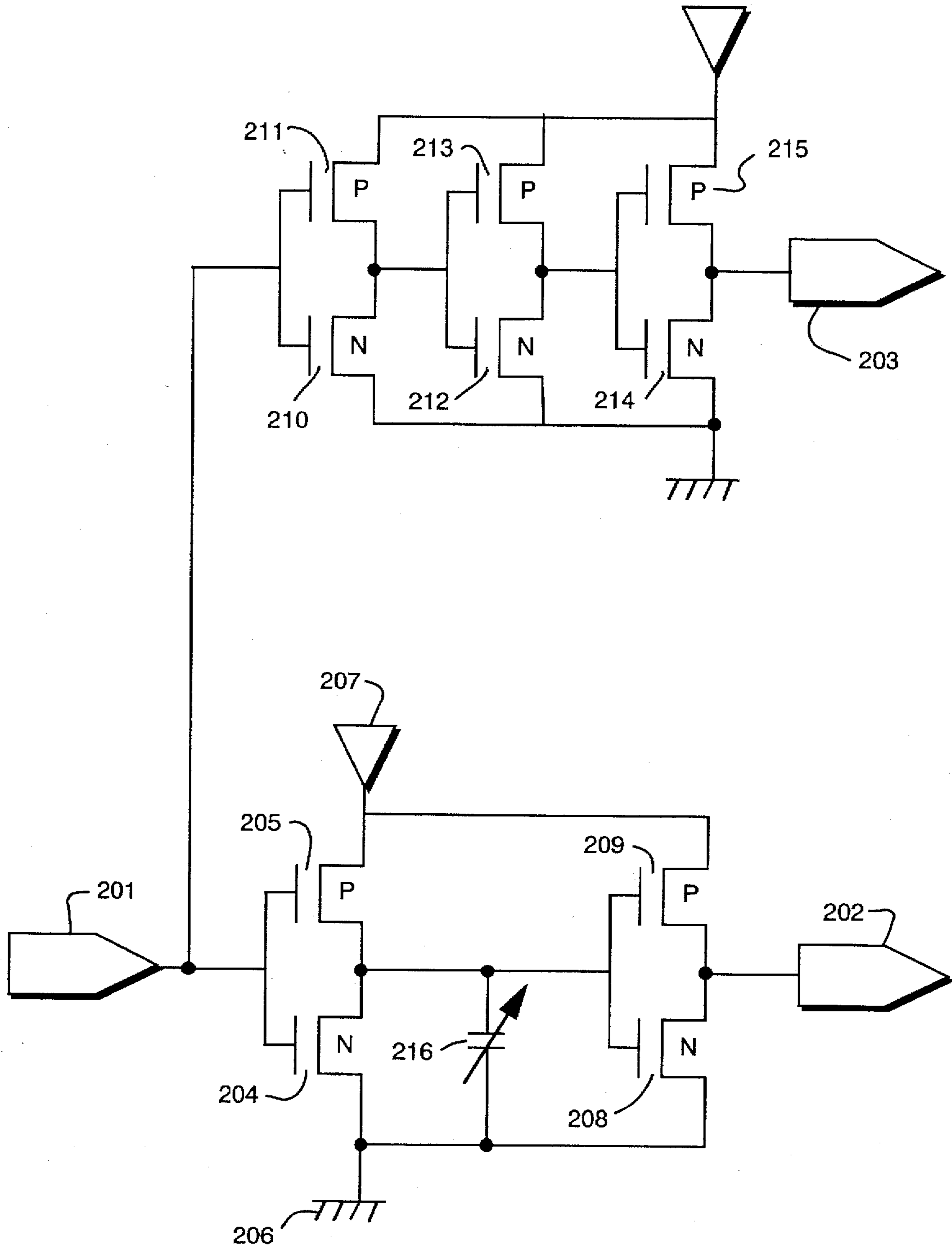
FIG. 2 (PRIOR ART)
