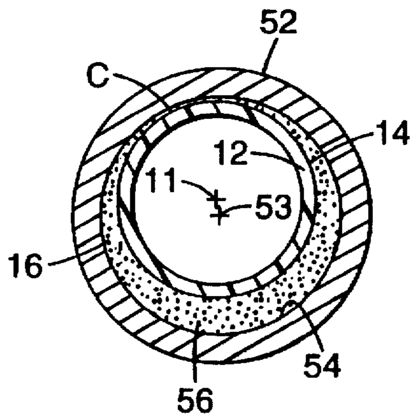
Fig. 3 PRIOR ART
