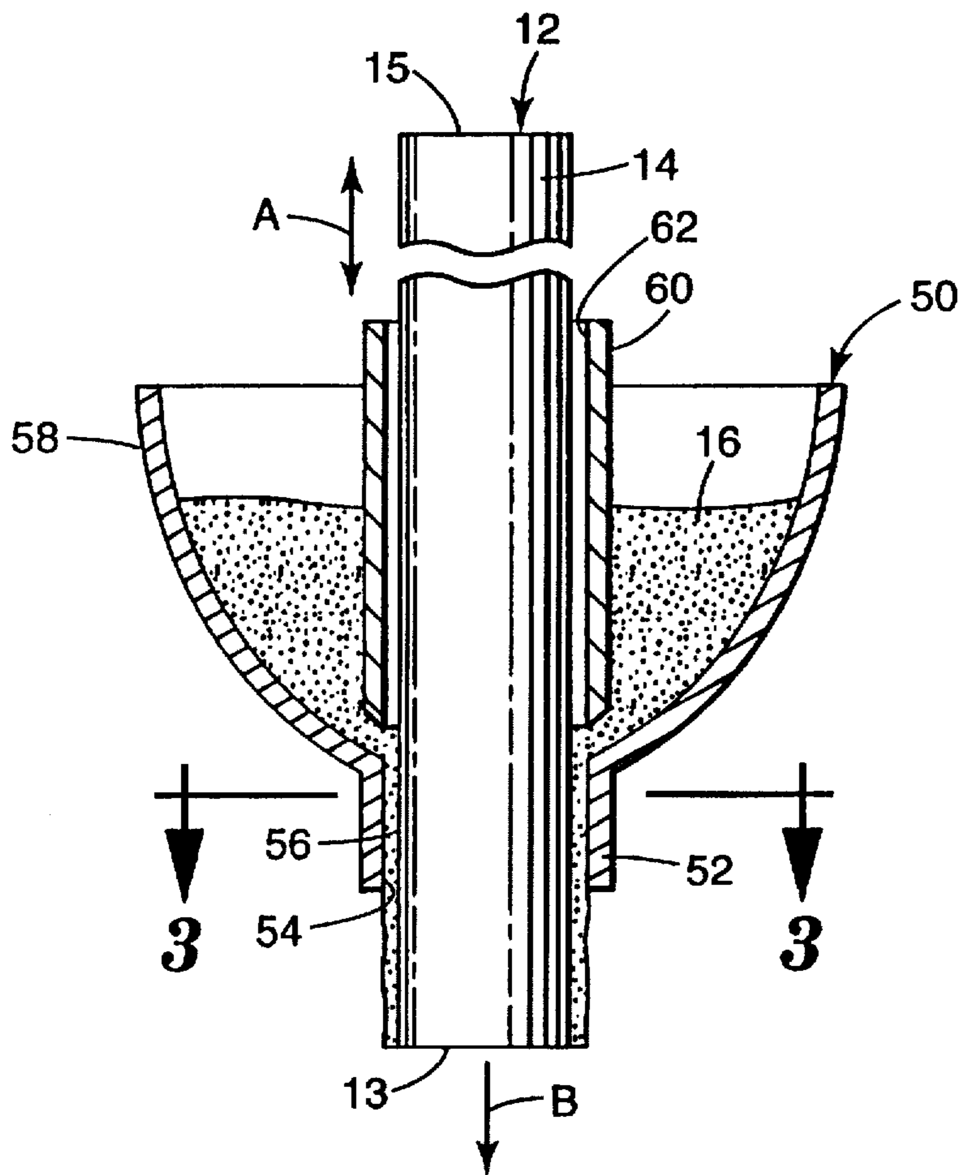
Fig. 2 PRIOR ART
