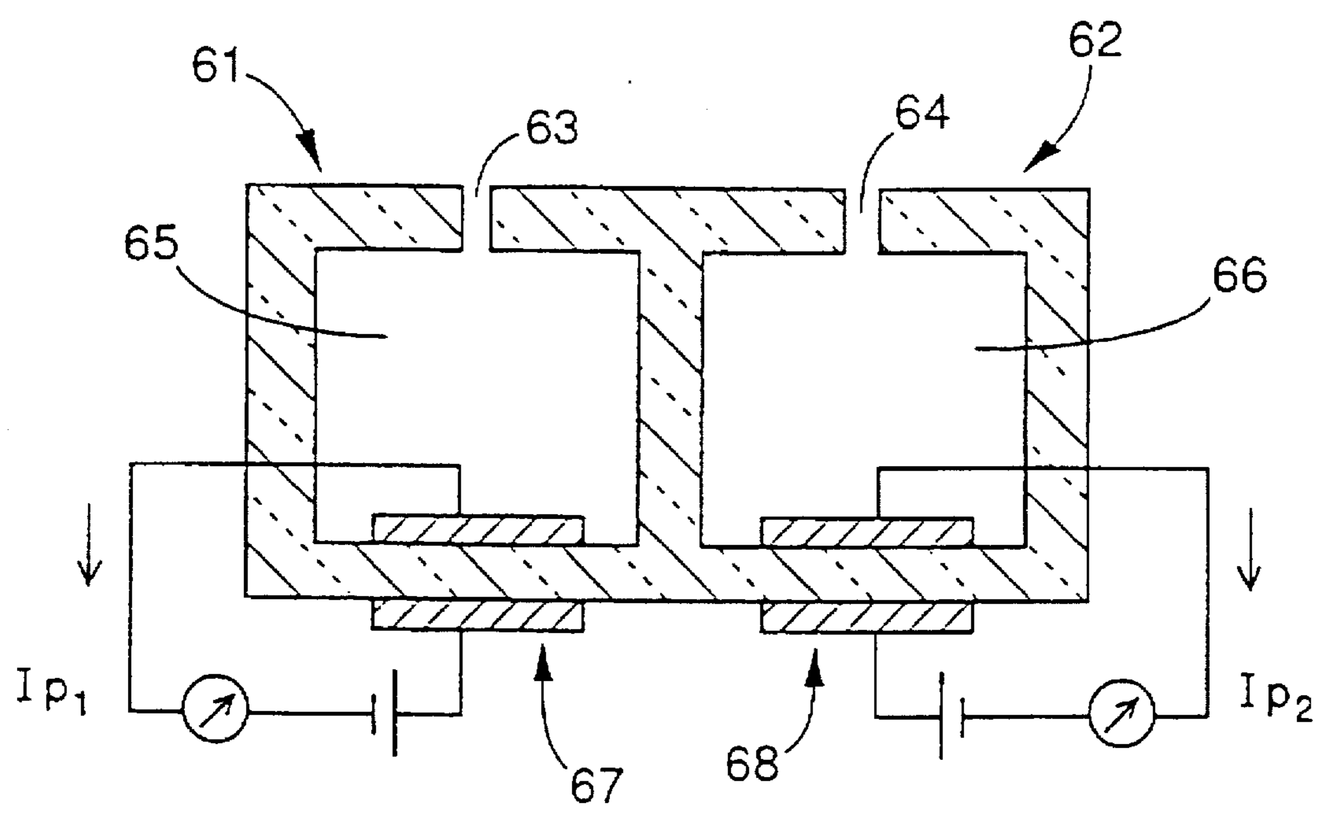
FIG. 25 PRIOR ART
