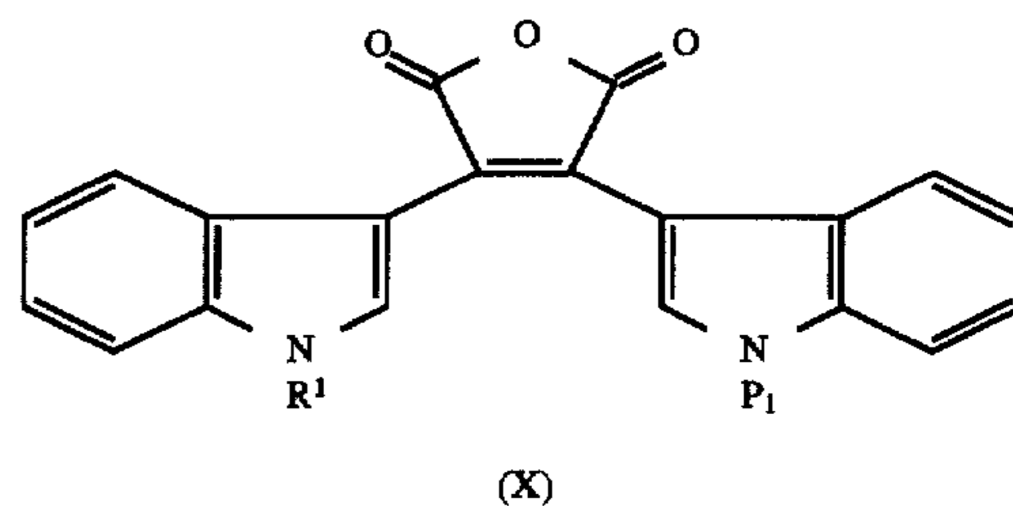
-continued Scheme 1
