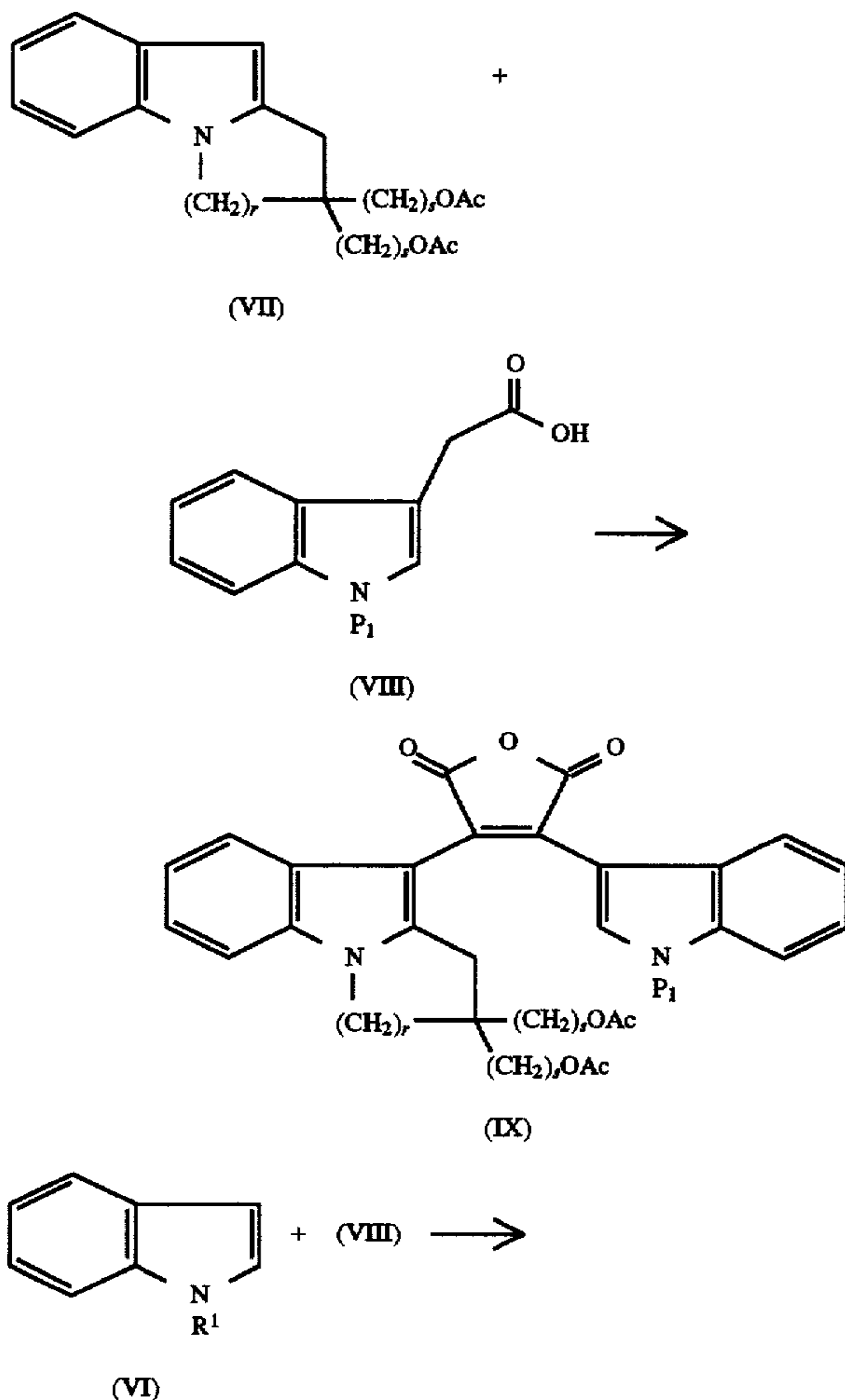
Scheme 1
