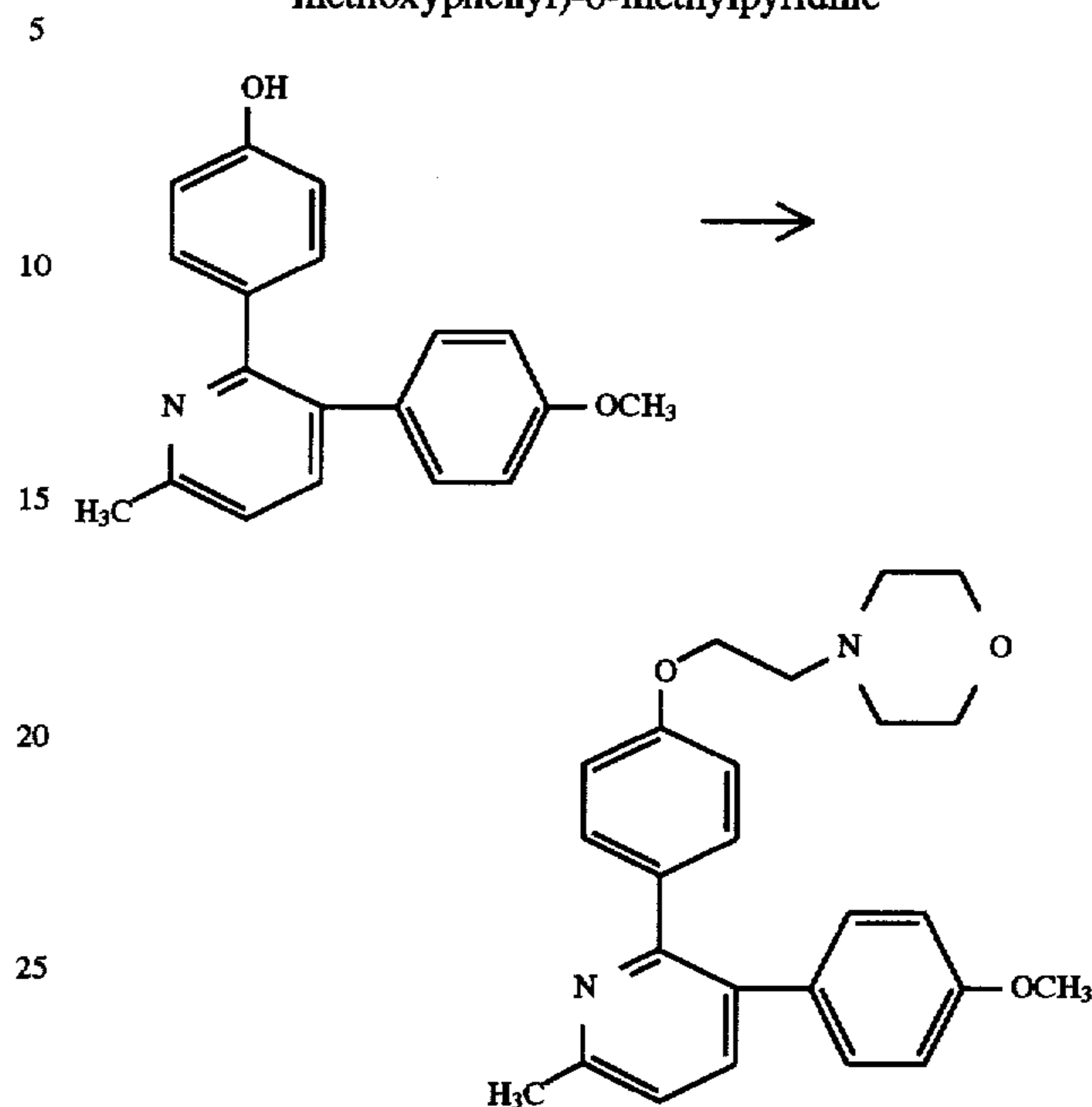
2-[4-[2-(4-Morpholinyl)ethoxy]phenyl]-3-(4-methoxyphenyl)-6-methylpyridine
