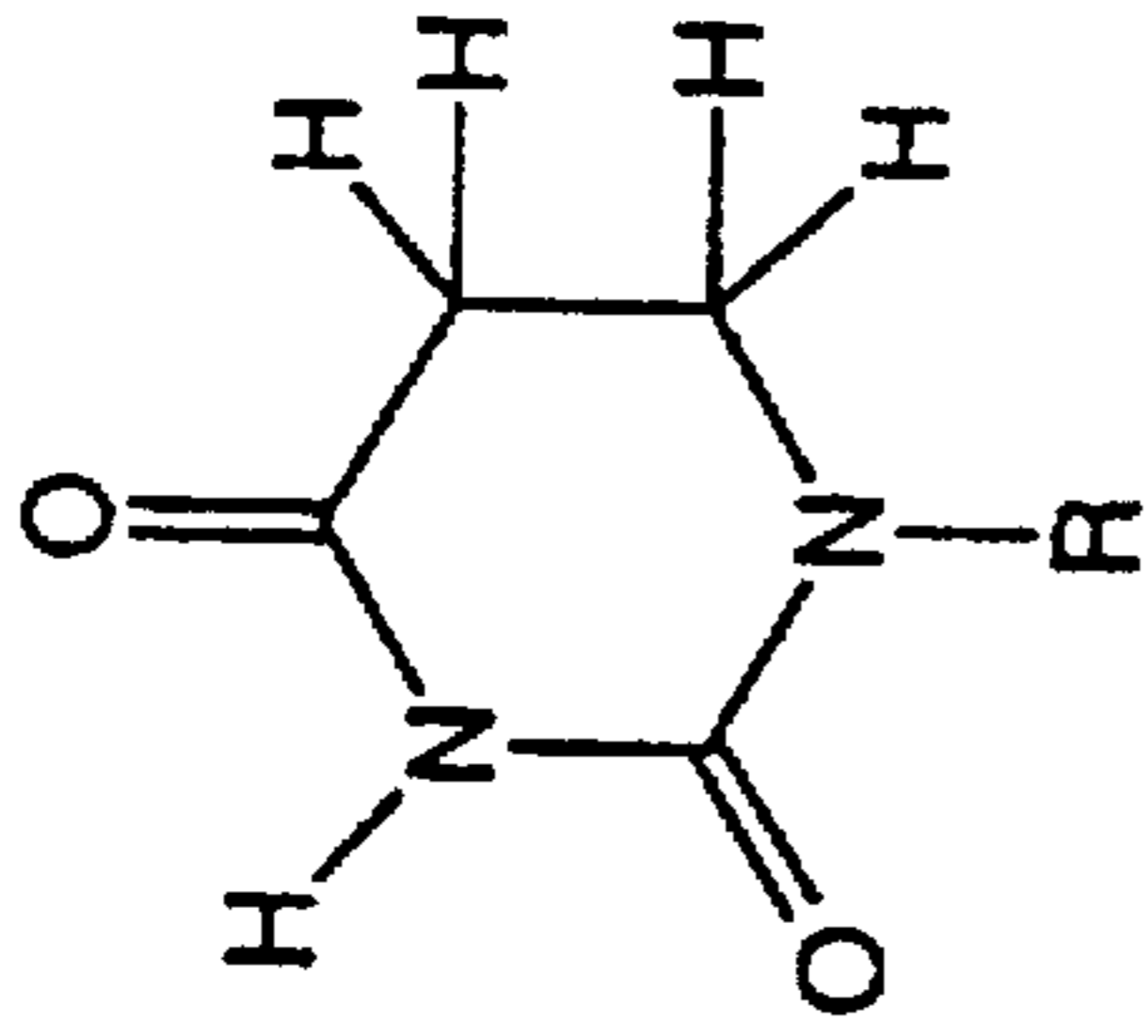
5,6-Dihydro-Uracil
