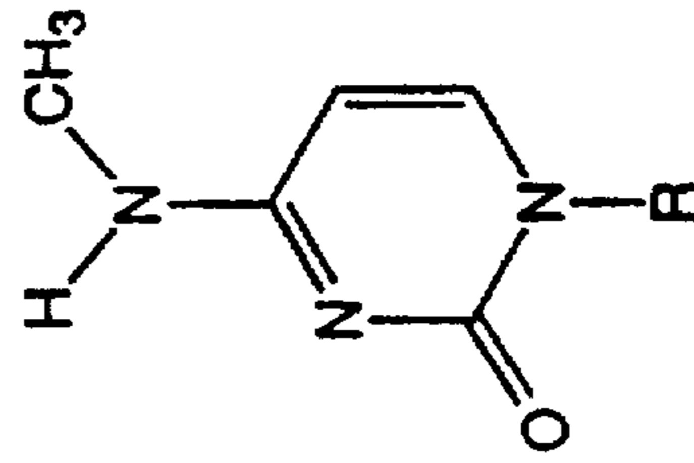
N 4 -Methyl-Cytosine
