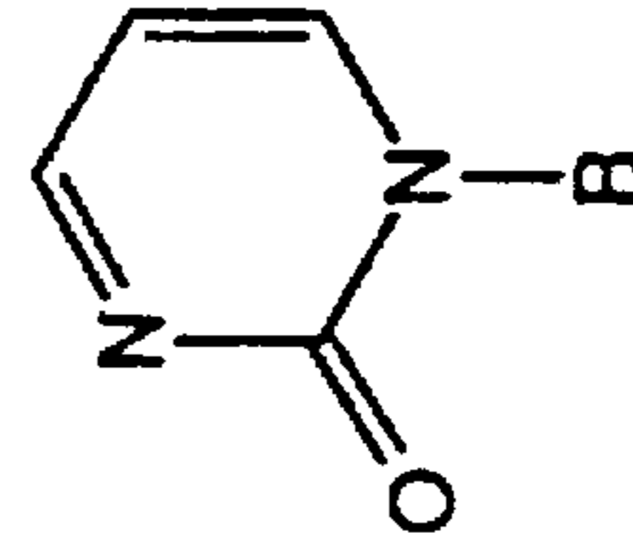
2-Pyridone
