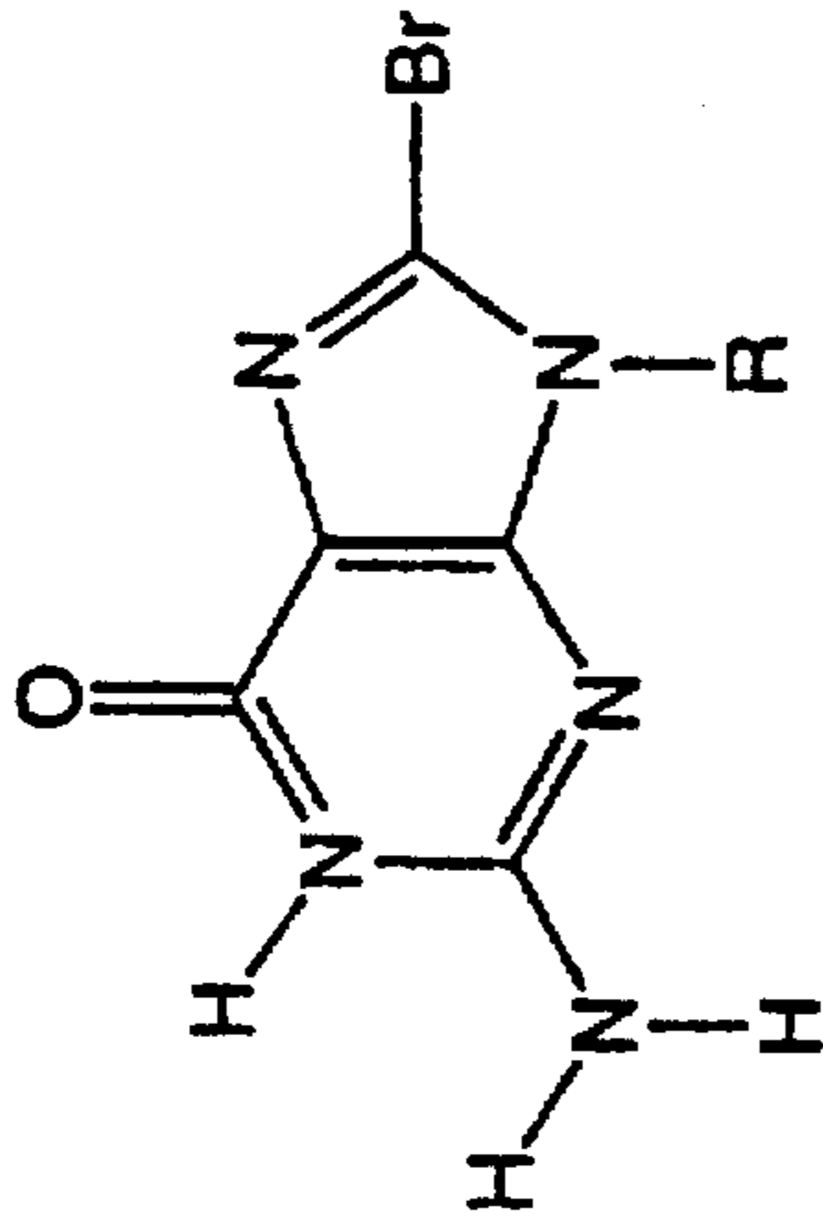
8-Bromo-Guanine
