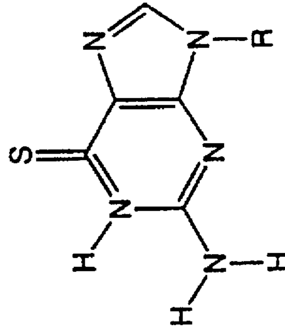
6-Thio-Guanine
