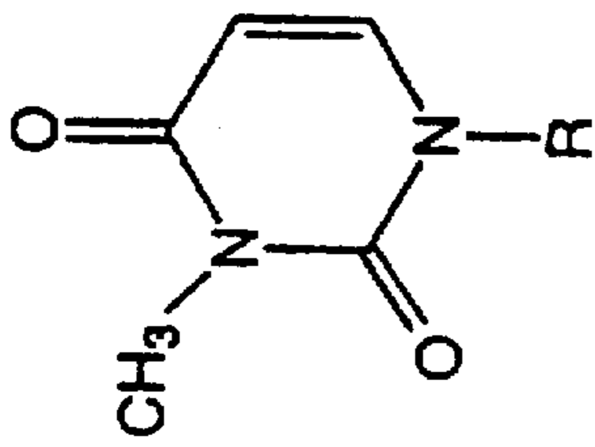
3-Methyl-Uracil
