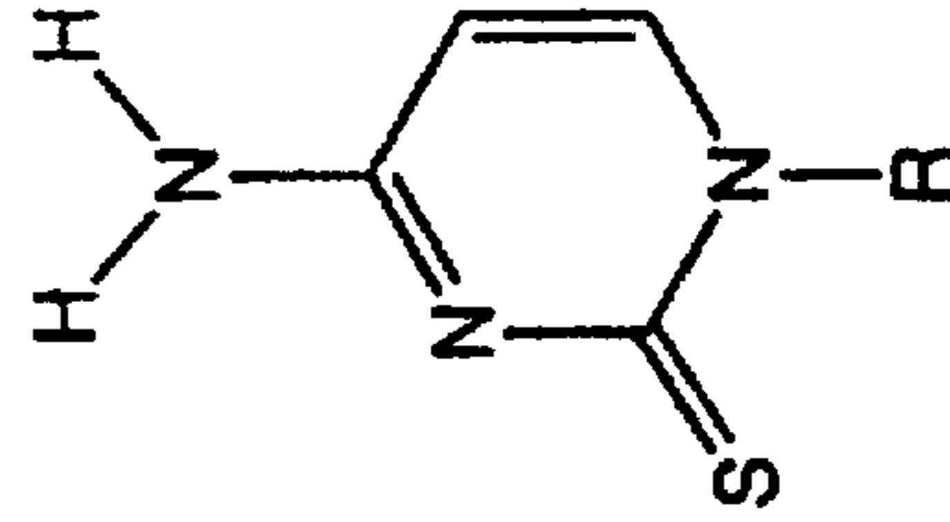
2-Thio-Cytosine
