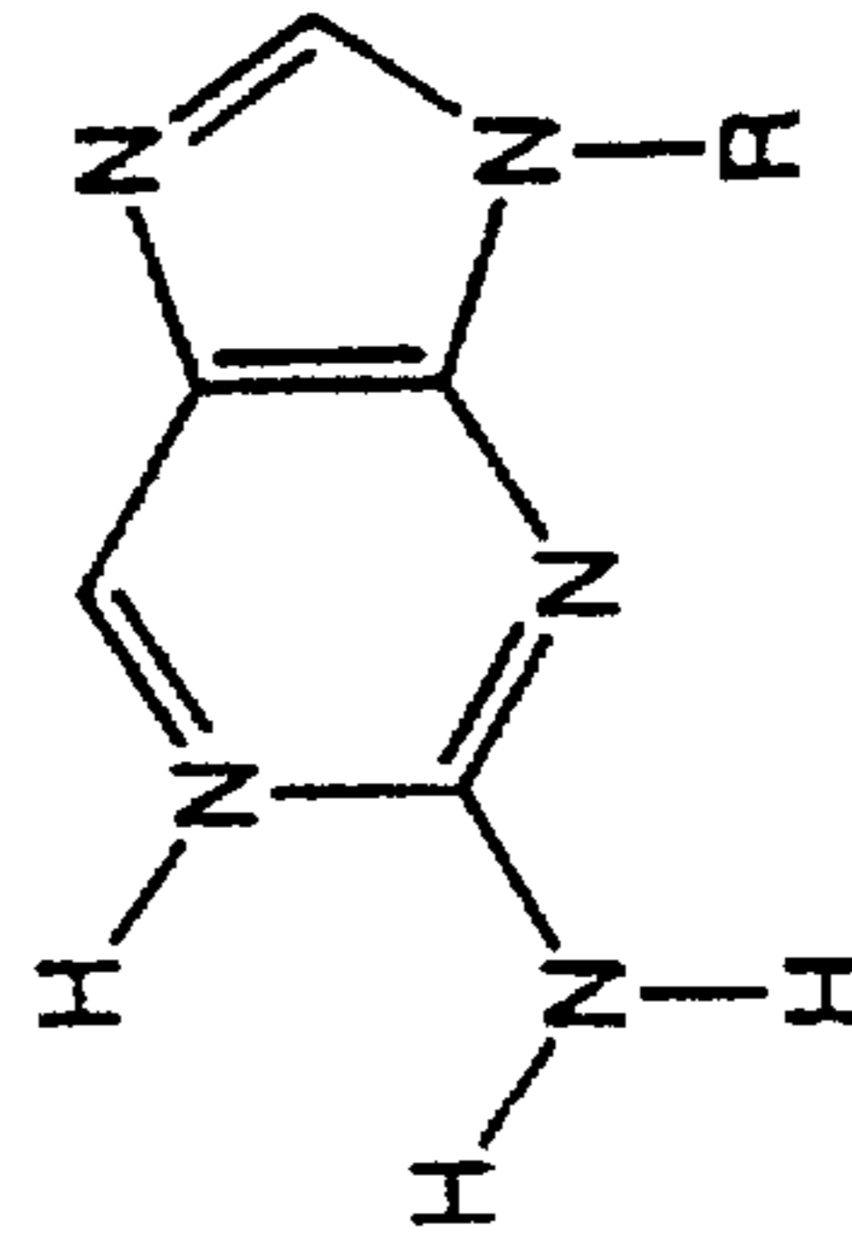
2-Amino-Purine
