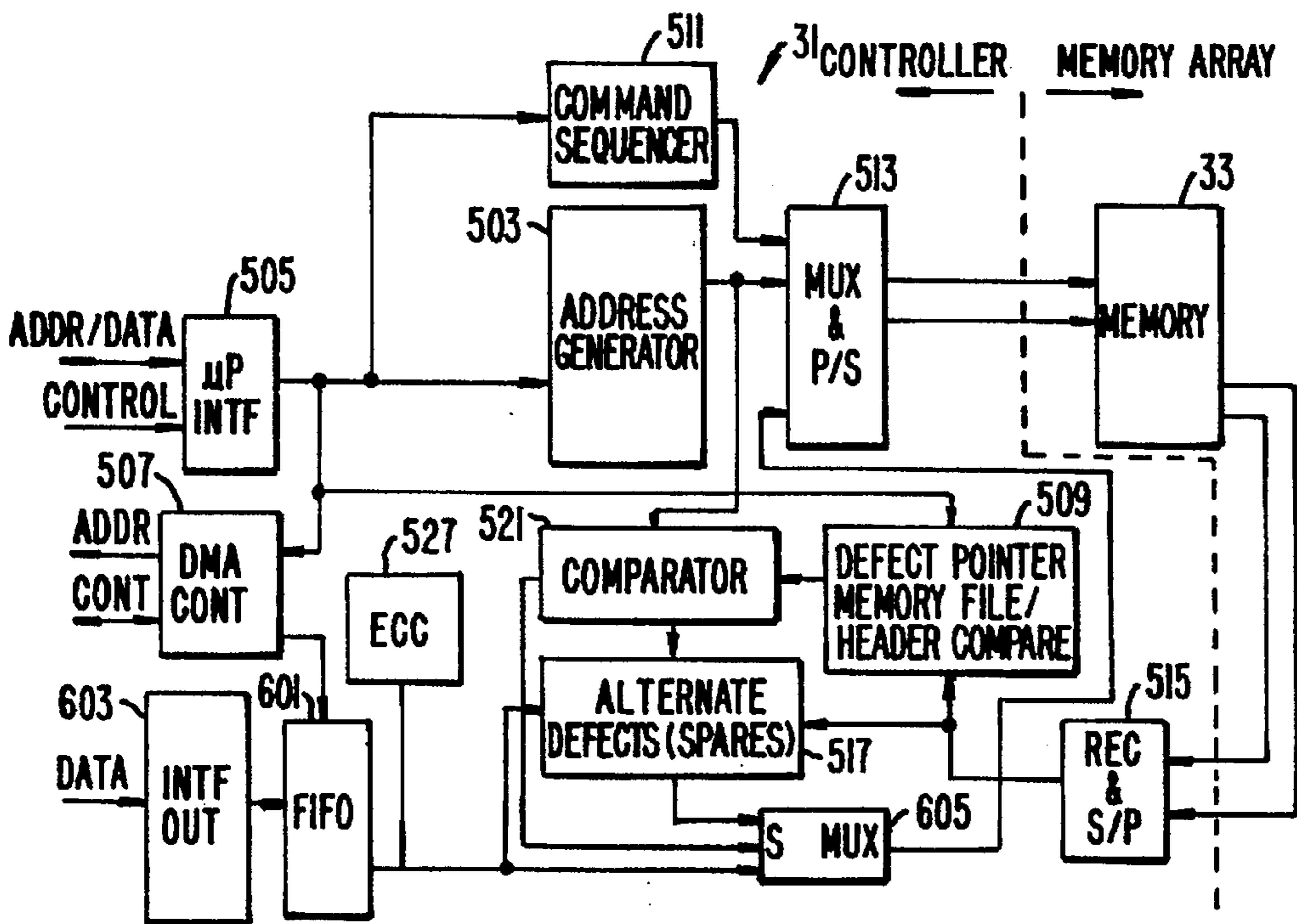
WRITE DATA PATH CONTROL FIG. 7.
