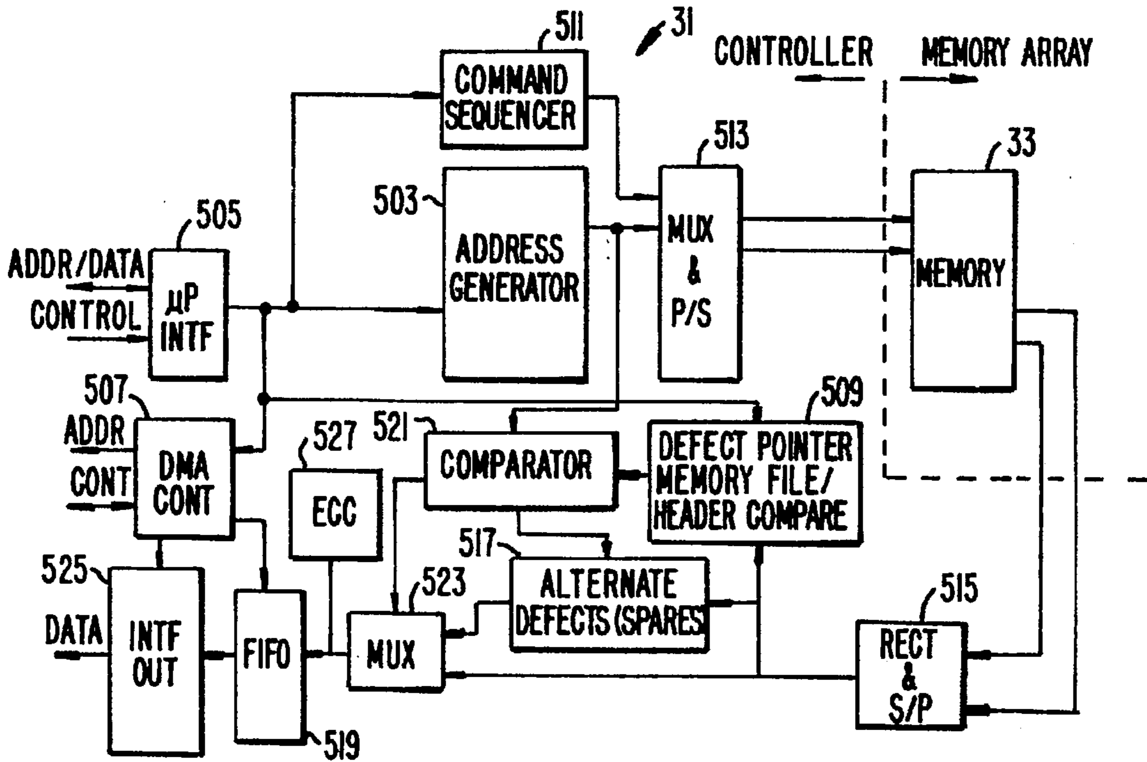
READ DATA PATH CONTROL FIG. 6.
