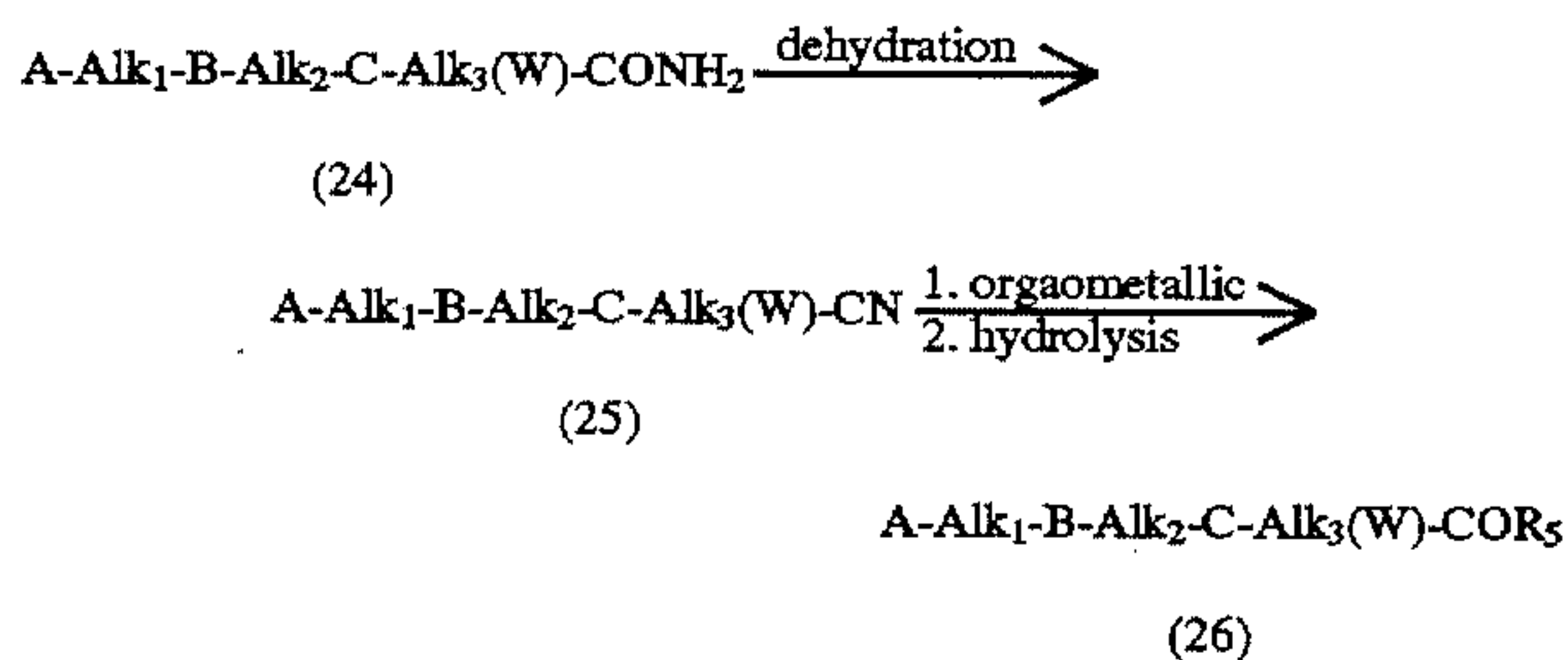
Scheme 10 Generic Preparation of Ketones
