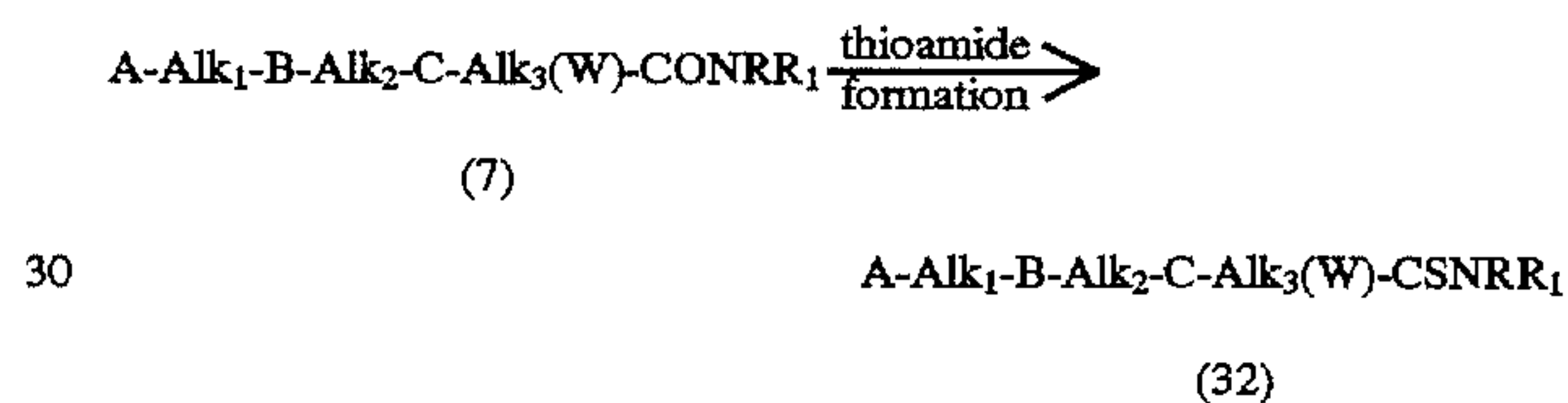
Scheme 14 Generic Preparation of Thioamides
