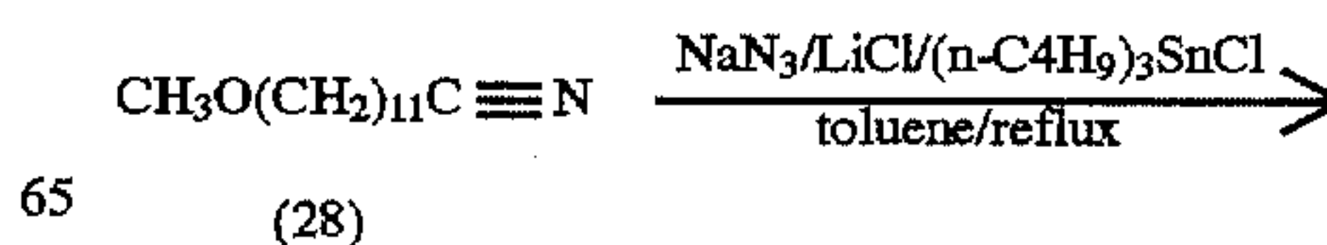
Scheme 17 Preparation of 5-(11-Methoxyundecyl)-1H-tetrazole
