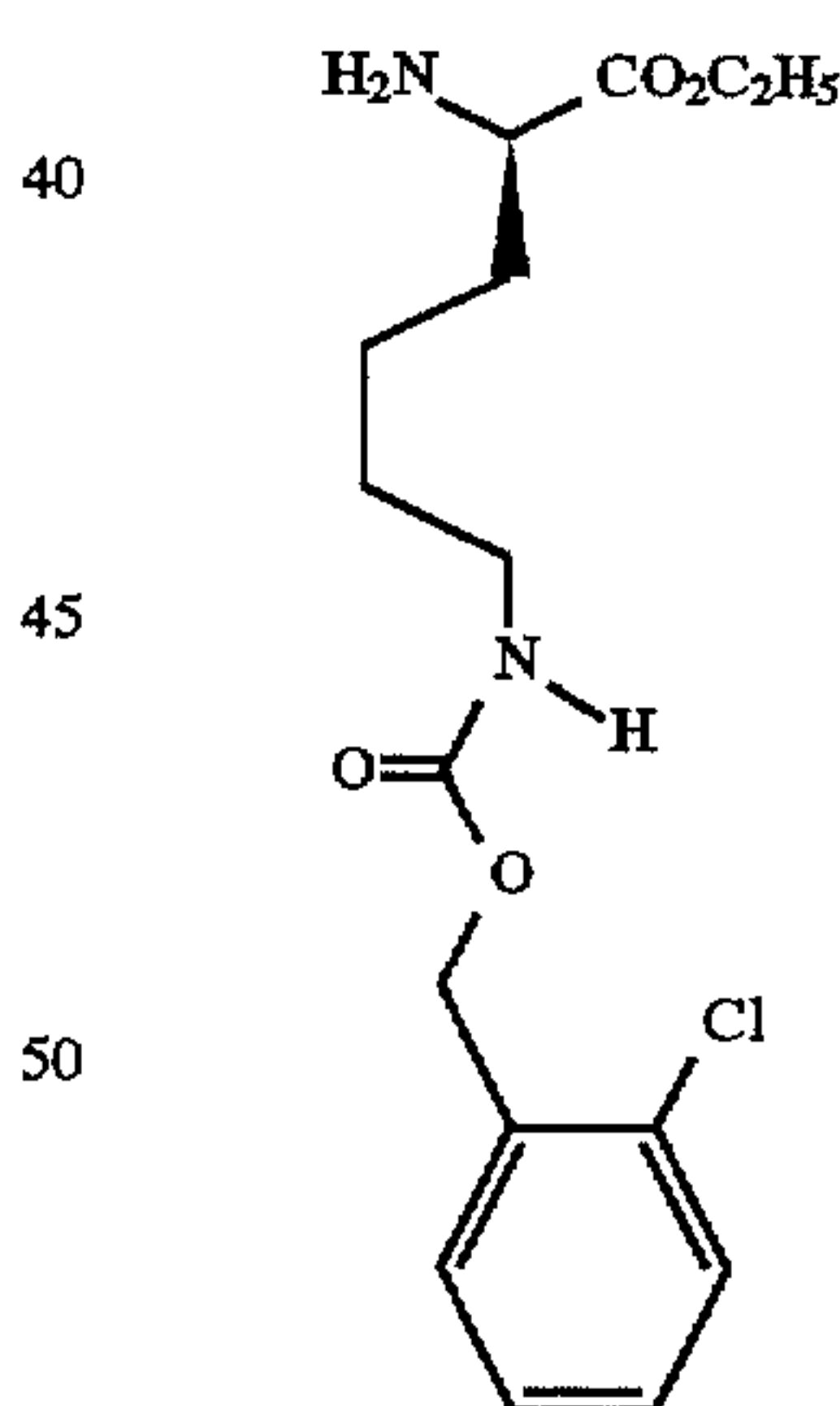
N6-[[[(2-Chlorophenyl)methoxy]carbonyl]-N2-(12-methoxy-1-oxododecyl)-L-lysine, ethyl ester
