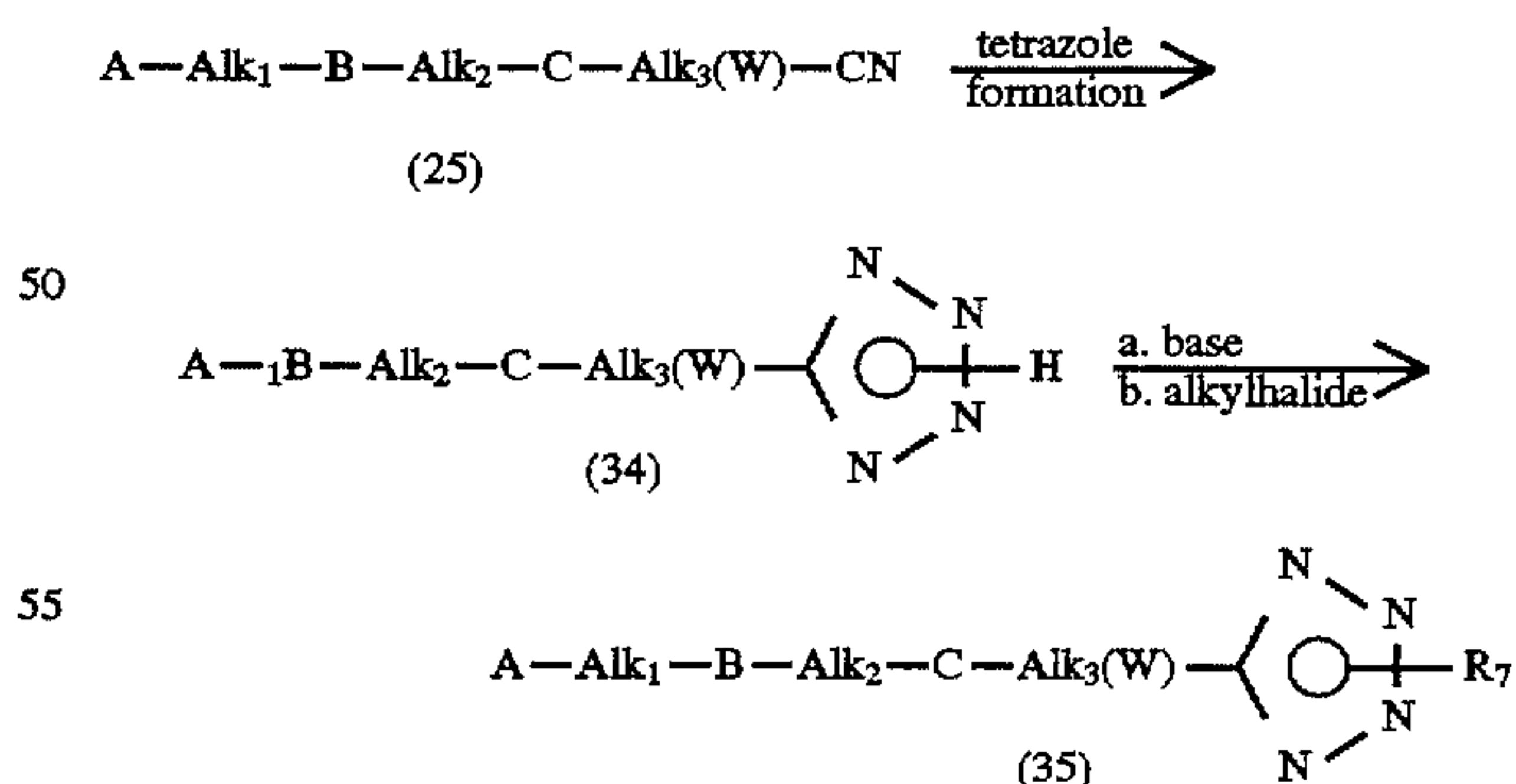
Scheme 16 Generic Preparation of Tetrazoles
