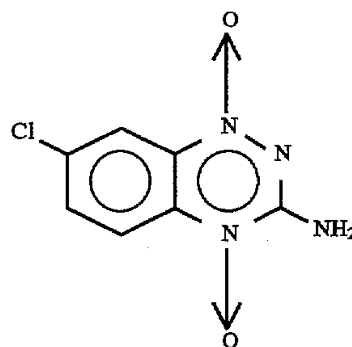
12 7-chloro-3-amino-1,2,4-benzotriazine-1,4-dioxide
