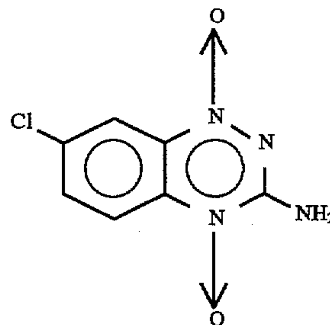
12 7-chloro-3-amino-1,2,4-benzotriazine-1,4-dioxide
