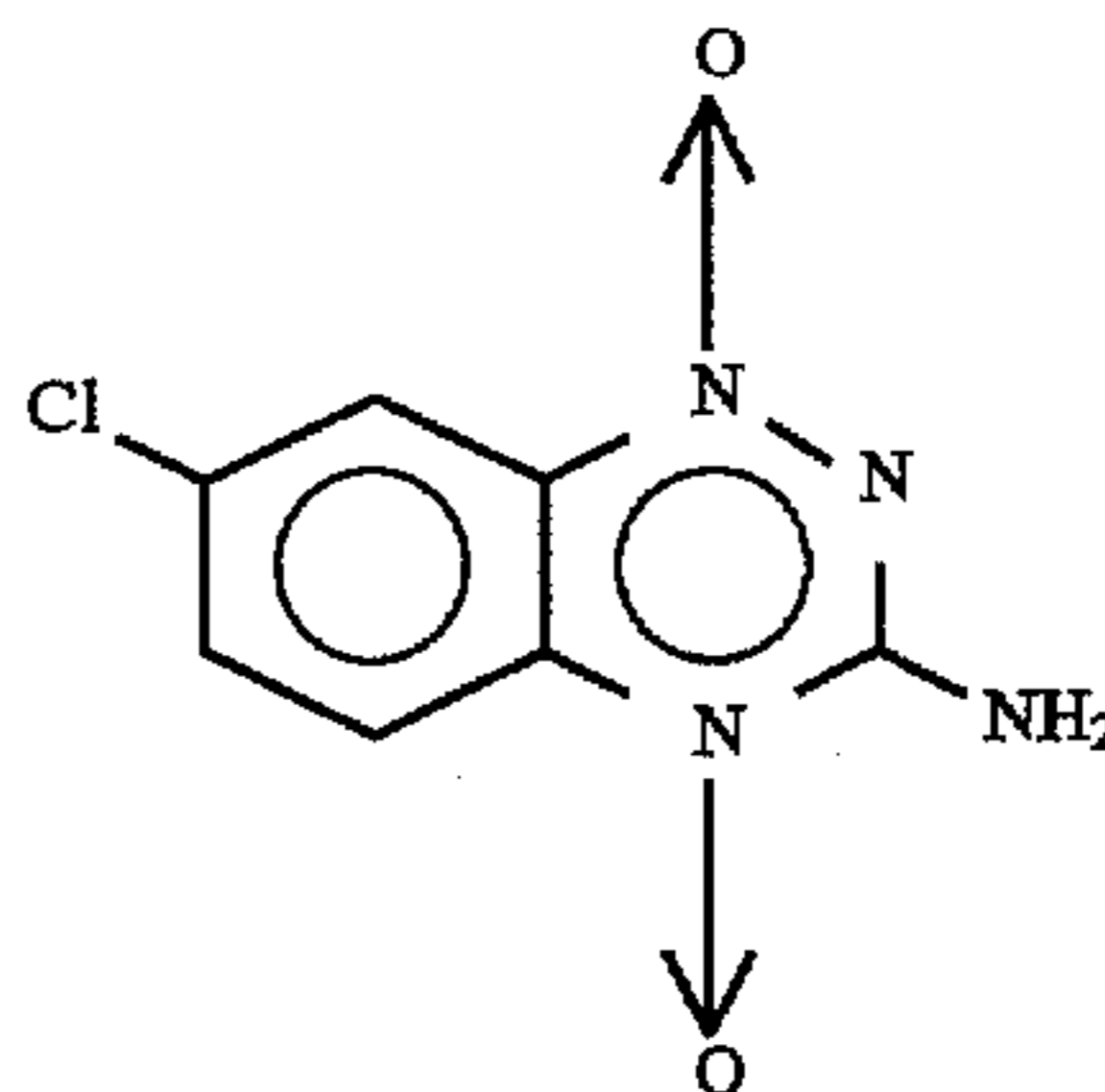
12 7-chloro-3-amino-1,2,4-benzotriazine-1,4-dioxide
