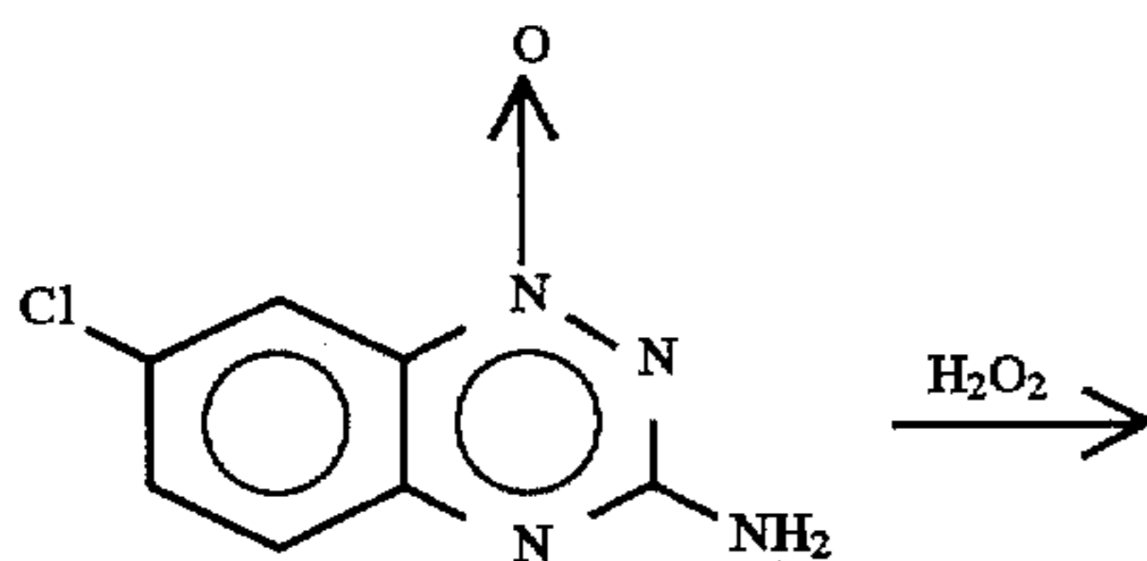
10 7-chloro-3-amino-1,2,4-benzotriazine-1-oxide
