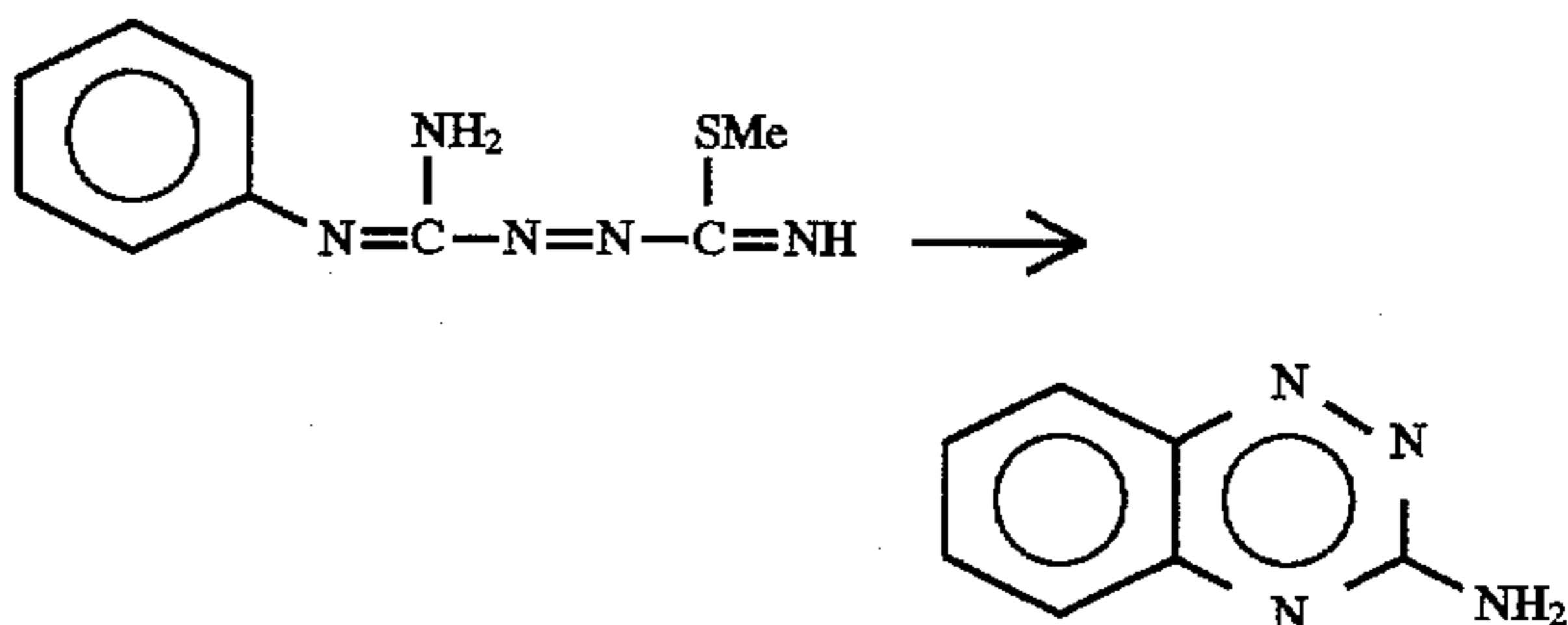
Scheme III
