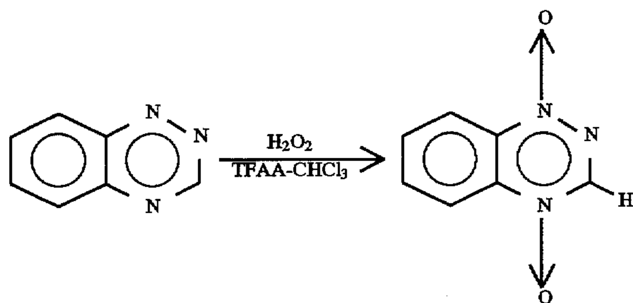
8 1,2,4-benzotriazine
