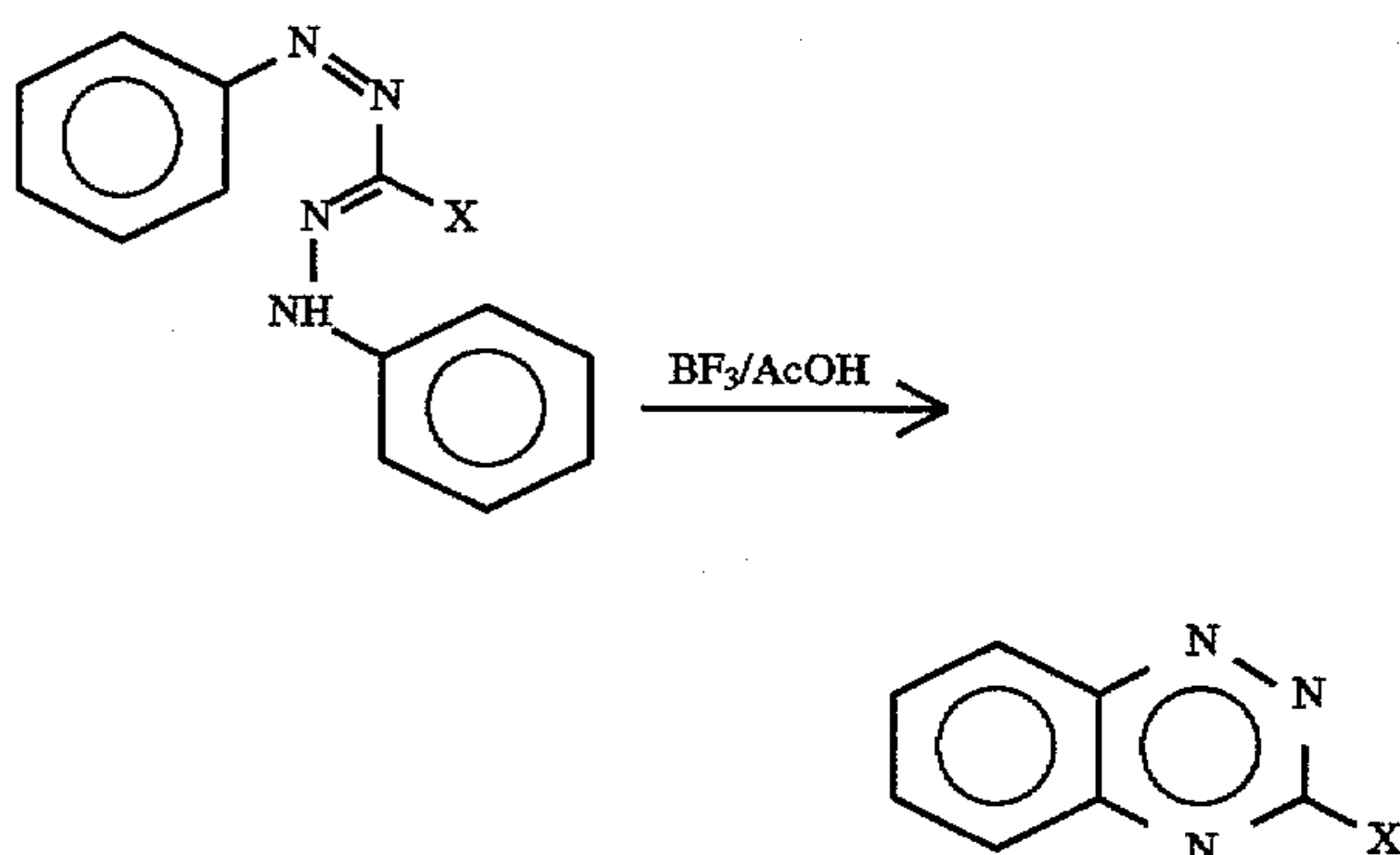
Scheme II
