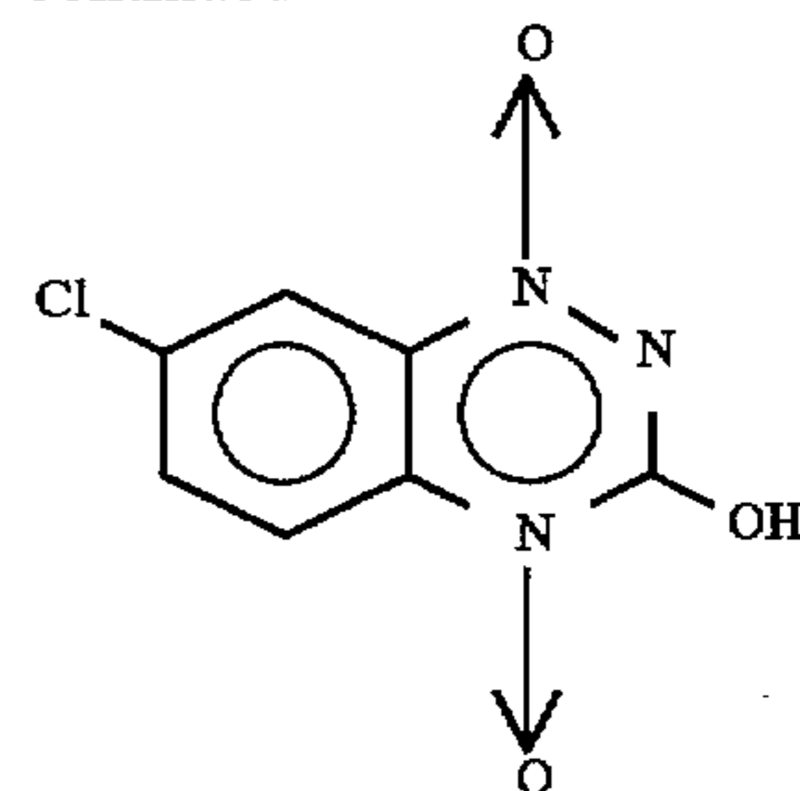
11 7-chloro-3-hydroxy-1,2,4-benzotriazine-1,4-dioxide
