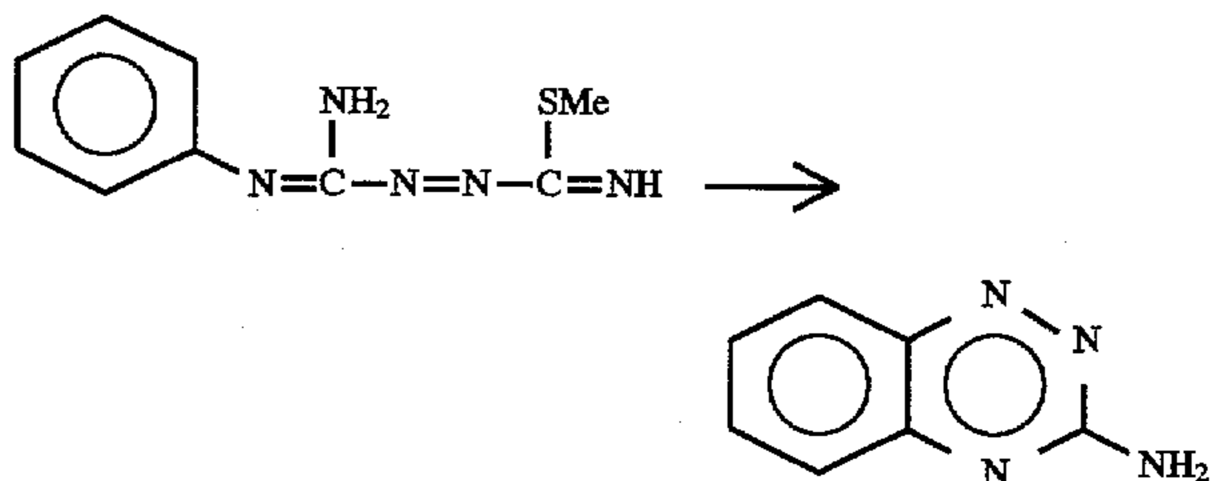
Scheme III
