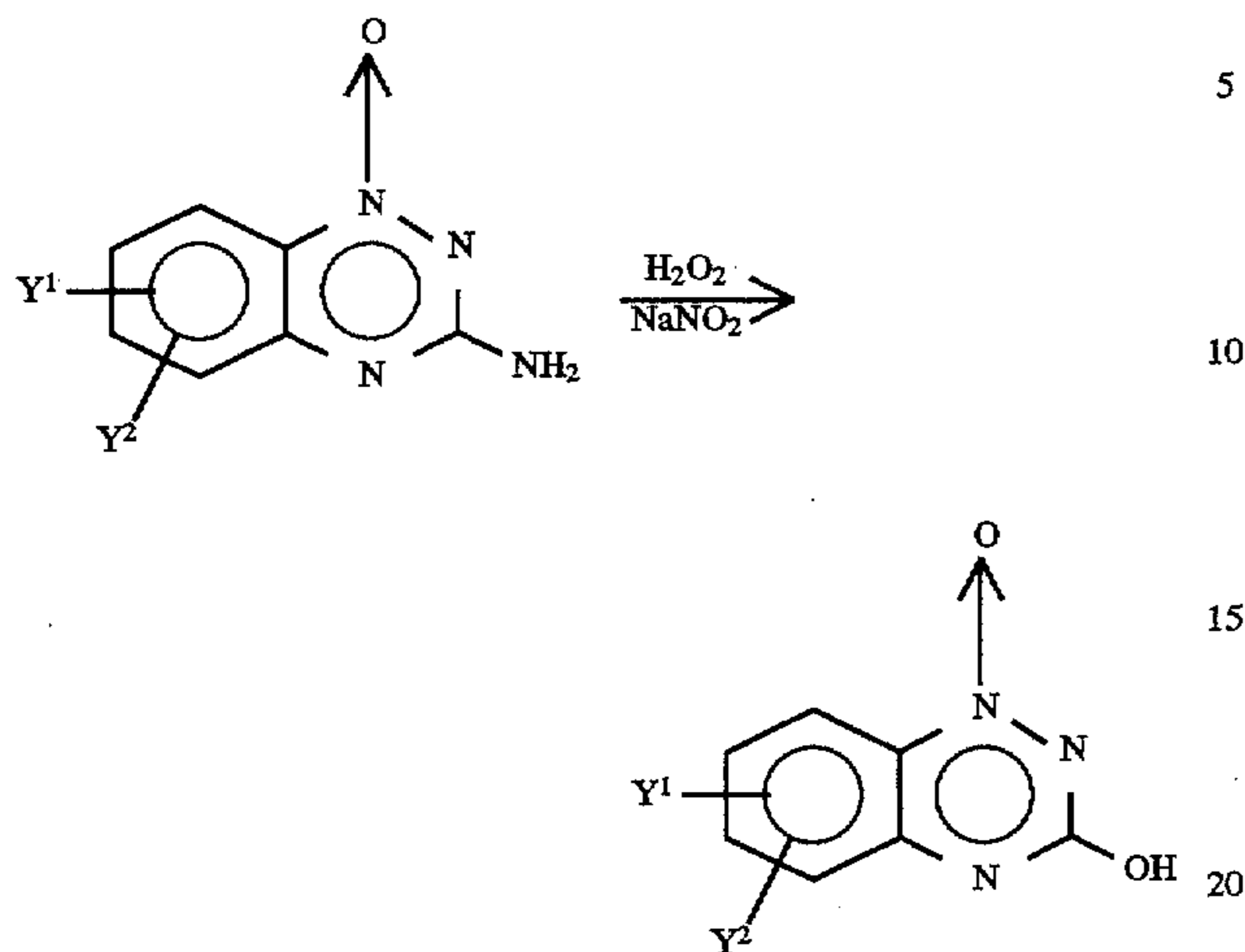
Scheme IV
