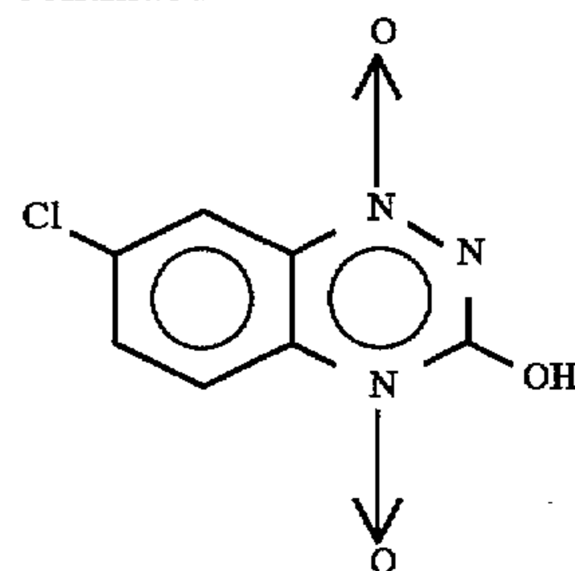
11 7-chloro-3-hydroxy-1,2,4-benzotriazine-1,4-dioxide
