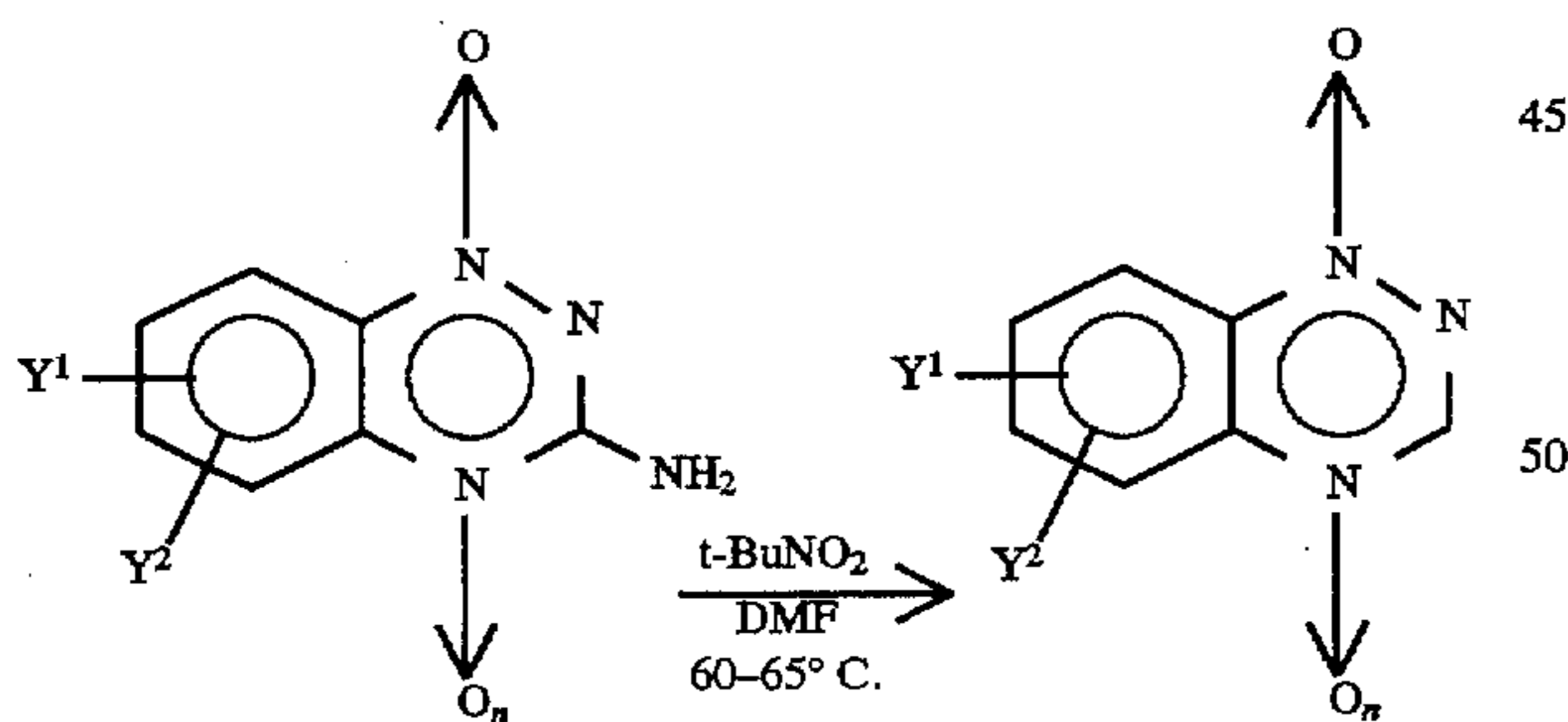
Scheme V
