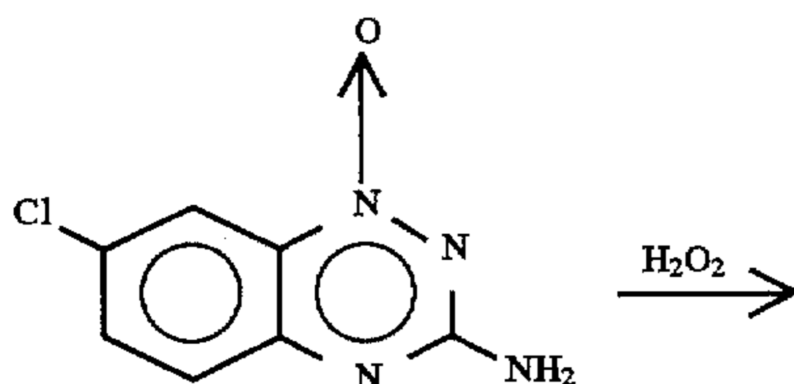
10 7-chloro-3-amino-1,2,4-benzotriazine-1-oxide
