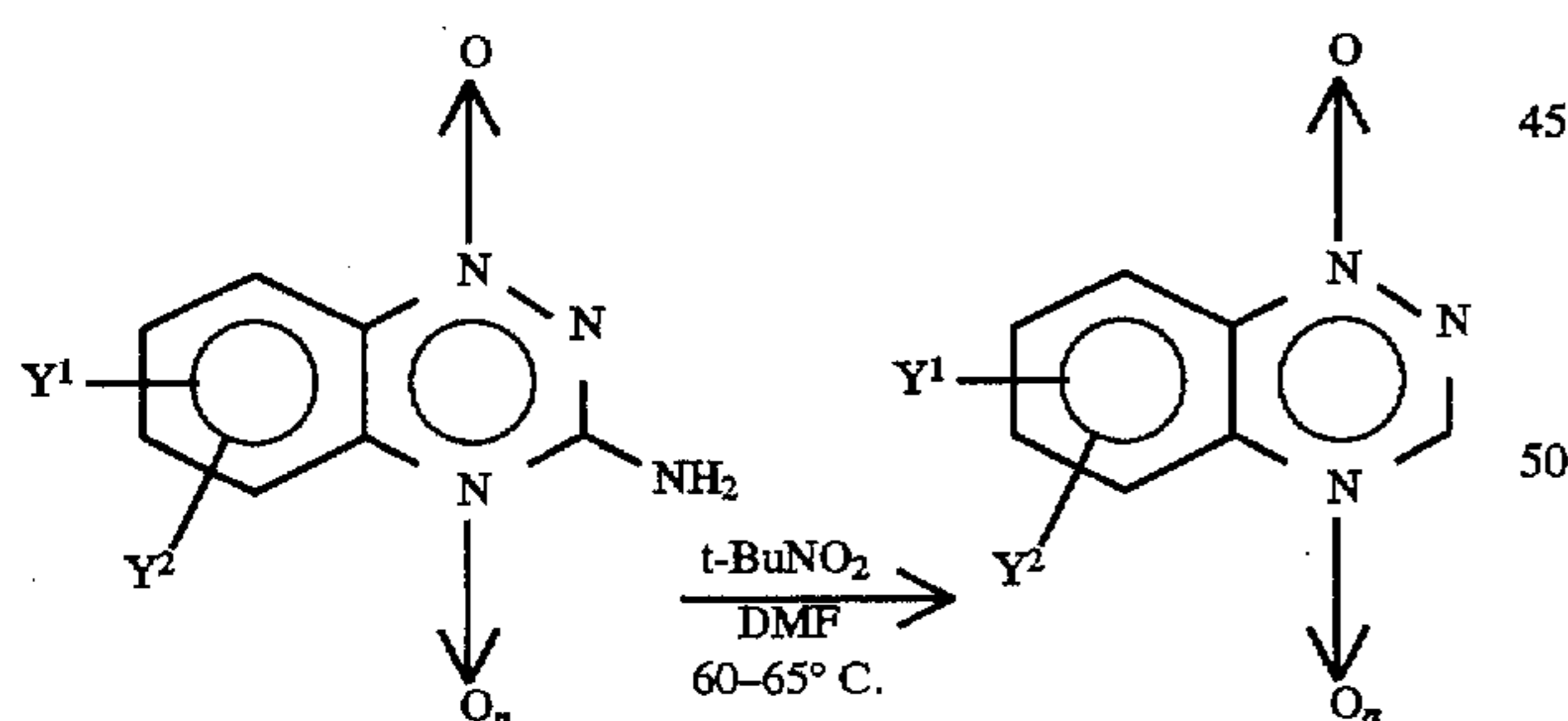
Scheme V
