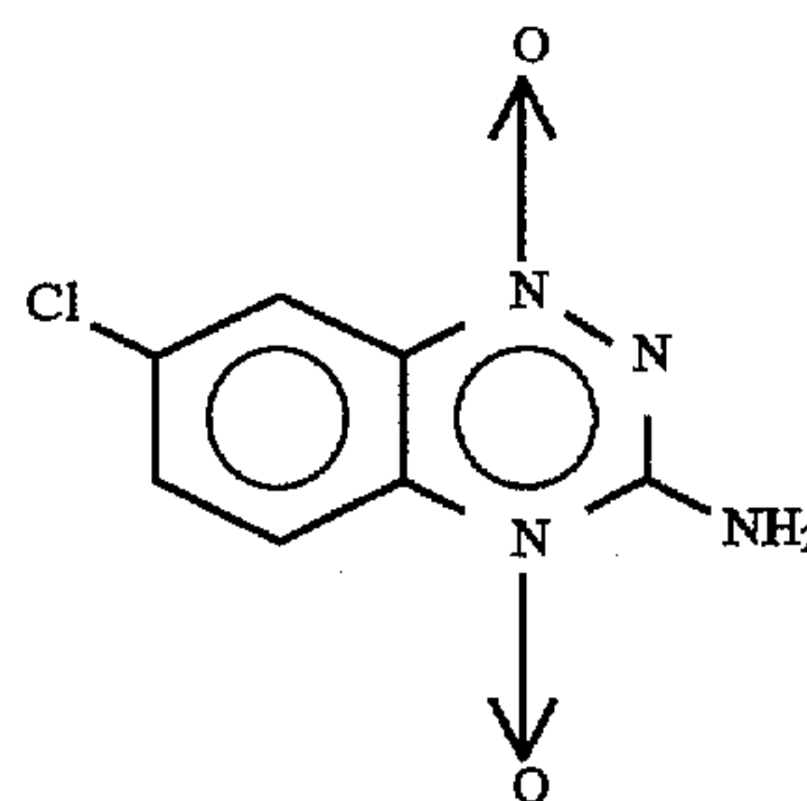
12 7-chloro-3-amino-1,2,4-benzotriazine-1,4-dioxide
