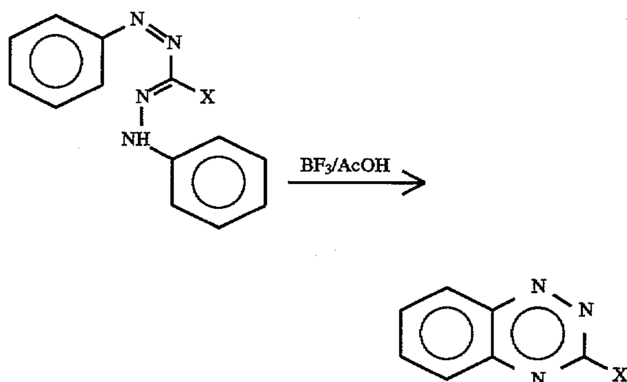
Scheme II
