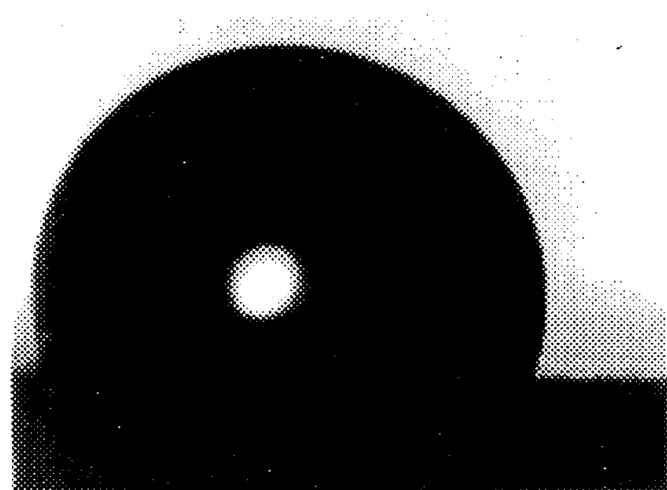
CONTACT ANGLE WITH TEFLON (110°)
