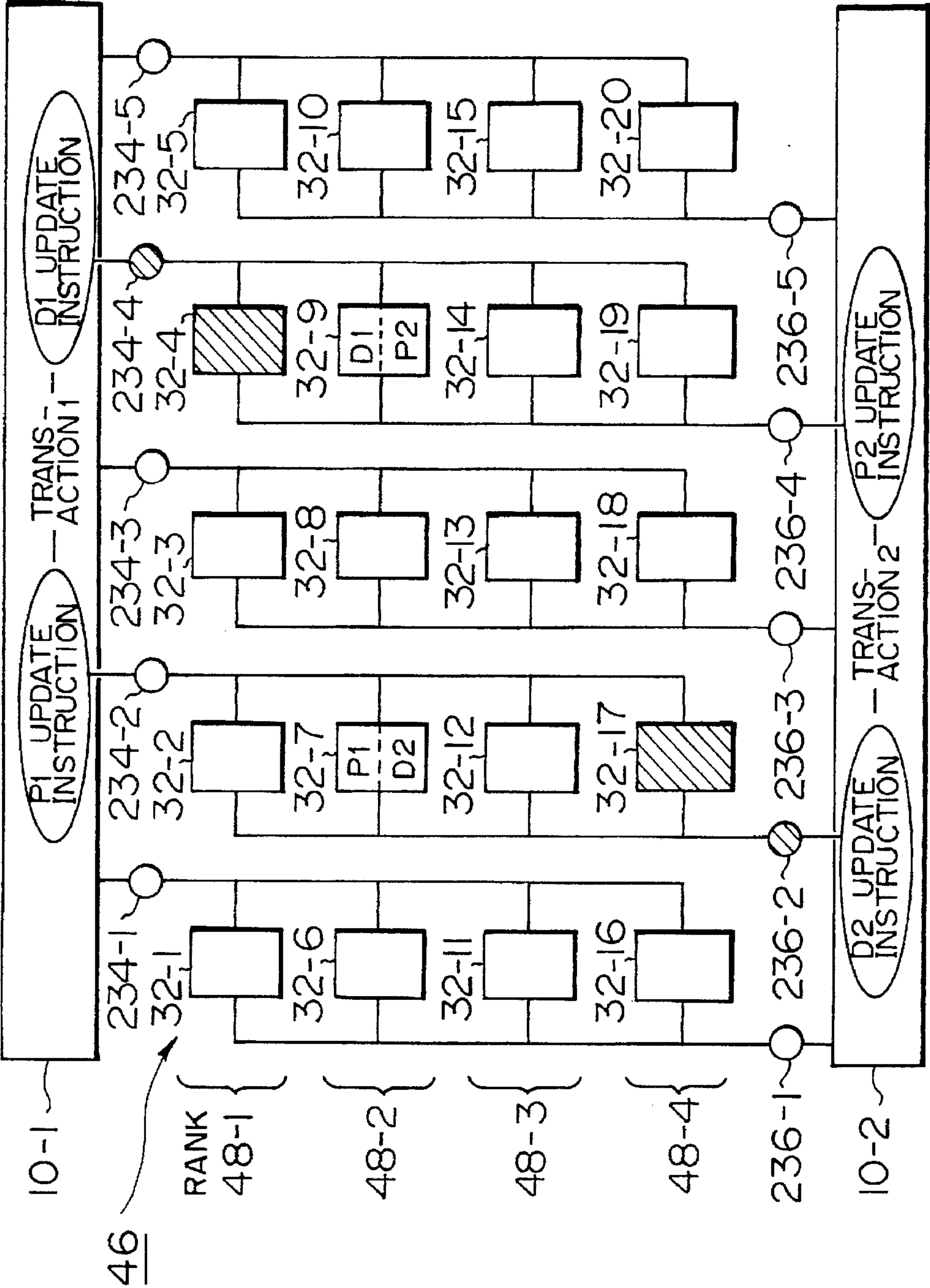
FIG. 9 PRIOR ART
