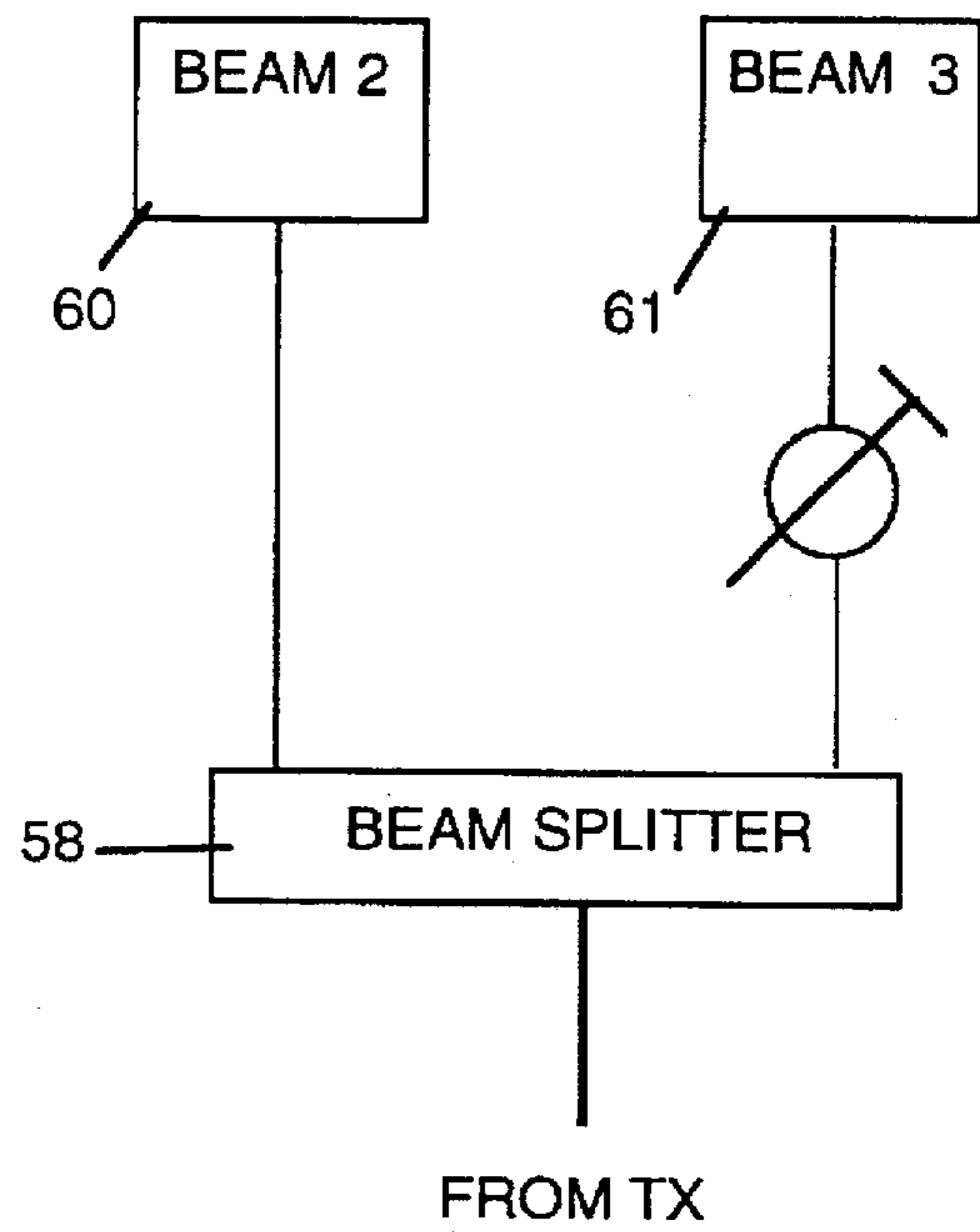
Fig. 14 (b) QUADRATURE
