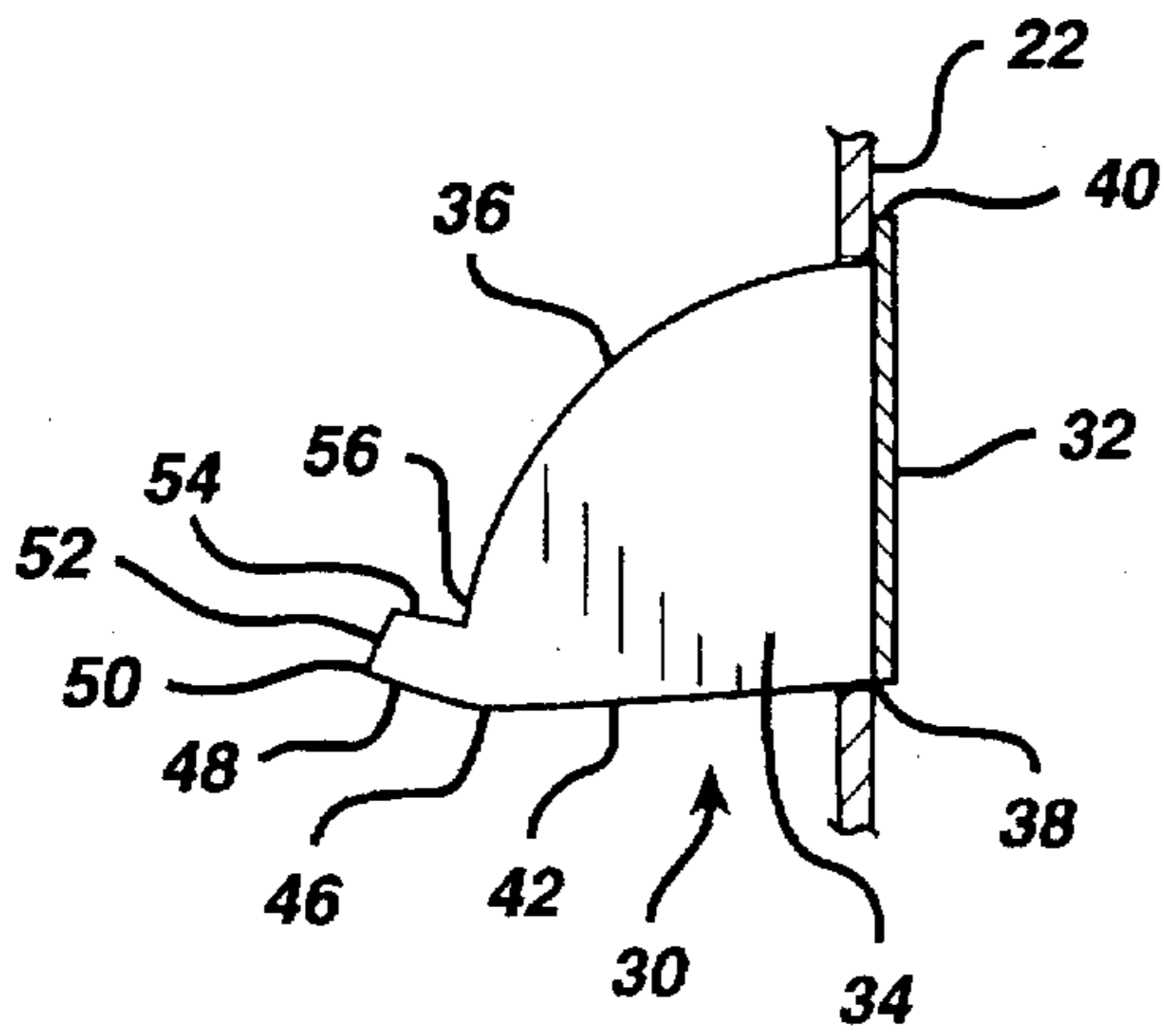
FIG. 18 PRIOR ART
