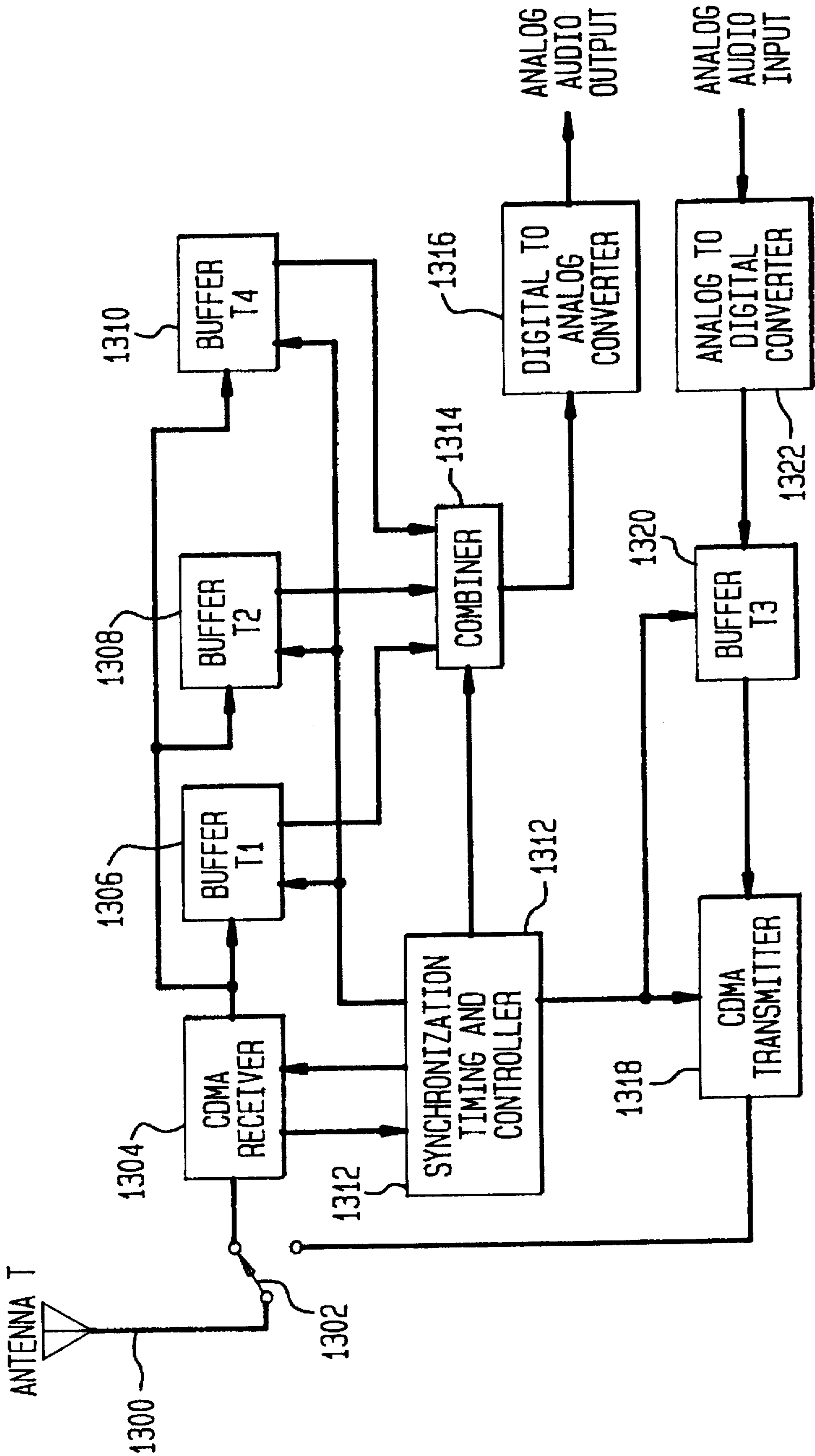
FIG. 13 SUBSCRIBER STATION
