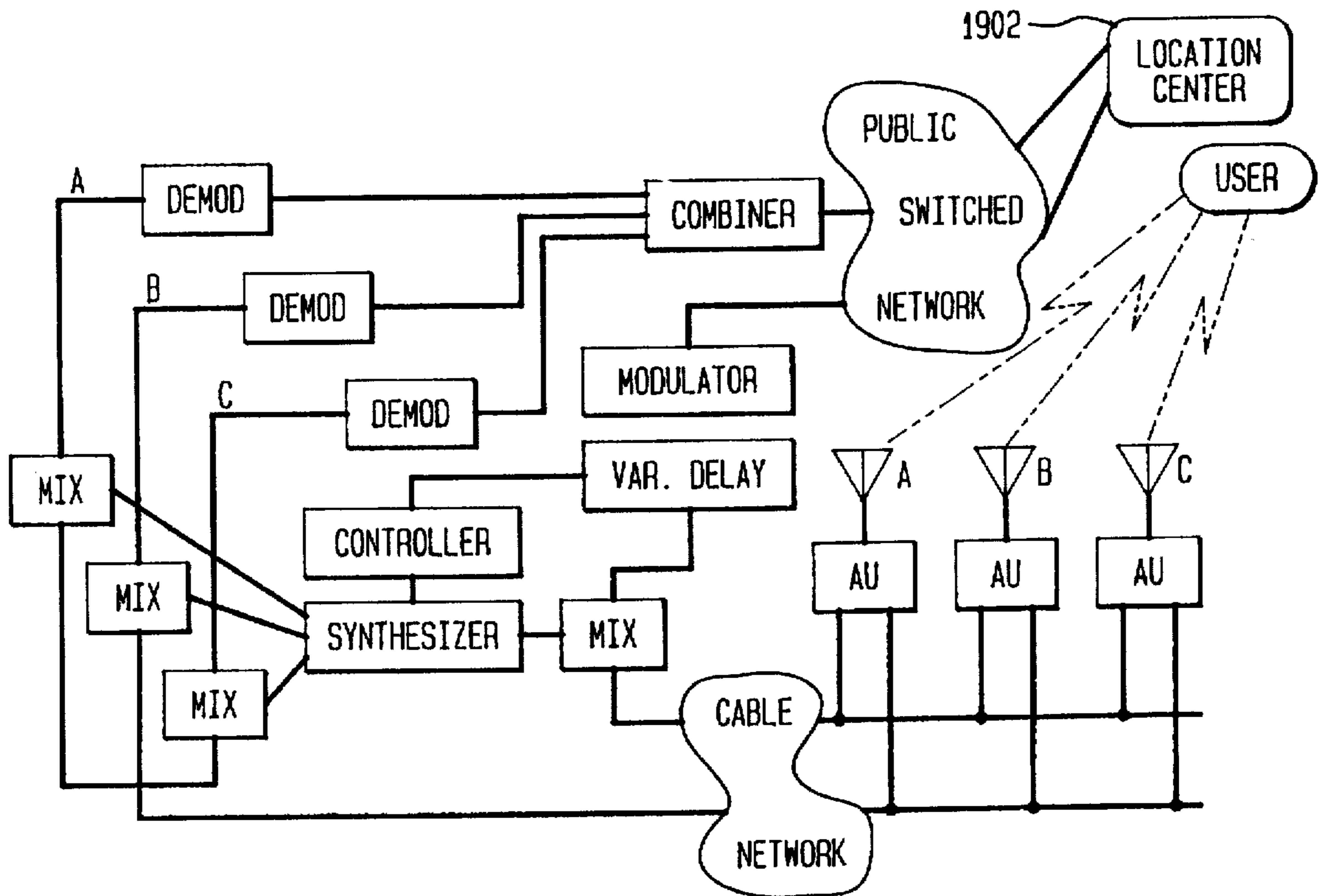
LOCATION CENTER EXTERNAL TO COMMUNICAITON SYSTEM
