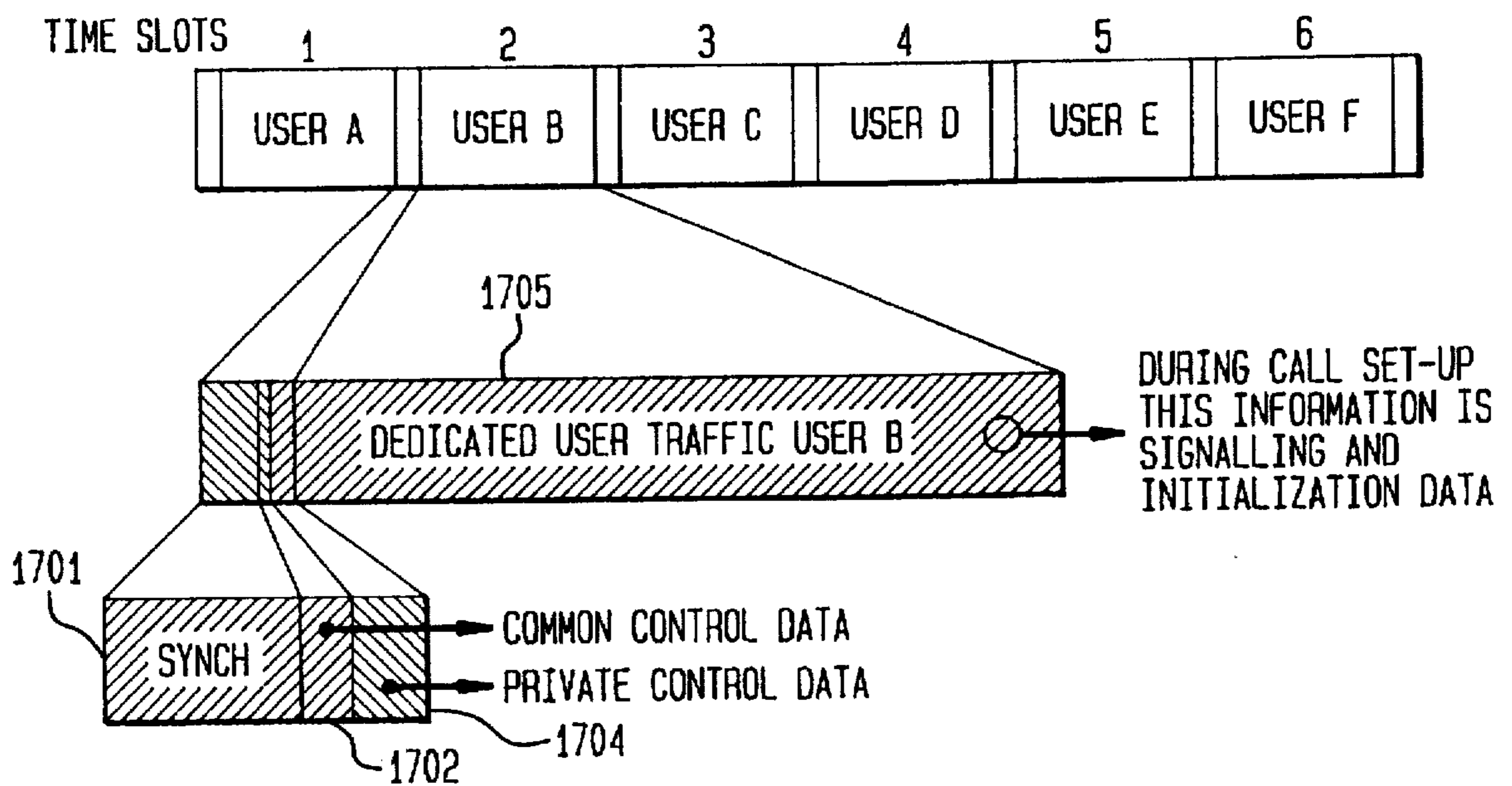
FIG. 17 SYNCH AND CONTROL CHANNEL STRUCTURE
