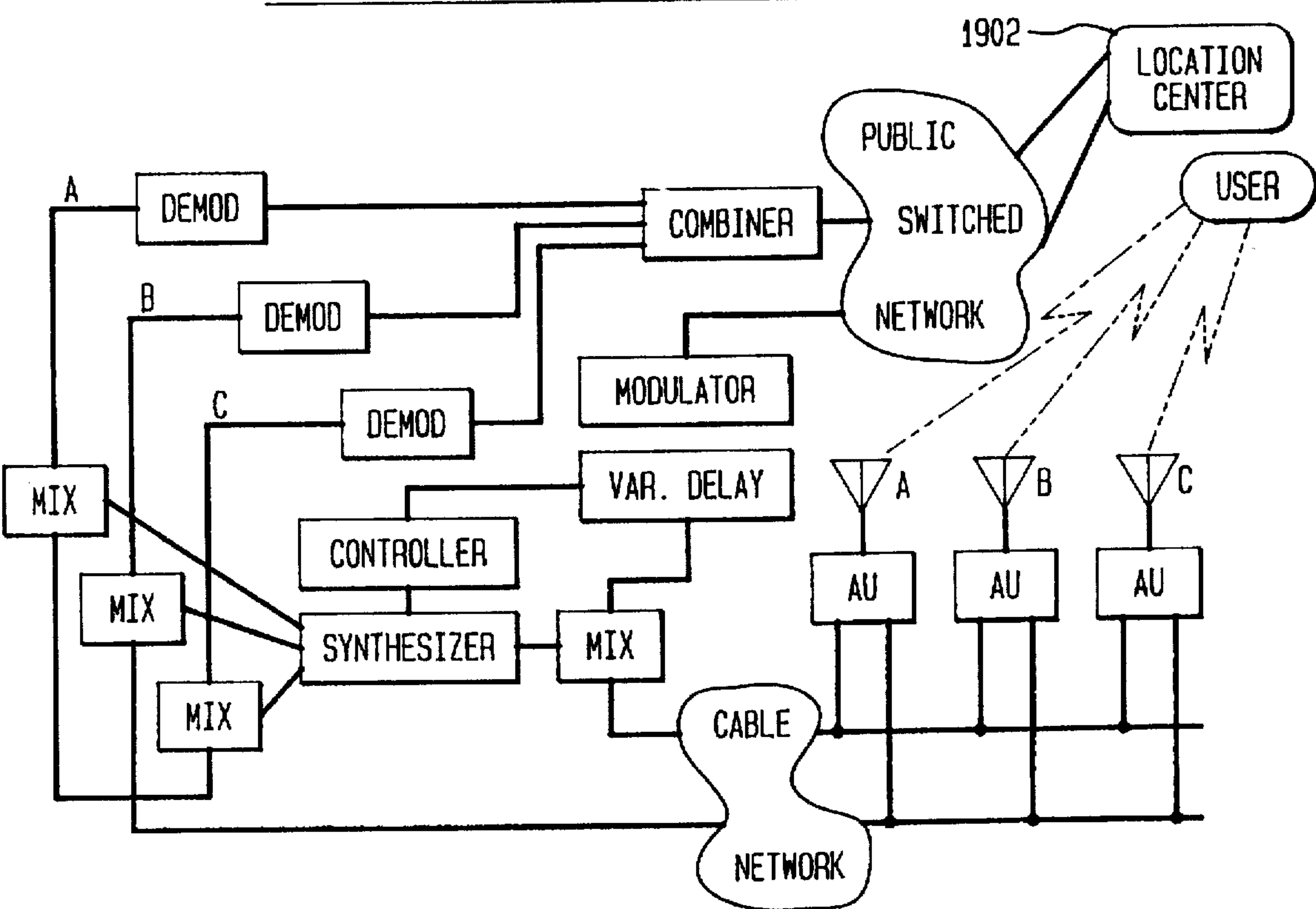
LOCATION CENTER EXTERNAL TO COMMUNICAITON SYSTEM
