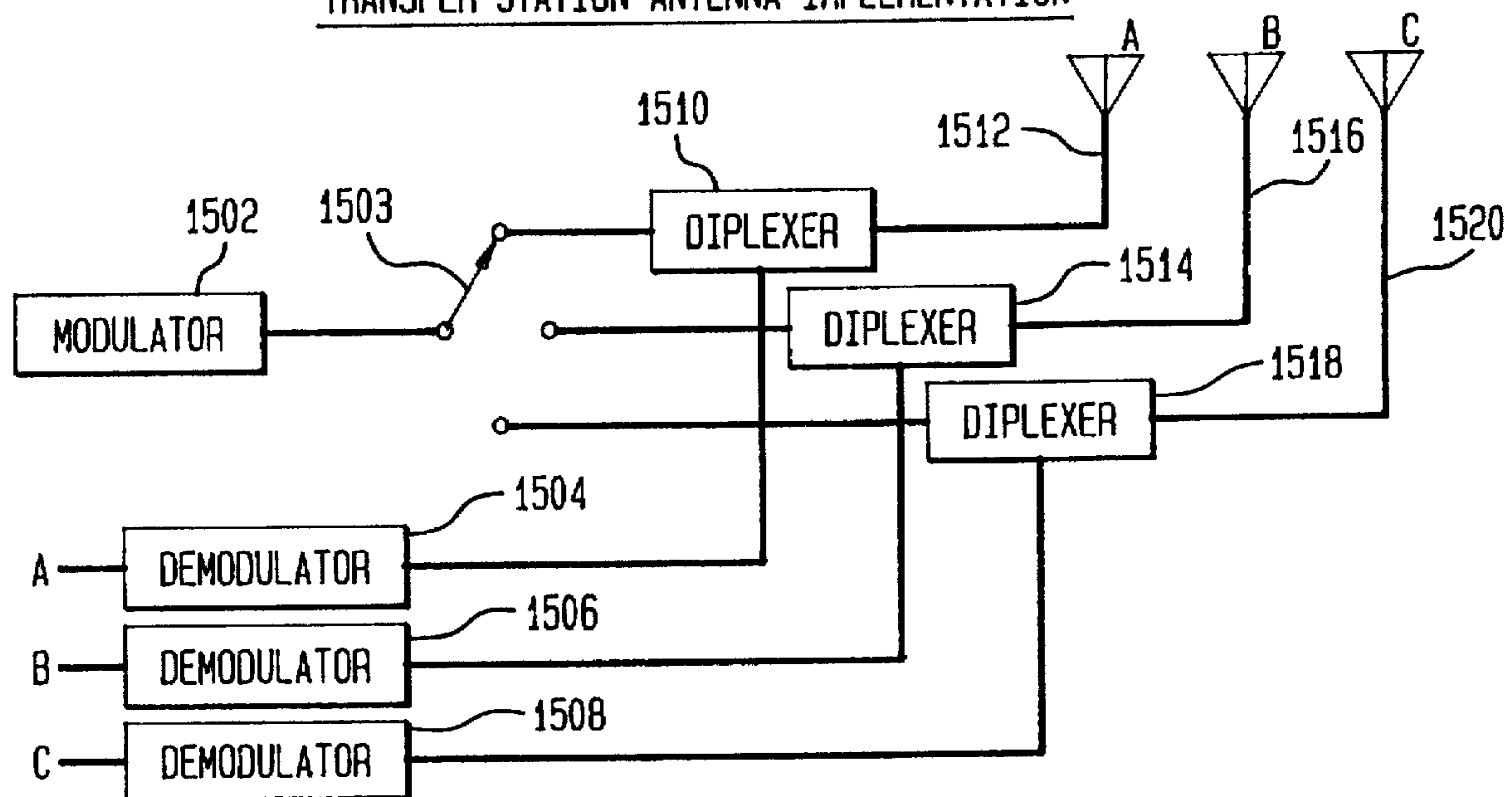
FIG. 15 TRANSFER STATION ANTENNA IMPLEMENTATION
