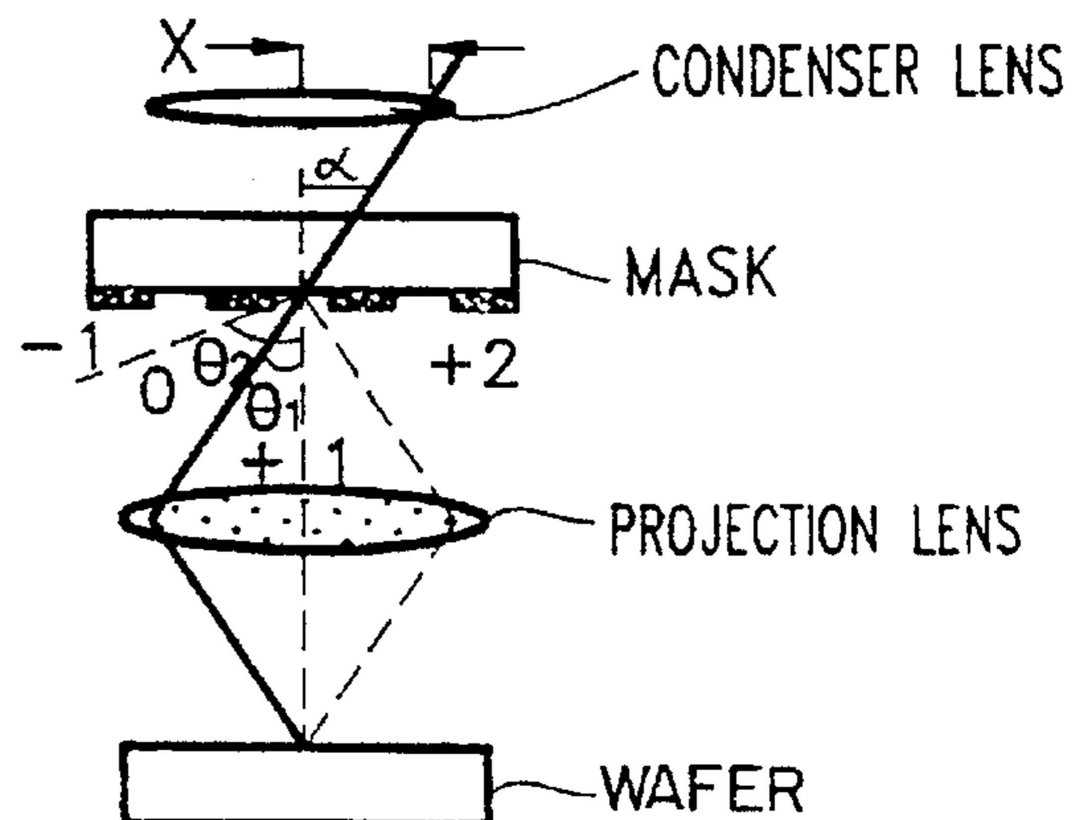
FIG. 4 (PRIOR ART)
