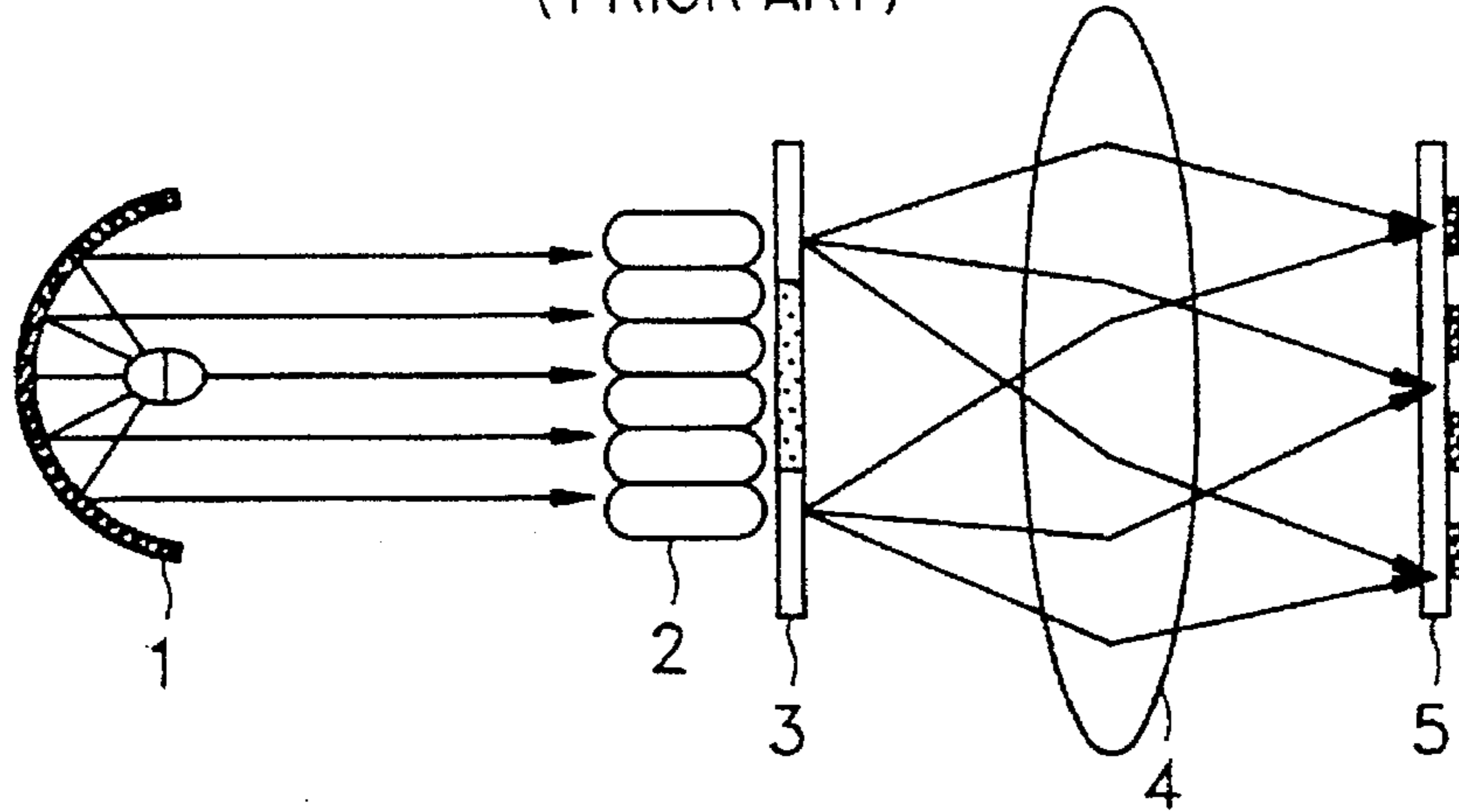
FIG. 1 (PRIOR ART)
