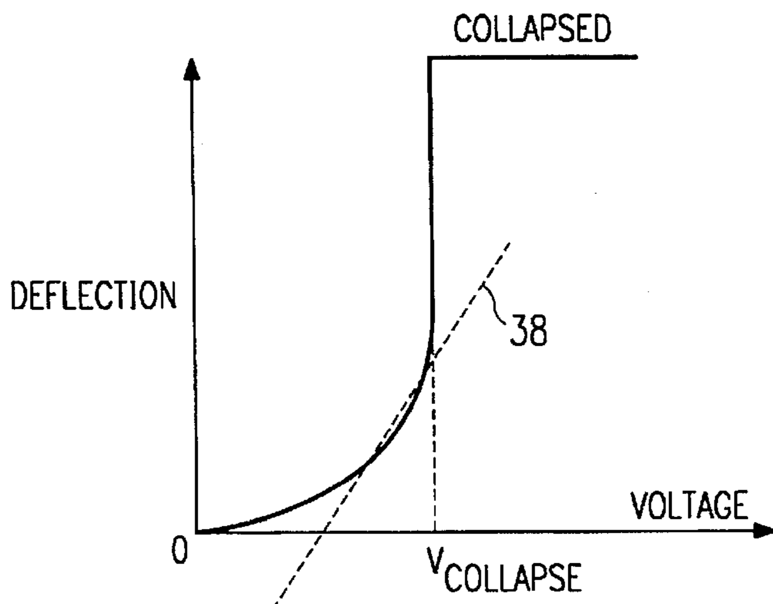
FIG. 1C (PRIOR ART)
