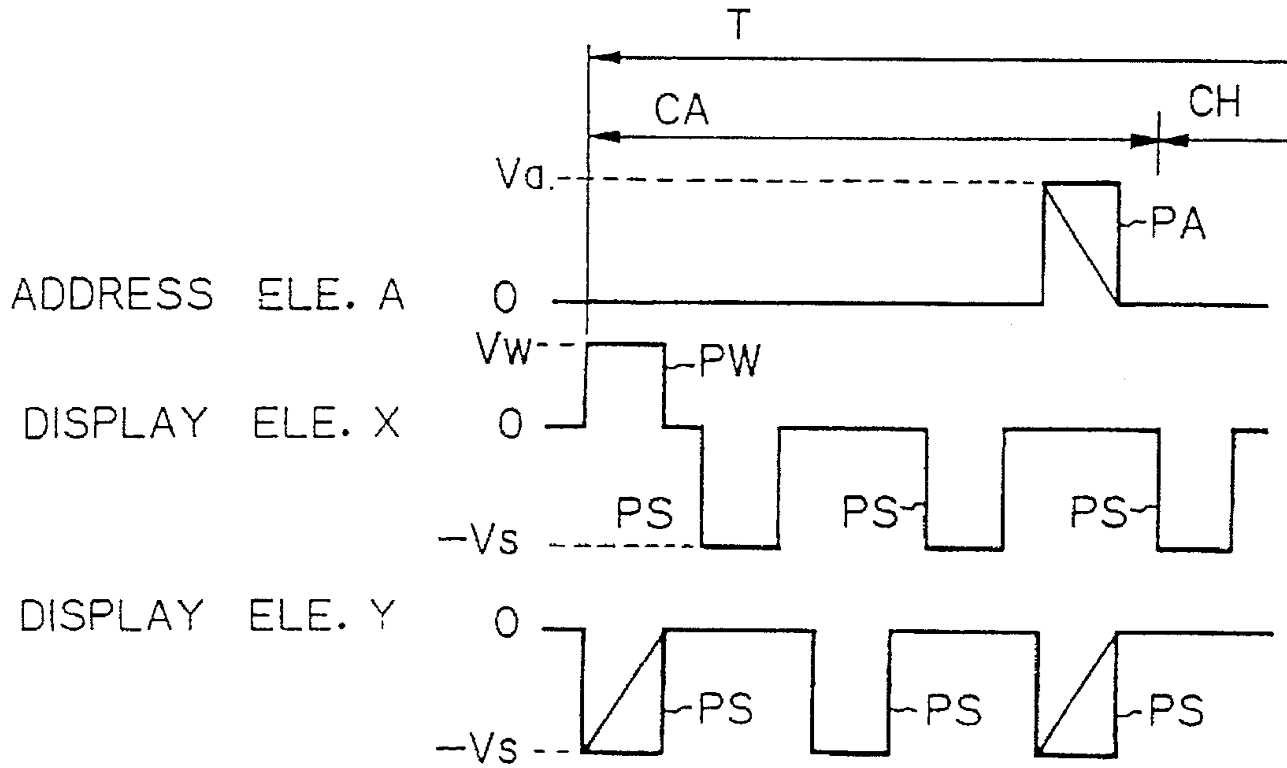
Fig. 5 PRIOR ART
