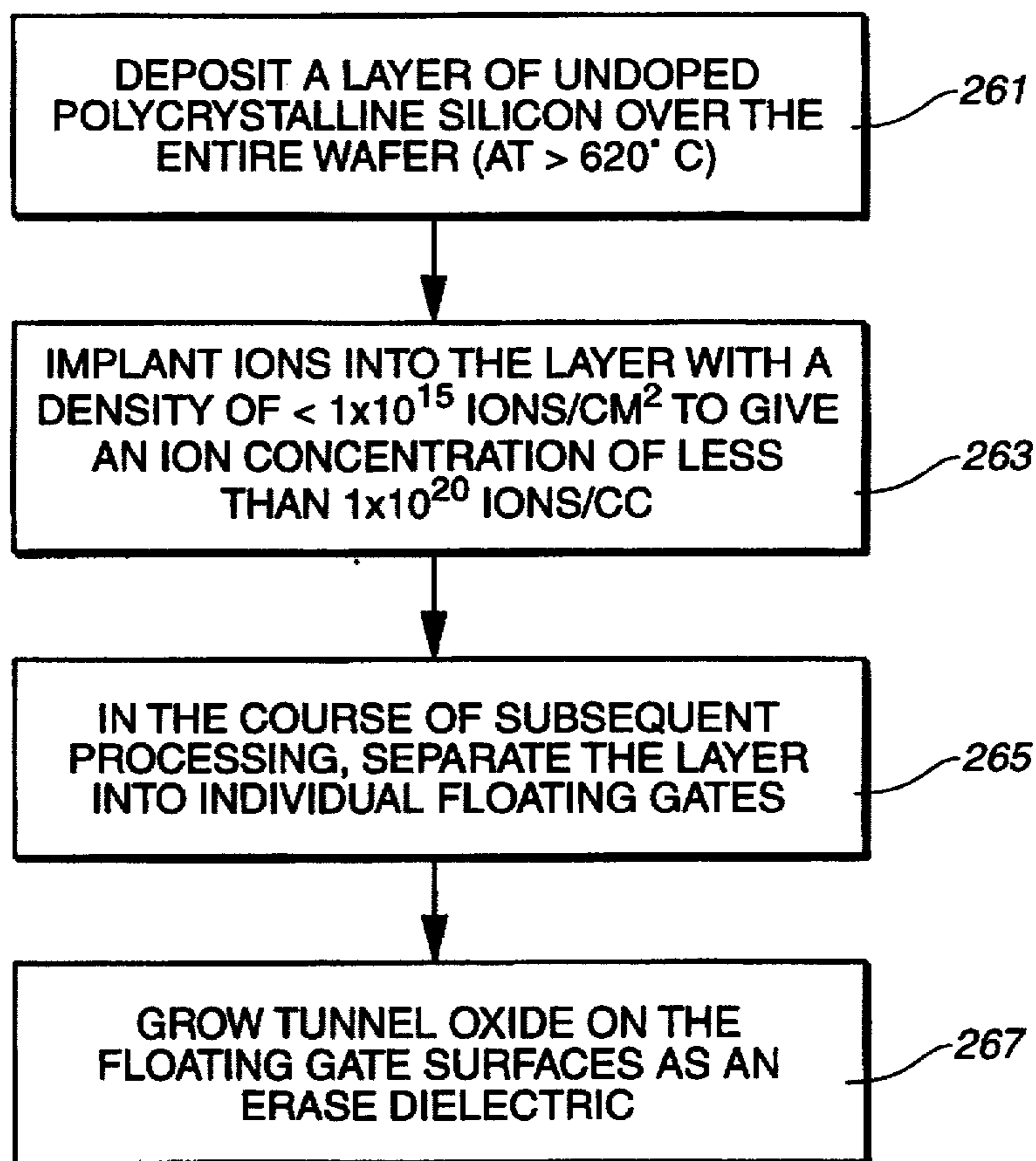
FIG. 27 (POLY I FORMATION PROCESS)
