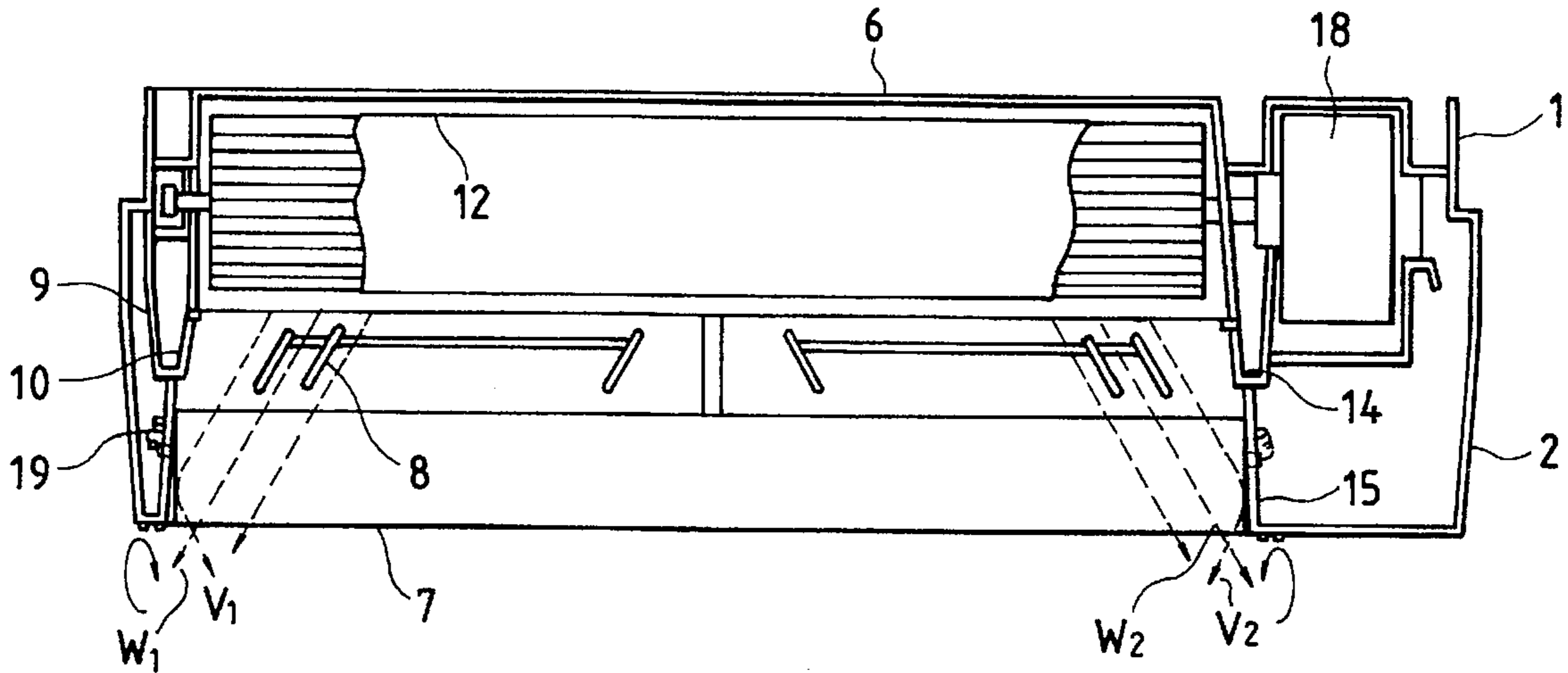
FIG. 62 PRIOR ART
