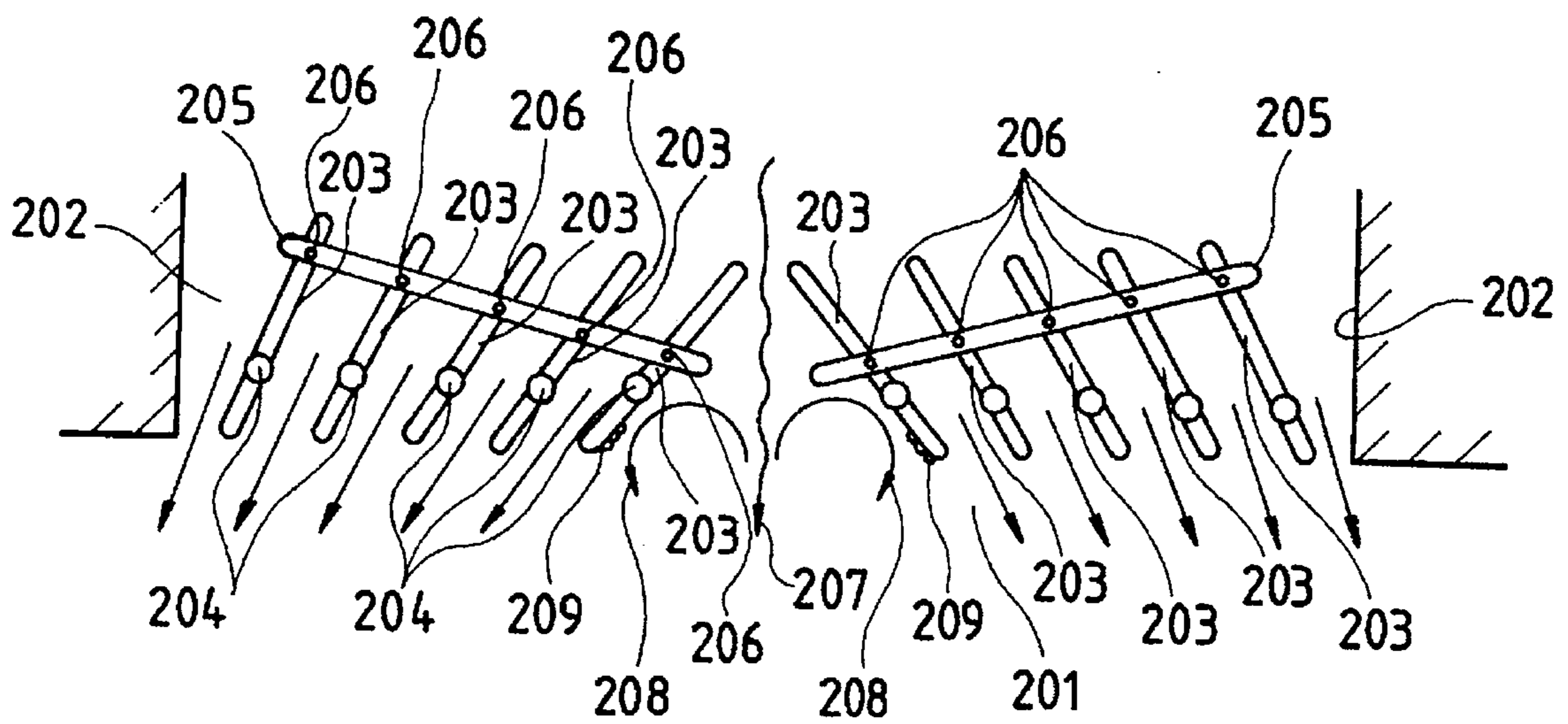
FIG. 66 PRIOR ART
