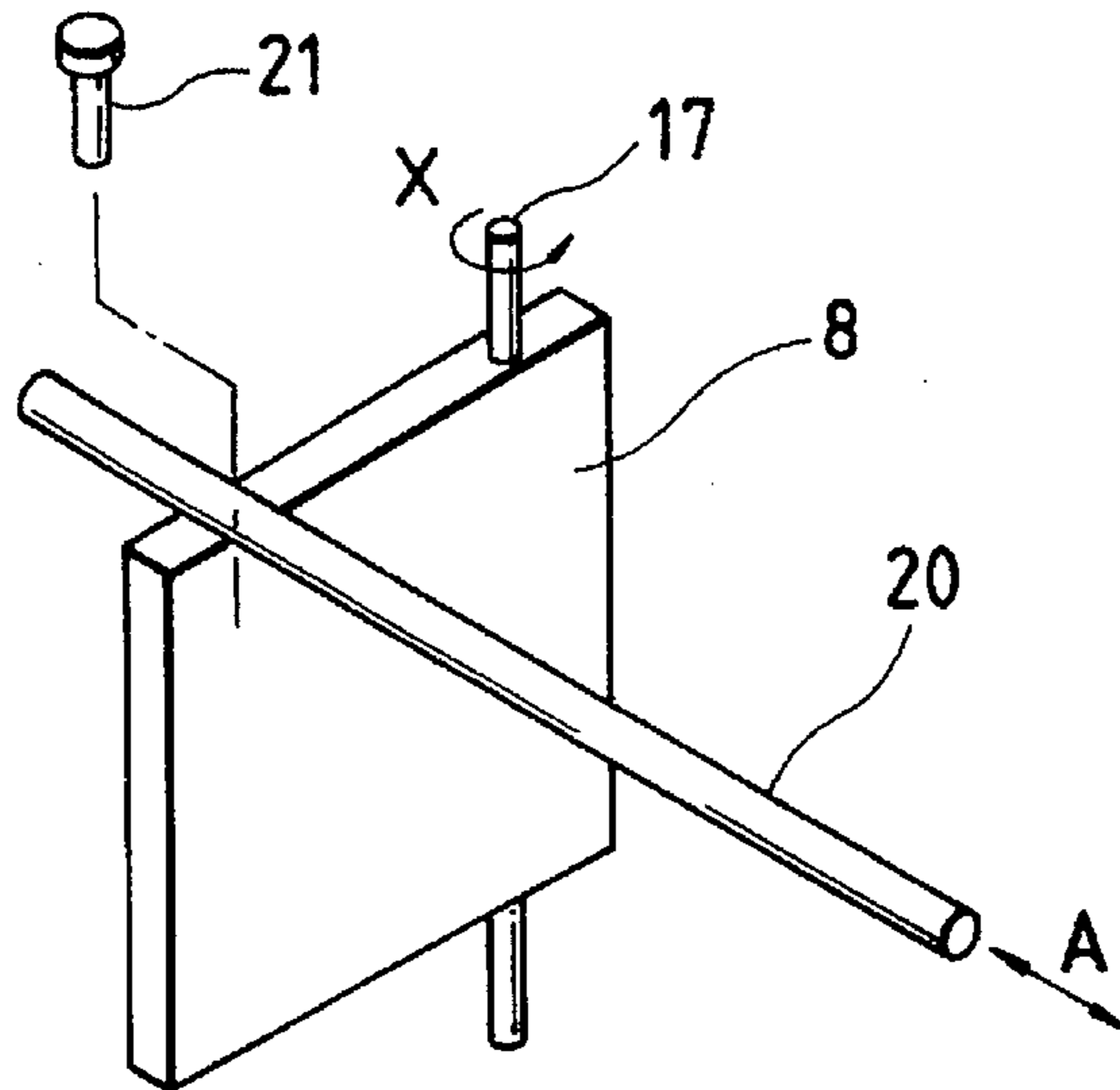
FIG. 64 PRIOR ART
