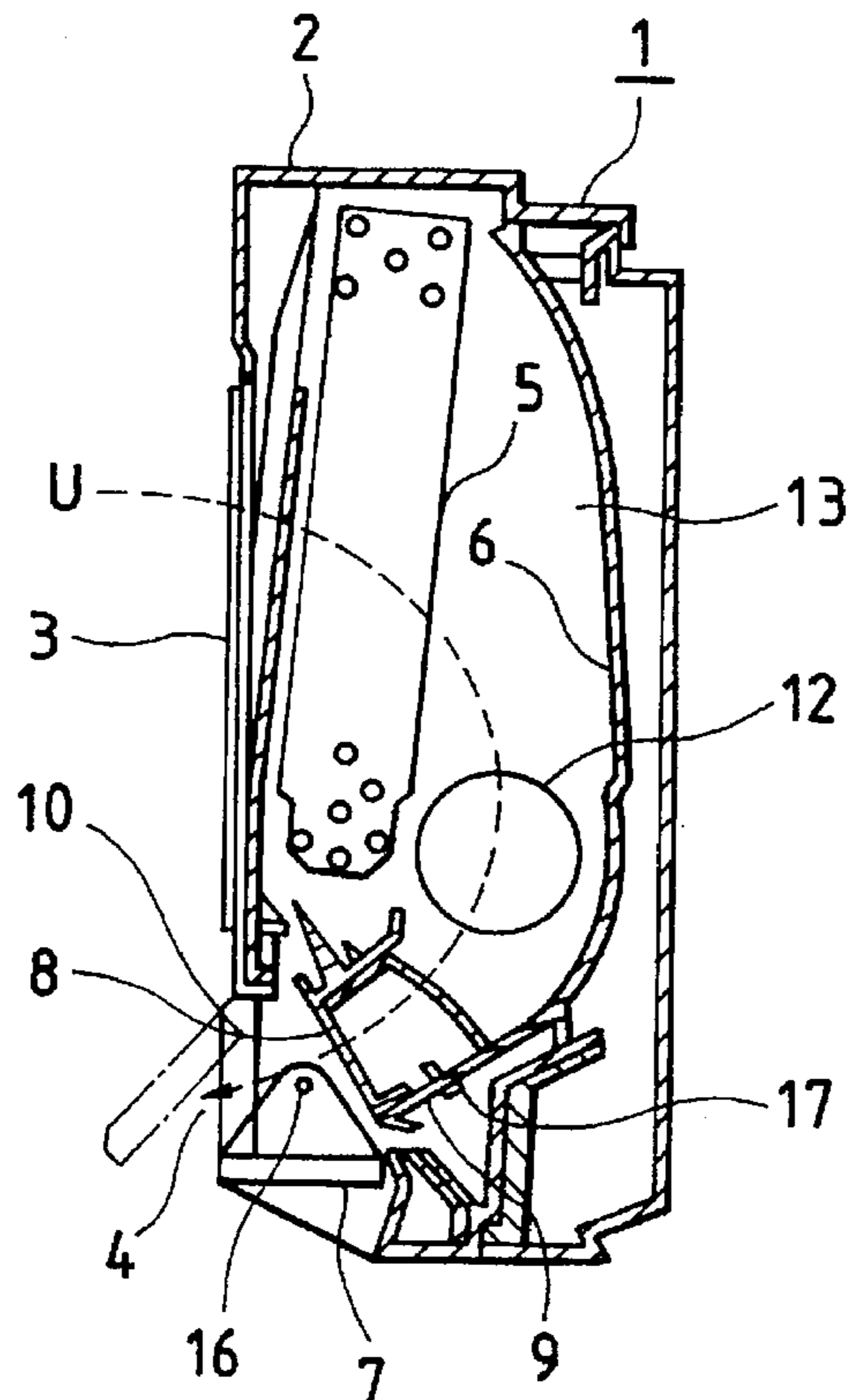
FIG. 61 PRIOR ART
