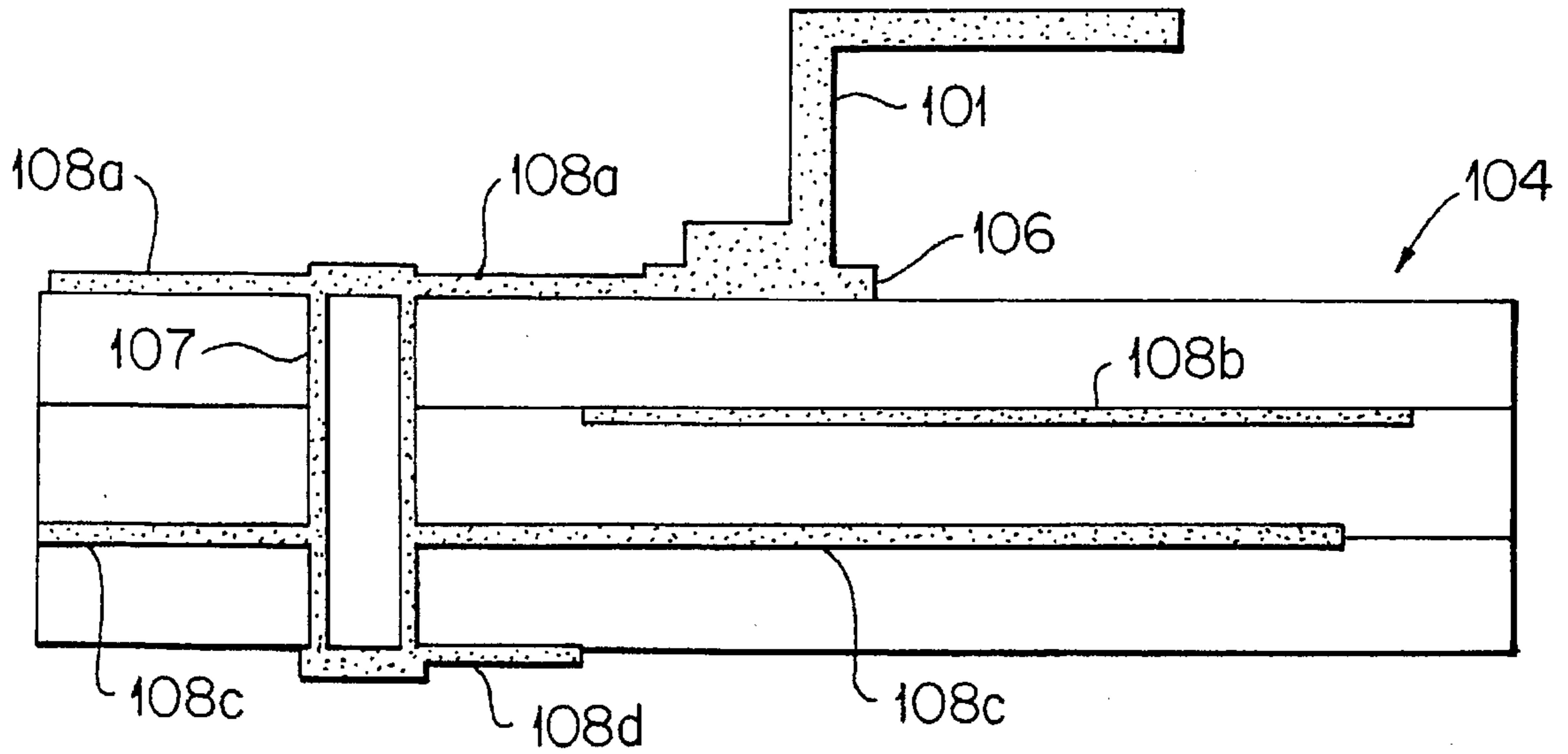
FIG. 6 PRIOR ART
