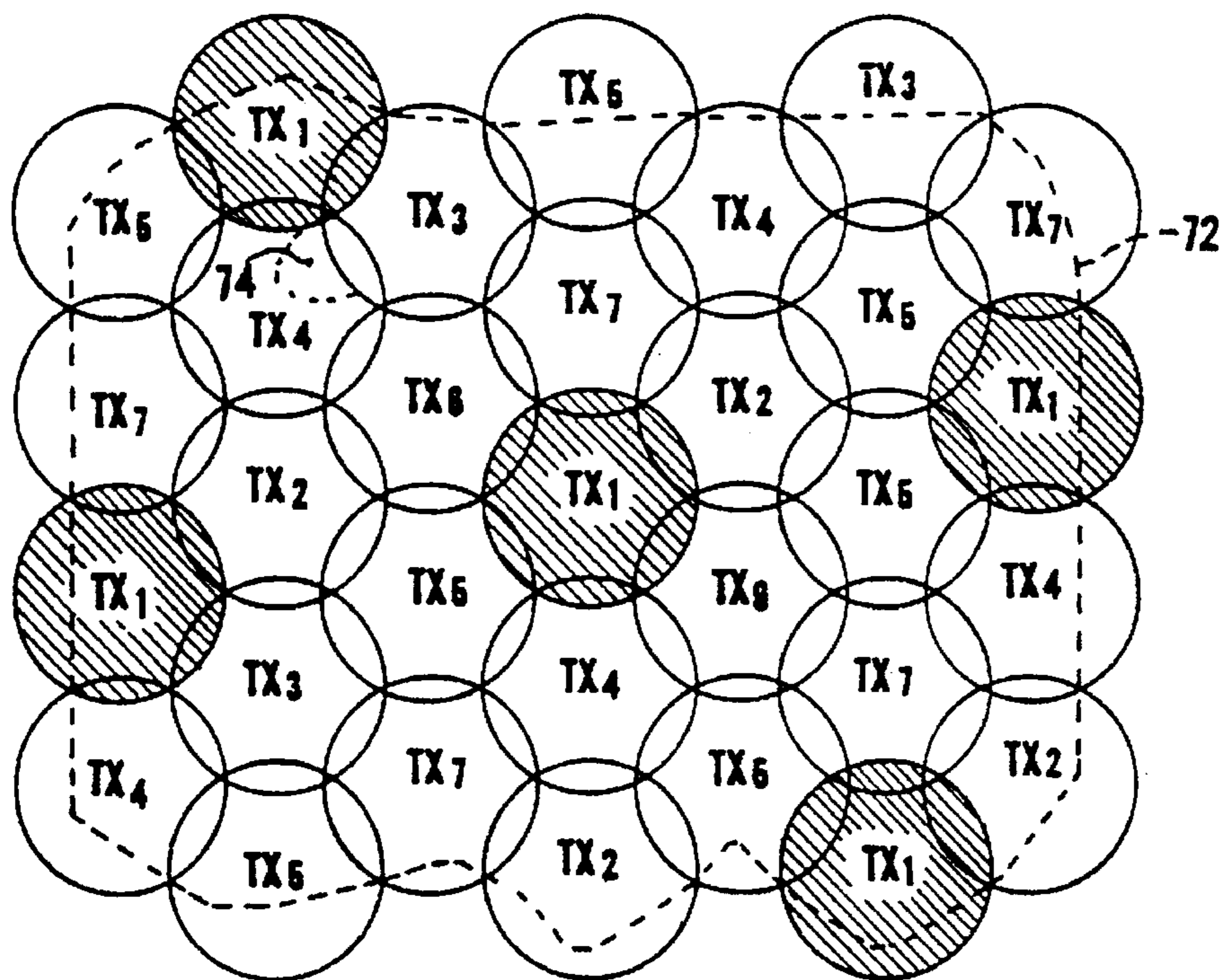
FIGURE 2 (PRIOR ART)
