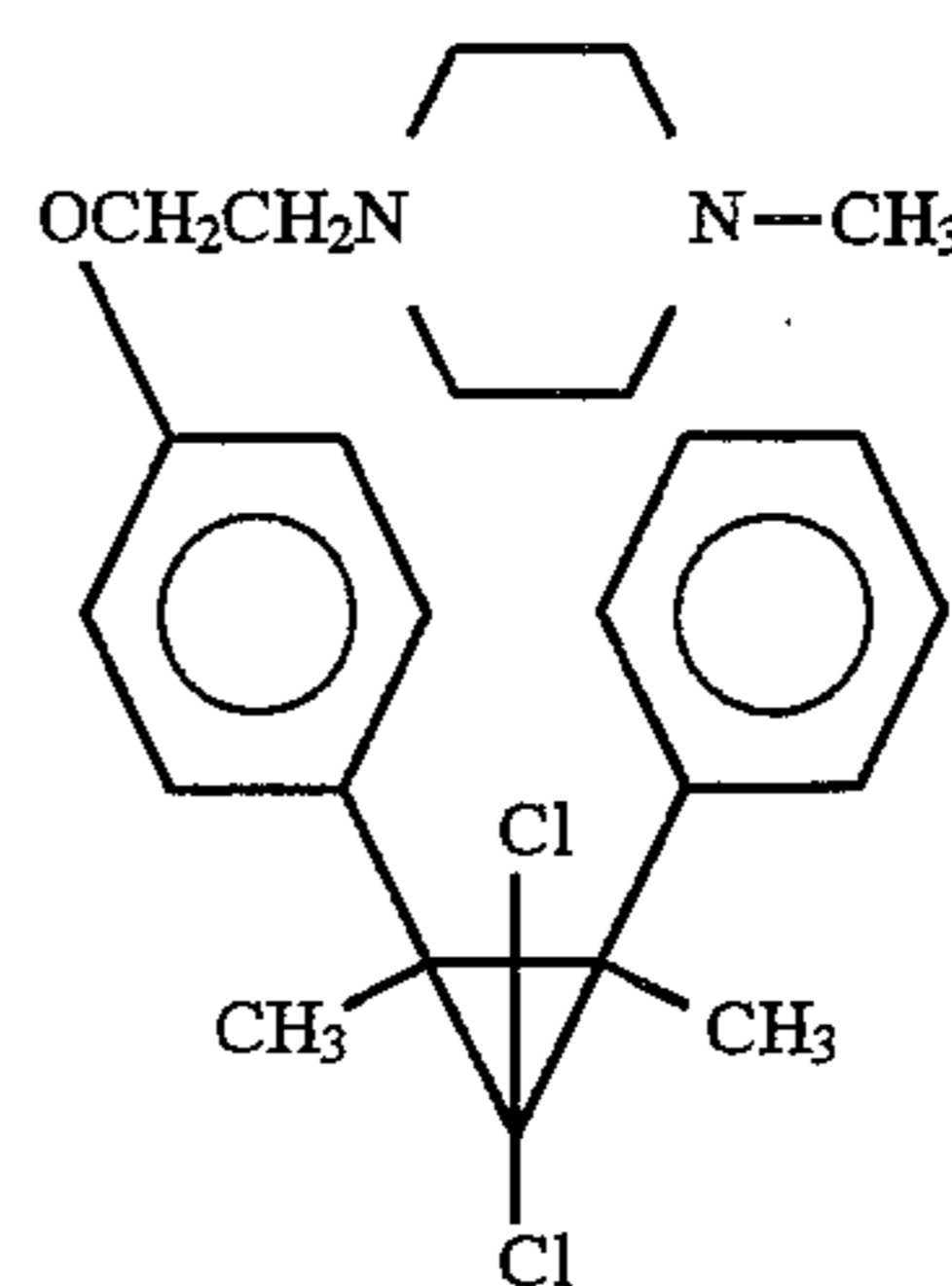
(Z)-1,1-Dichloro-2-[4-[2-(N-methylpiperazino)ethoxy]-phenyl]-2,3-dimethyl-3-phenylcyclopropane
