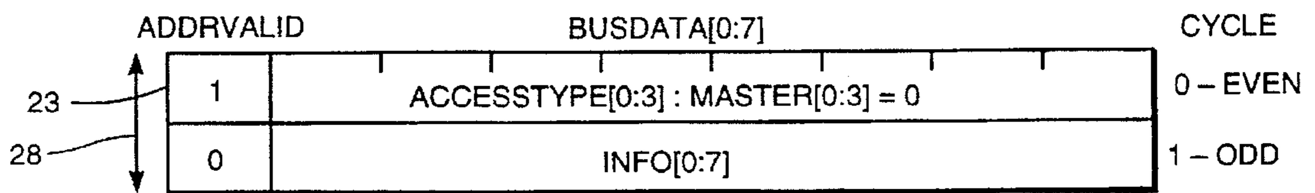
FIG. 5 REJECT (NACK) CONTROL PACKET
