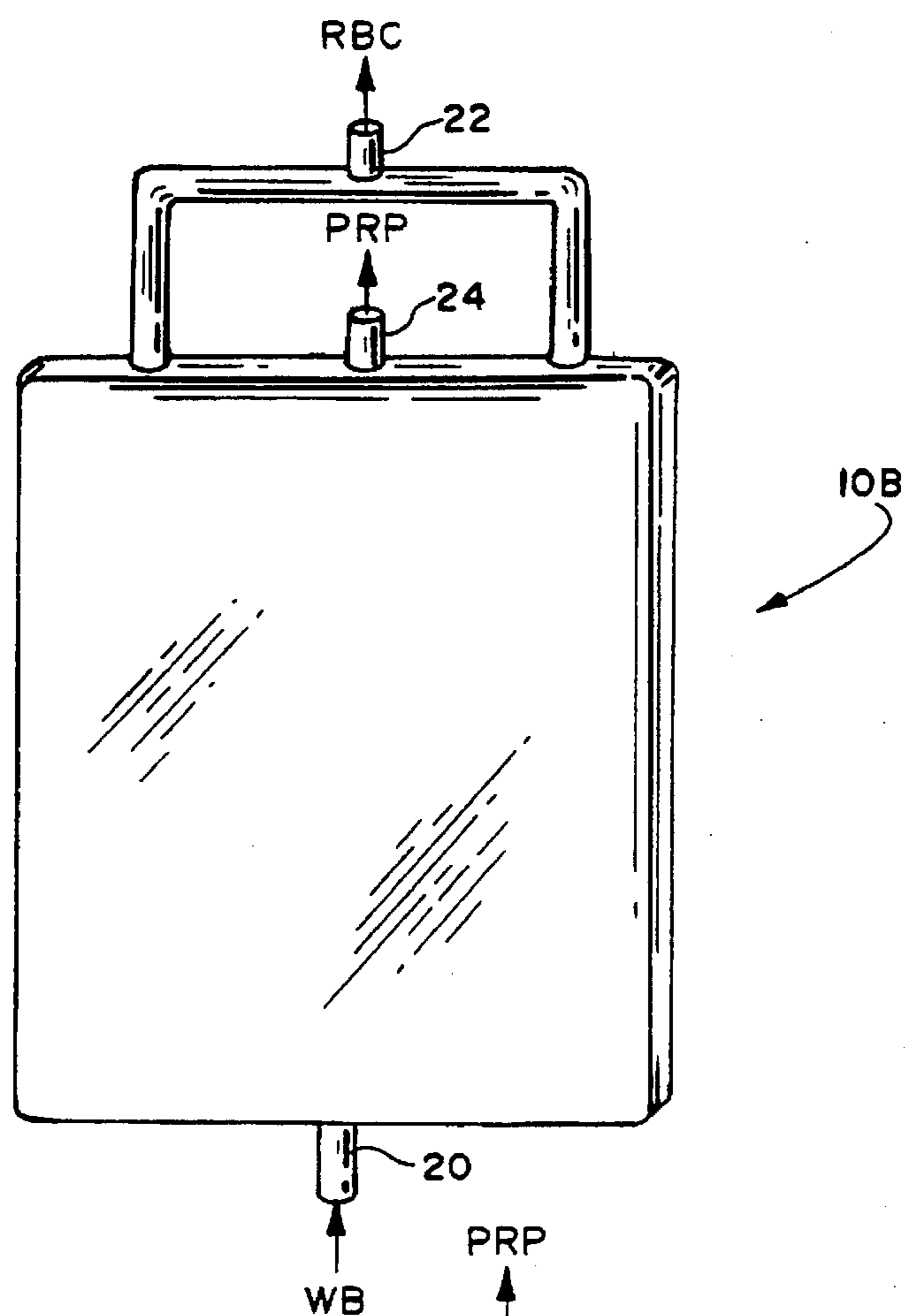
FIG. 4 PRIOR ART
