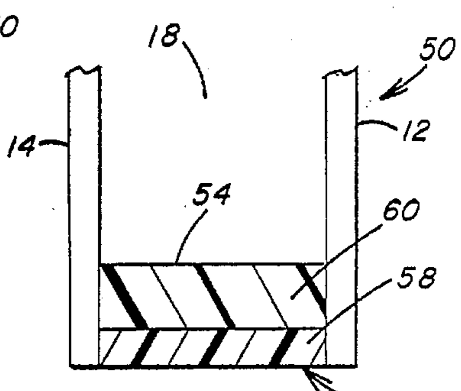
FIG. 3 PRIOR ART
