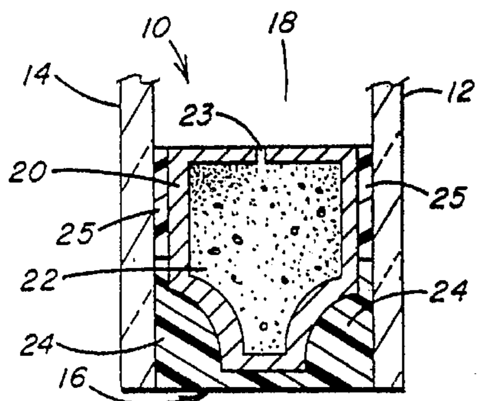
FIG. 1 PRIOR ART
