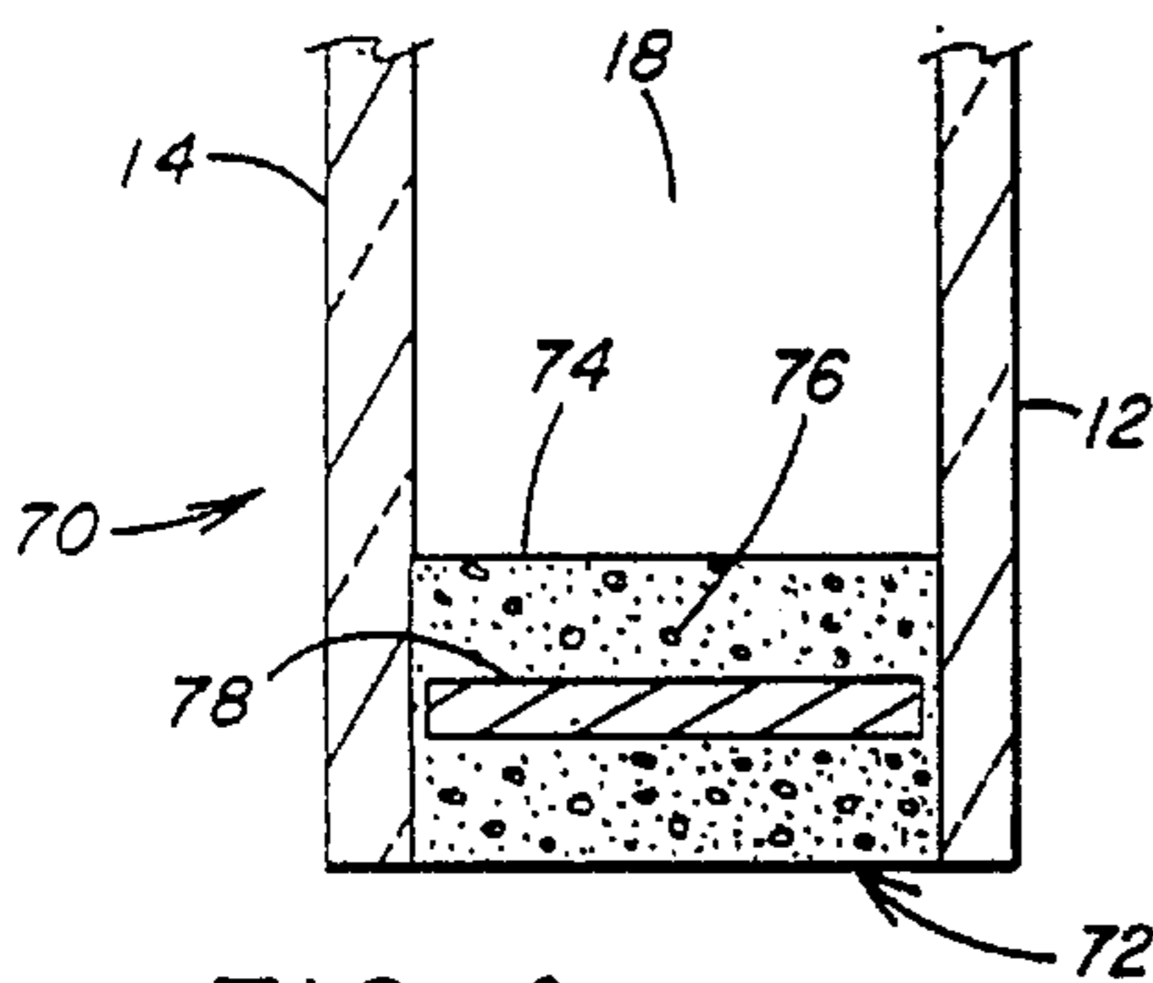
FIG. 4 PRIOR ART
