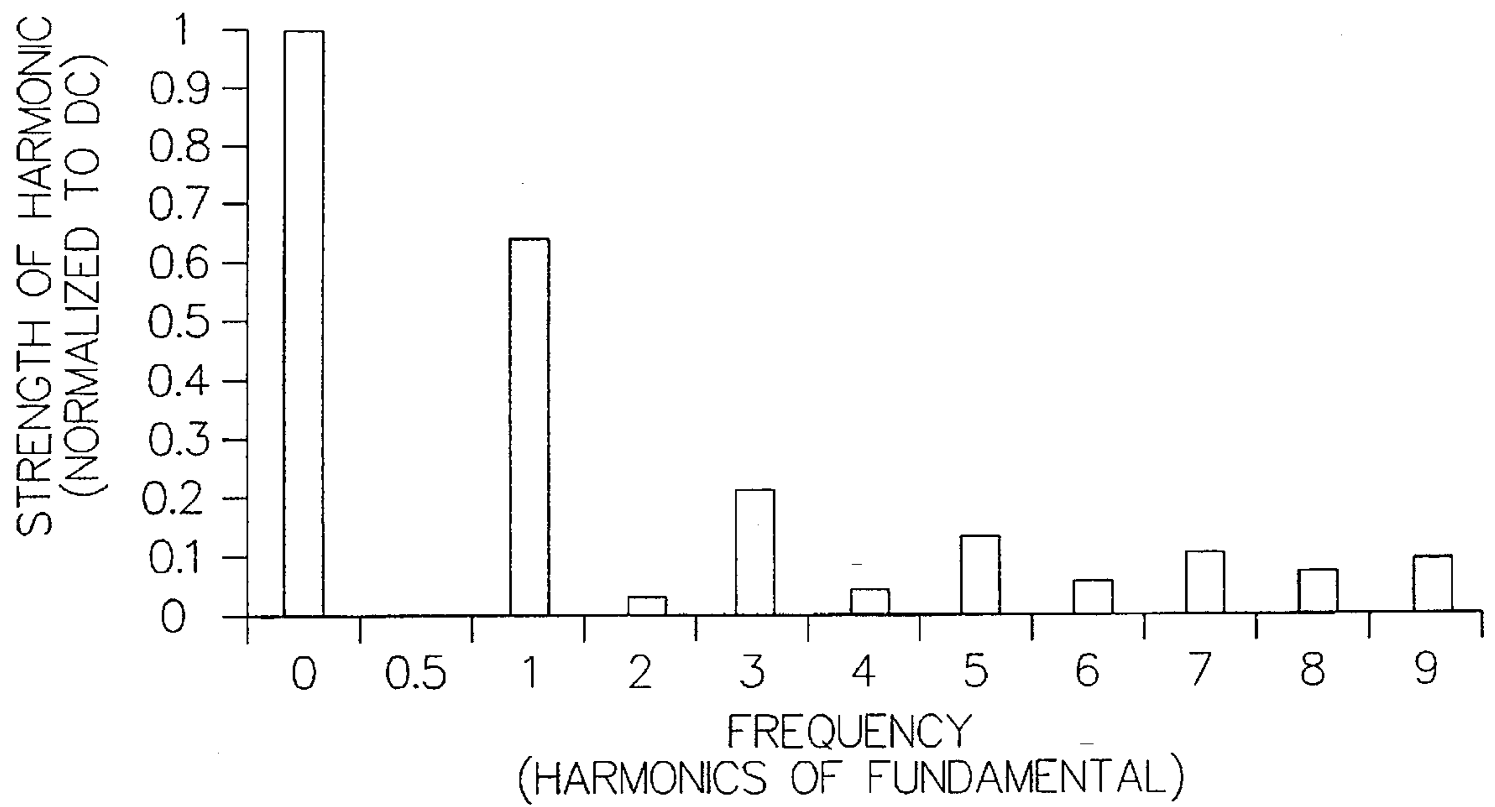
FFT FOLDBACK, MTF PAST SAMPLING FREQUENCY
