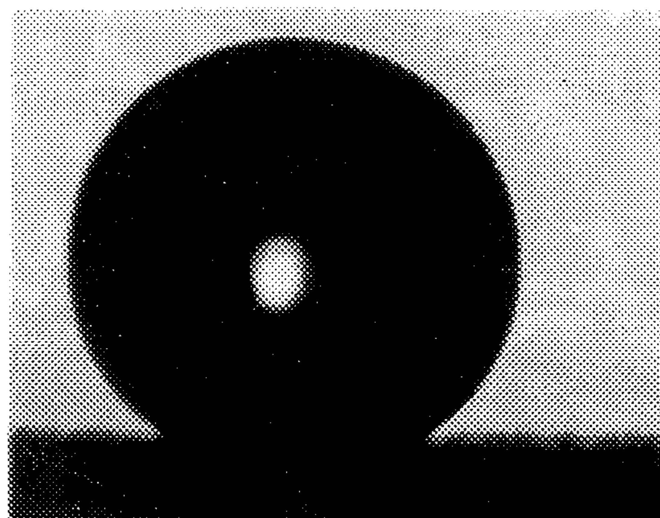
CONTACT ANGLE OF WATER WITH APD - FLUOROPOLYMER (145°)
