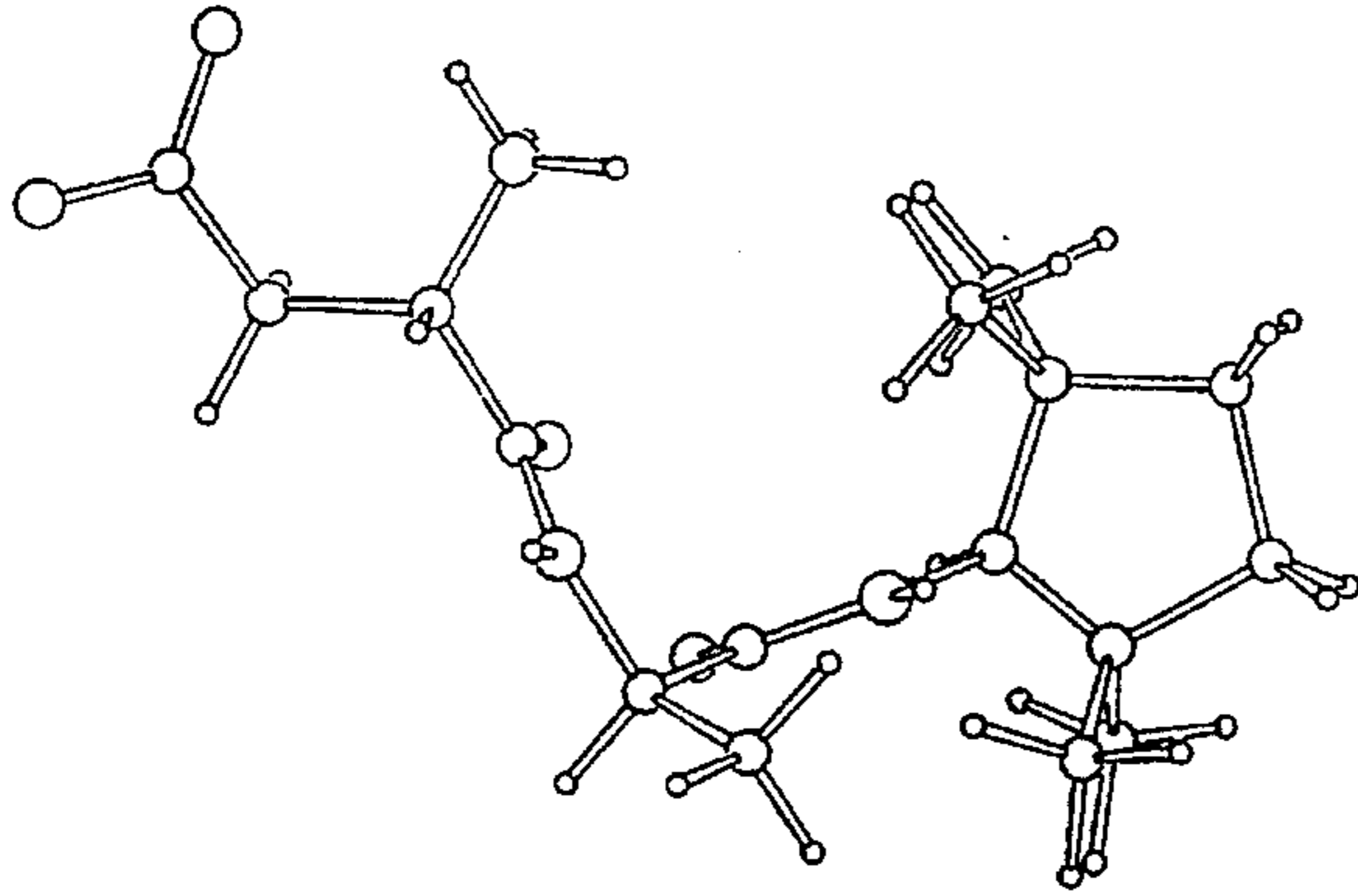
FIG. 2 a-d. Preferred minimum energy conformations of (A) N-(L-aspartyl)-N'-(tetramethylcyclopentanoyl)-(R)-1,1-diaminoethane, (B) (N-(L-aspartyl)-N'-(tetramethylcyclopentanoyl) (S)-1,1-diaminoethane, (C) L-aspartyl-D-alanyl-tetramethylcyclopentylamide and (D) L-aspartyl-L-alanyl-tetramethylcyclopentylamide.
