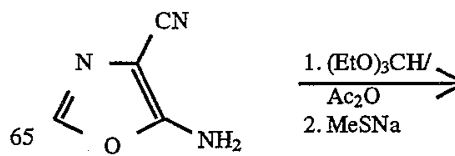
Scheme 25. Synthesis of Preferred Group 45; [5,4-d] ring fusion.
