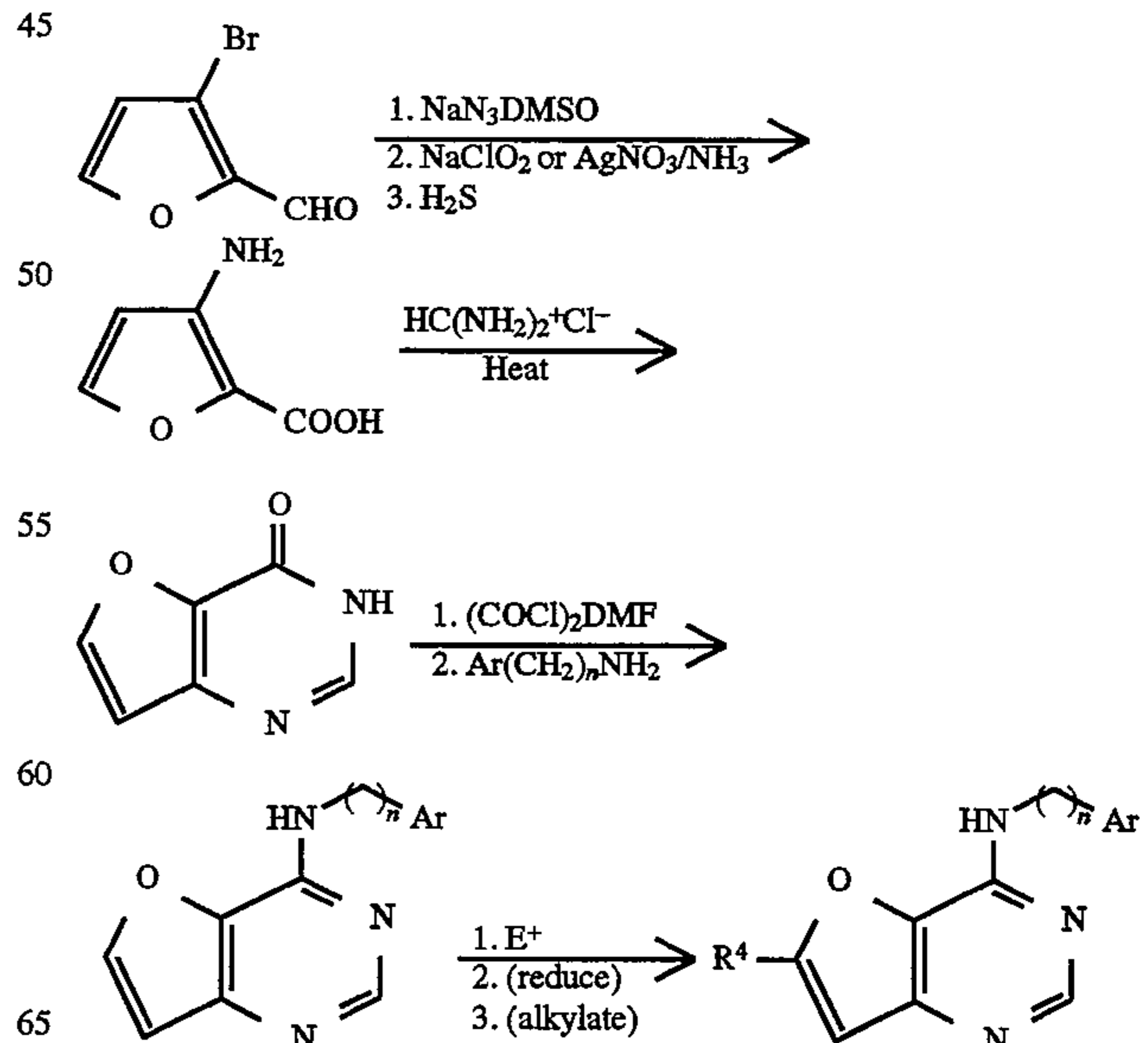
Synthesis of Preferred Group 42; [3,2-d] ring fusion
