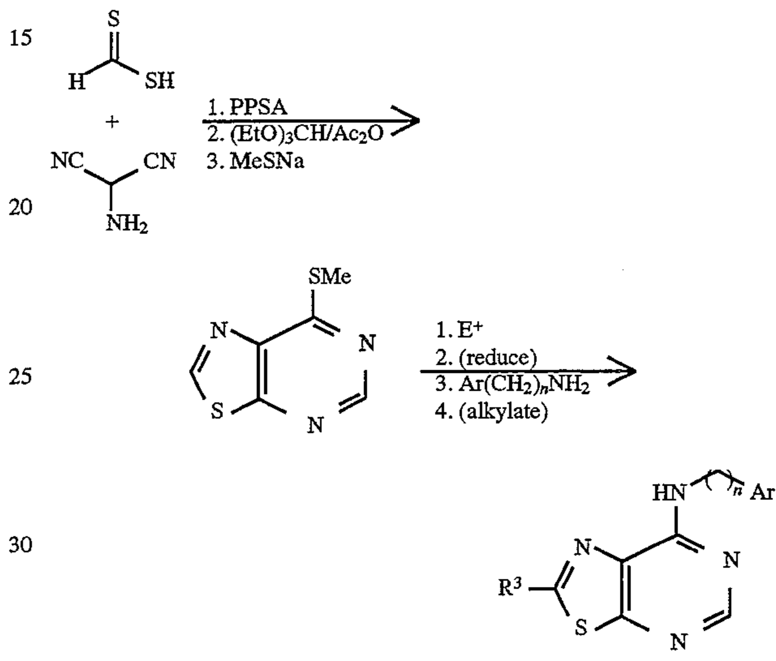
Scheme 23. Synthesis of Preferred Group 44; [5,4-d] ring fusion.
