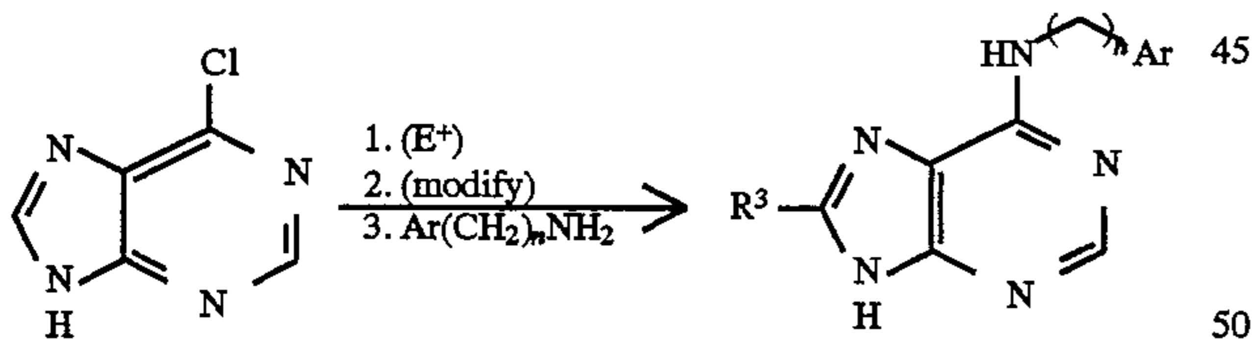
Scheme 27. Synthesis of Preferred Group 46.
