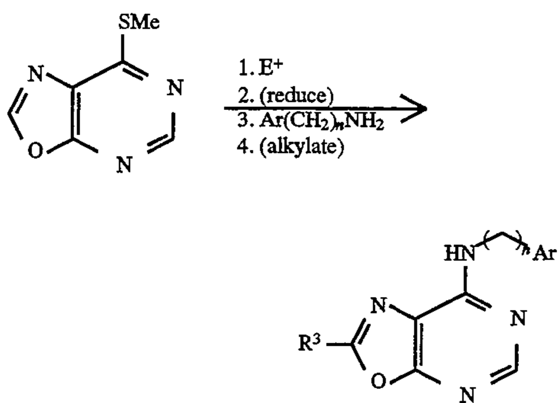
Scheme 25. Synthesis of Preferred Group 45; [5,4-d] ring fusion.
