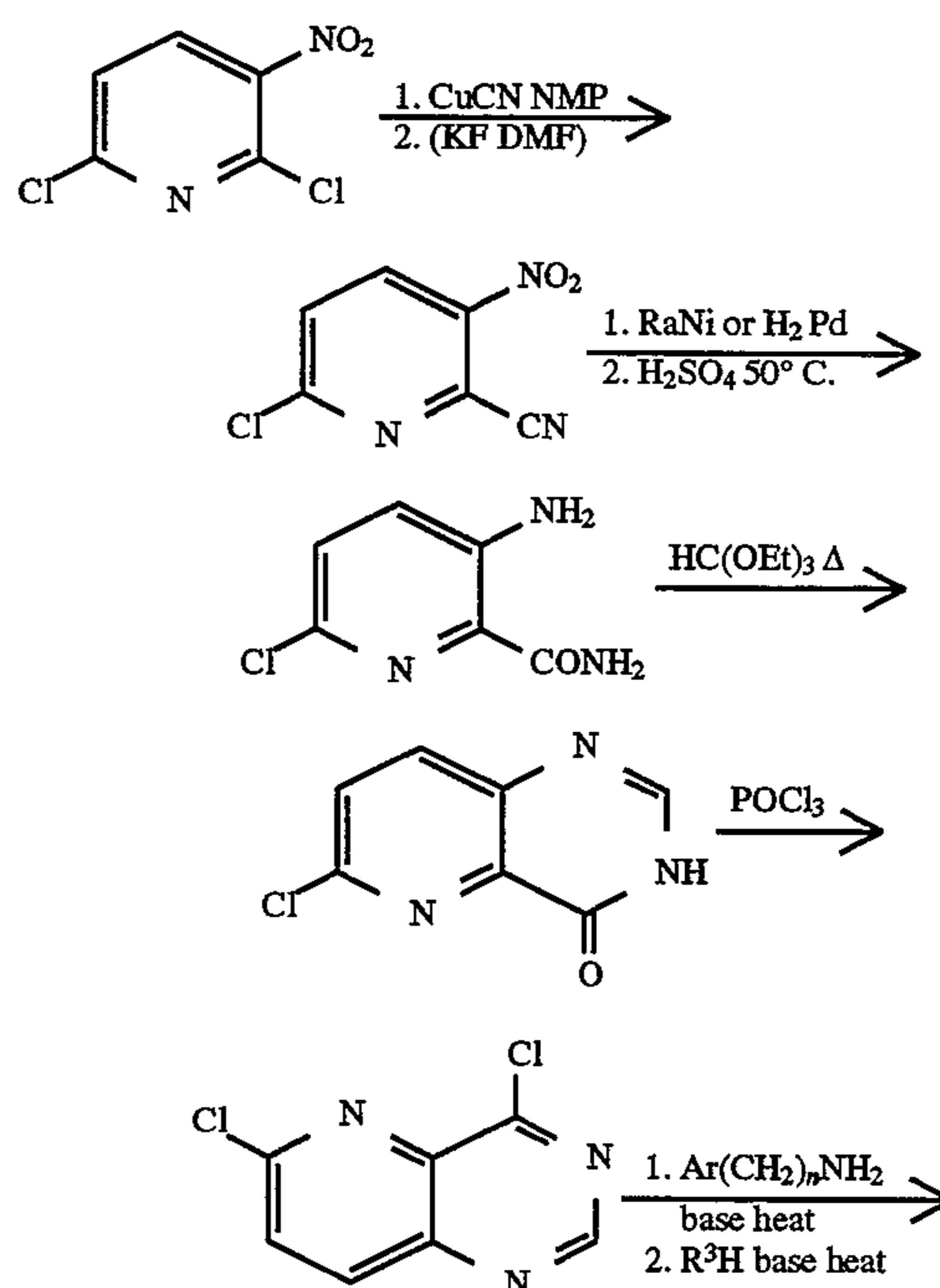
Scheme 1. Synthesis of Preferred Groups 1-5; R 4 = H
