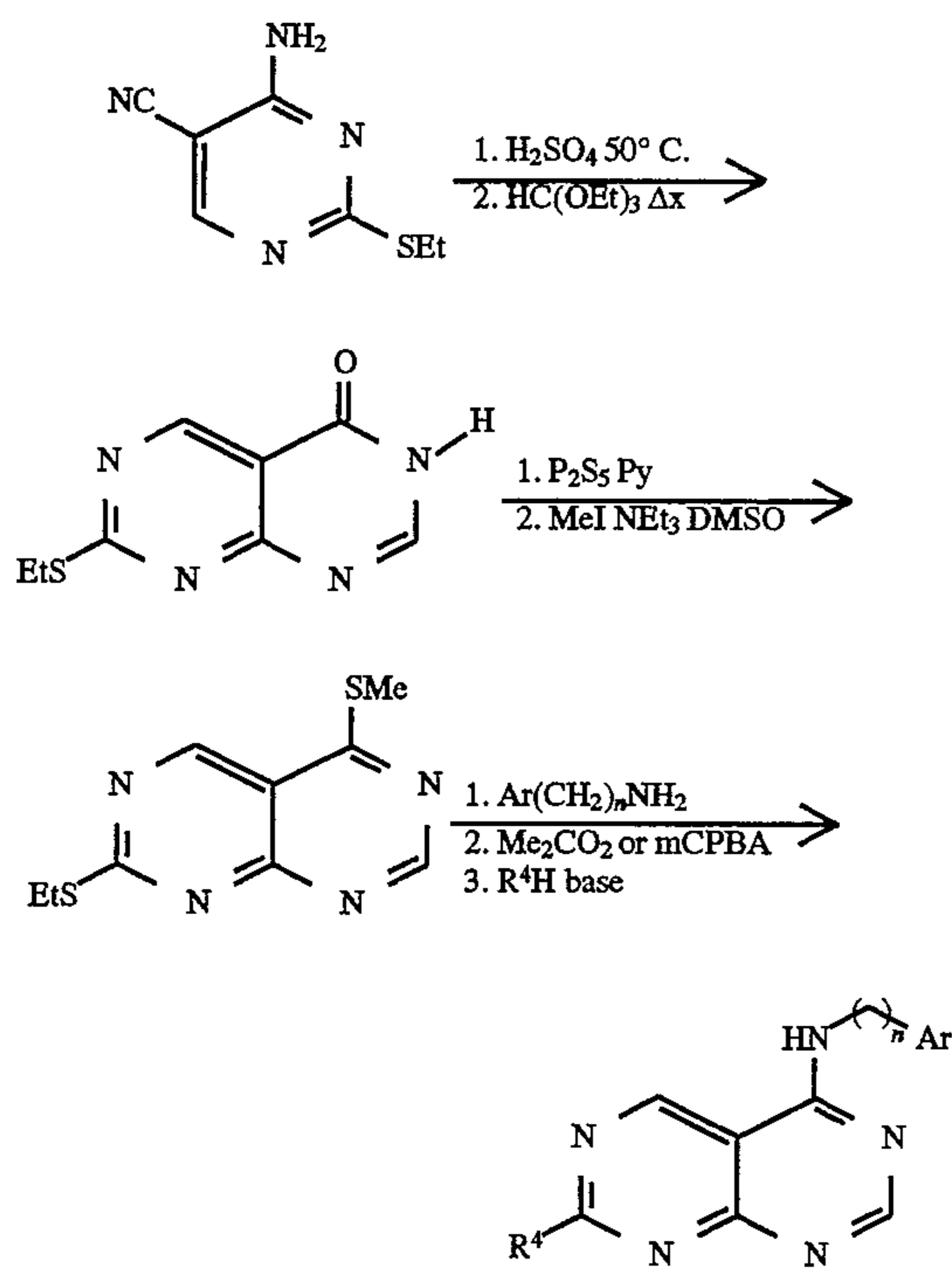
Scheme 15. Synthesis of Preferred Groups 33-36.
