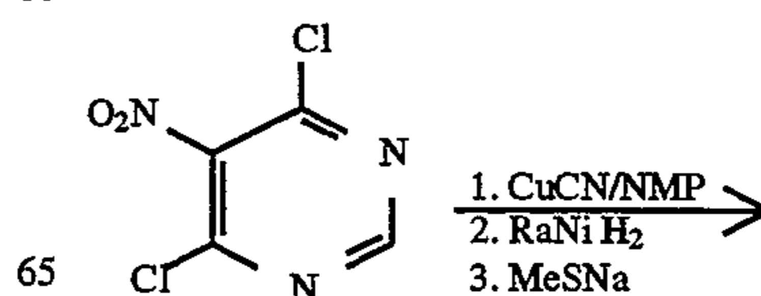
Scheme 31. Synthesis of Preferred Group 48; [4,5-d] ring fusion.
