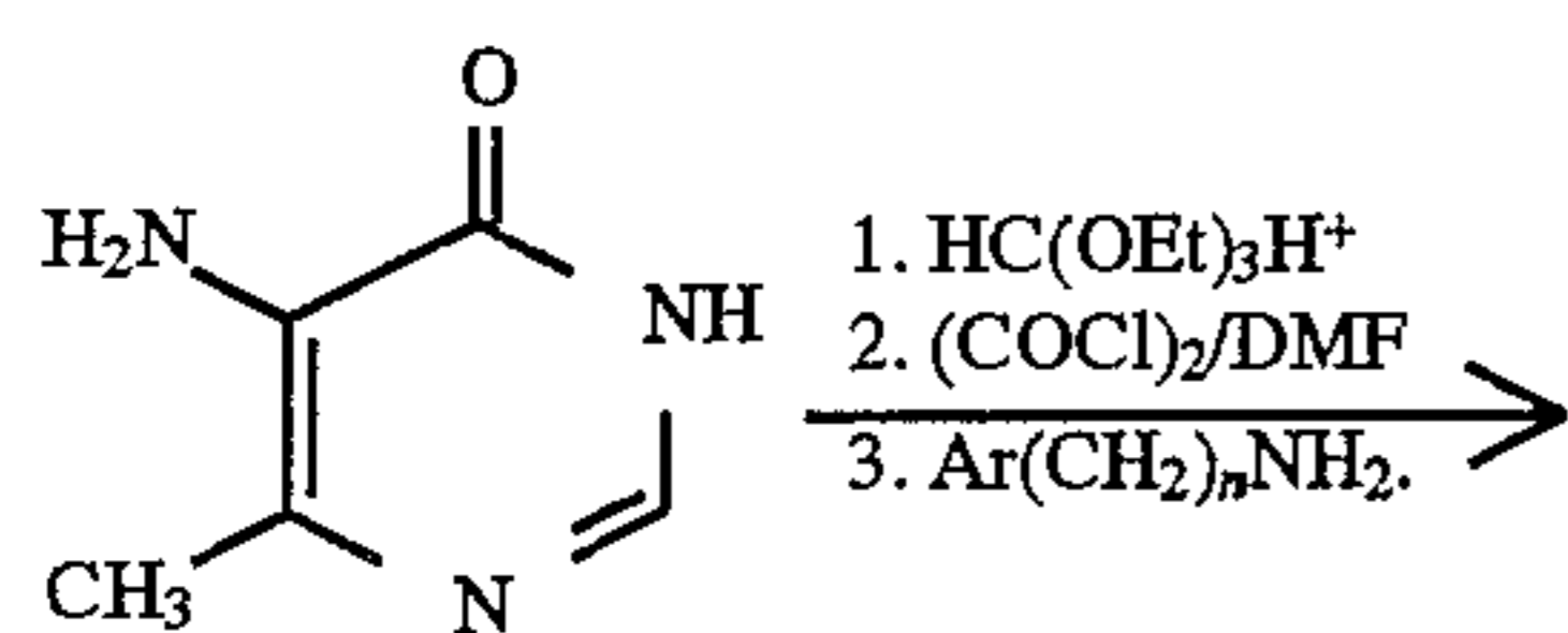
Scheme 22. Synthesis of Preferred Group 43; [2,3-d] ring fusion.
