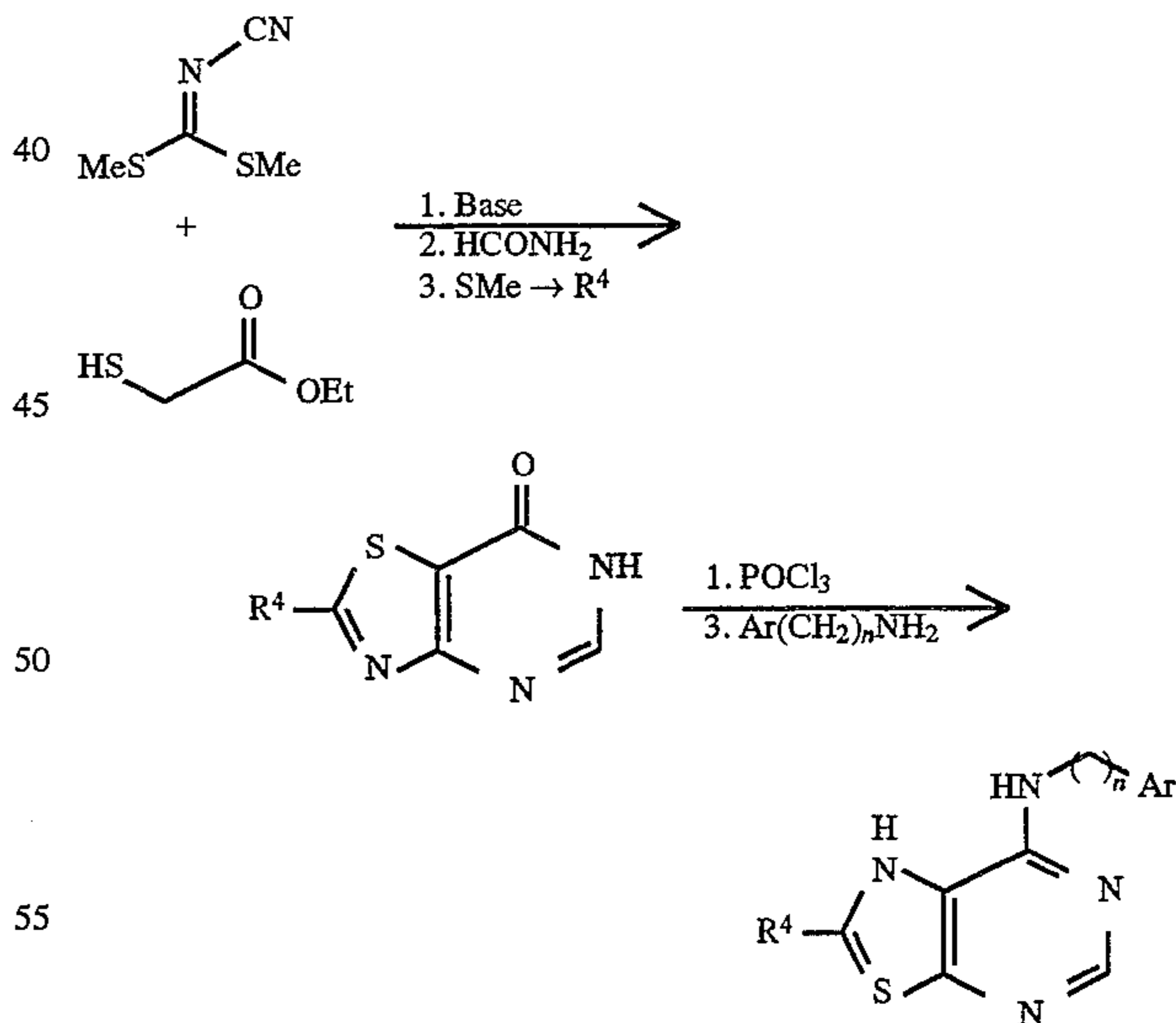
Scheme 24. Synthesis of Preferred Group 44; [4,5-d] ring fusion.
