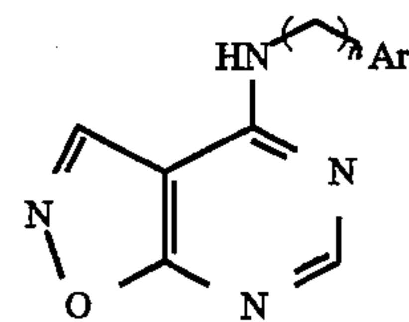
Scheme 28. Synthesis of Preferred Group 47; [5,4-d] ring fusion.
