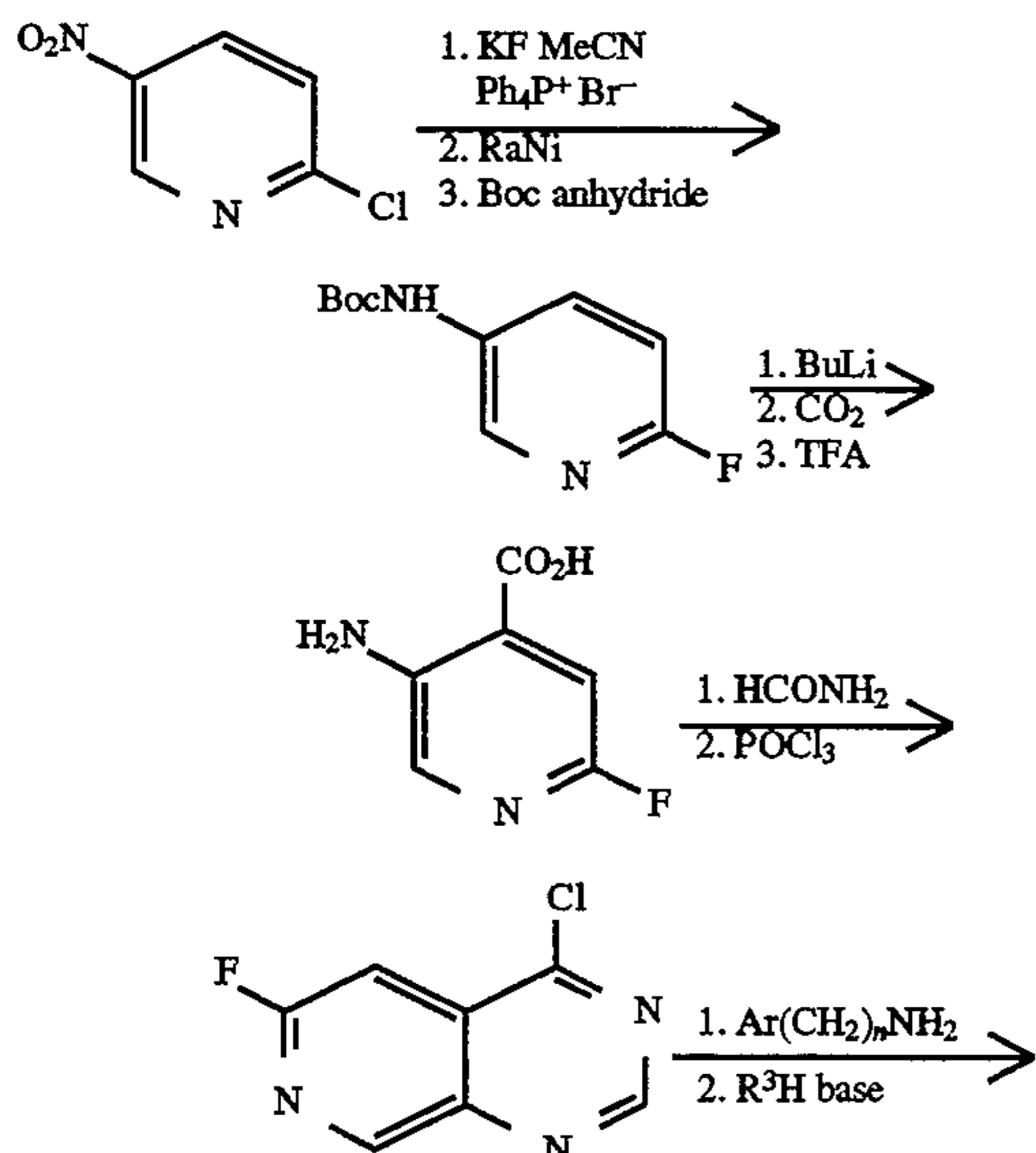
Scheme 8. Synthesis of Preferred Groups 17-21.
