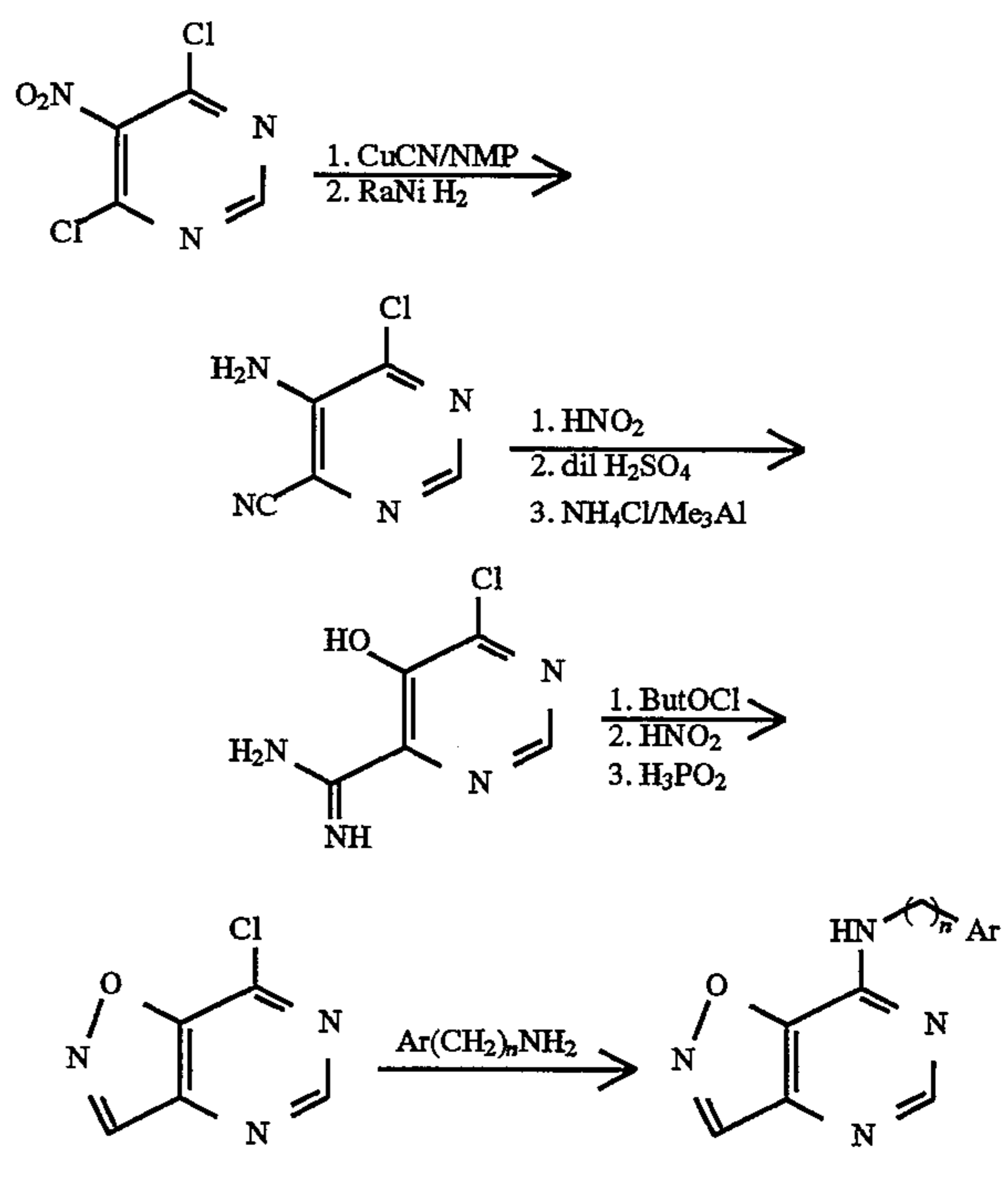
Scheme 29. Synthesis of Preferred Group 47; [4,5-d] ring fusion.
