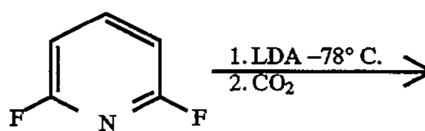
Scheme 10. Synthesis of Preferred Groups 22-26; R 3 = H.
