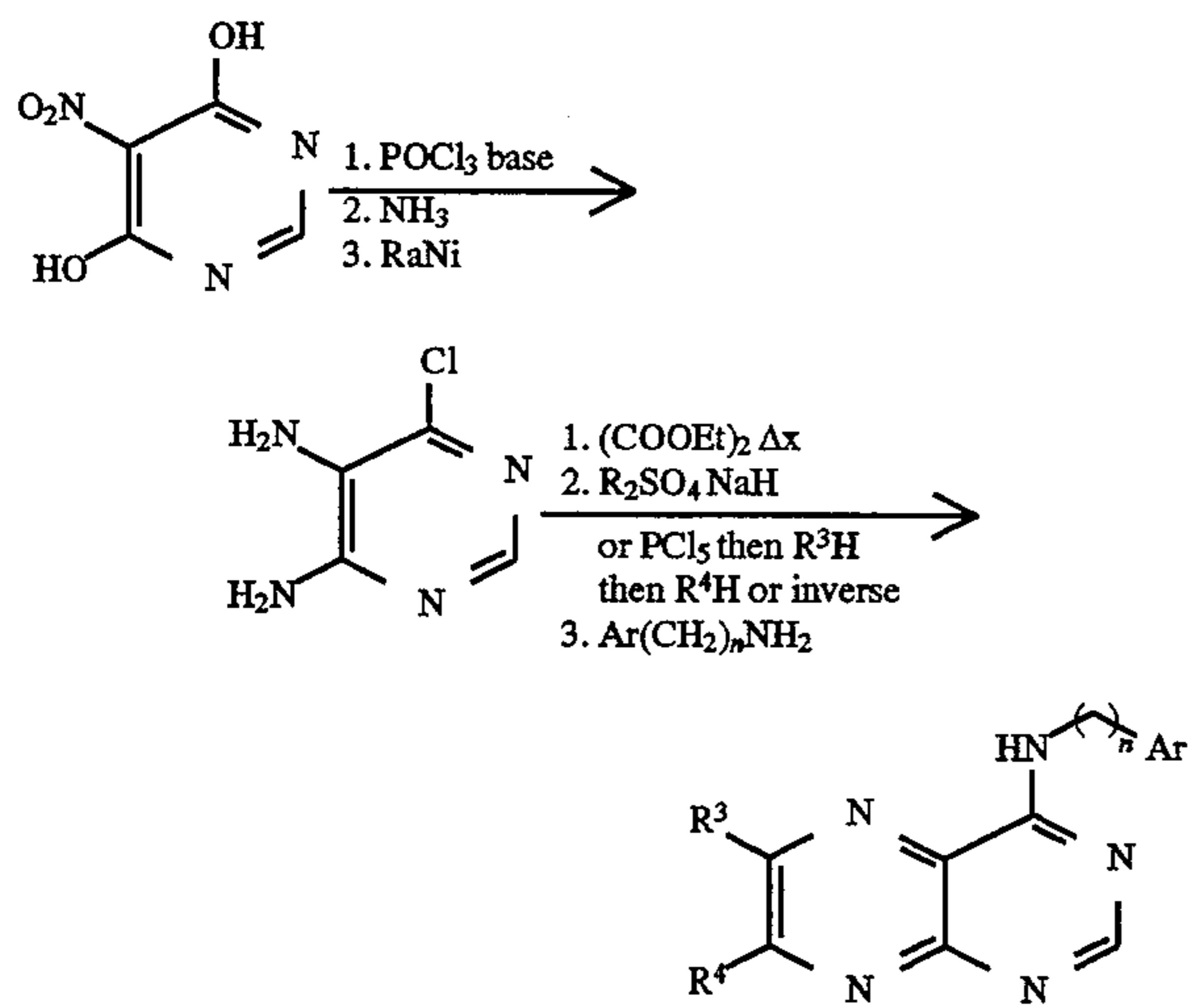
Scheme 16. Synthesis of Preferred Groups 37-40.
