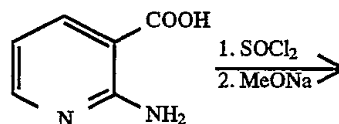
Scheme 9. Synthesis of Preferred Groups 22-26; R 4 = H.
