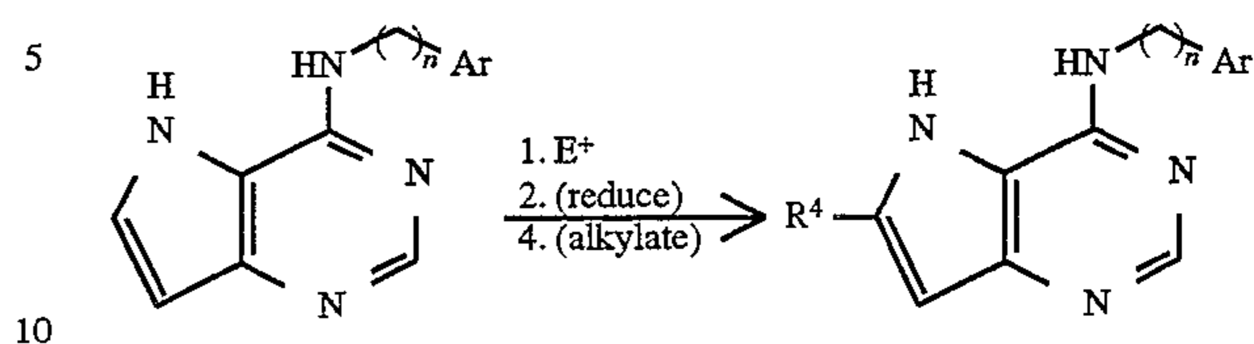
Scheme 22. Synthesis of Preferred Group 43; [2,3-d] ring fusion.
