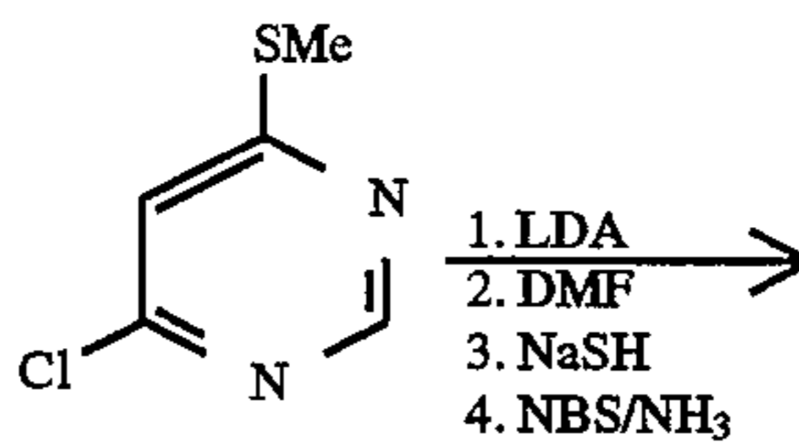
Scheme 30. Synthesis of Preferred Group 48; [5,4-d] ring fusion.
