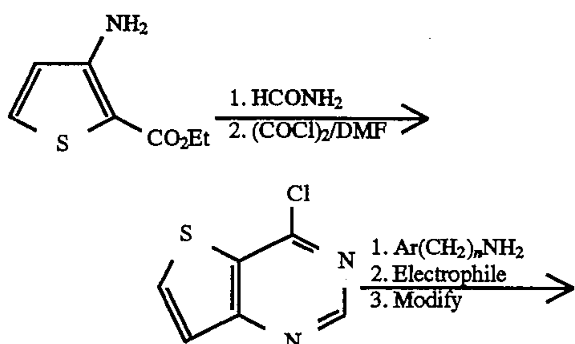
Scheme 17. Synthesis of Preferred Group 41; [3,2-d] ring fusion
