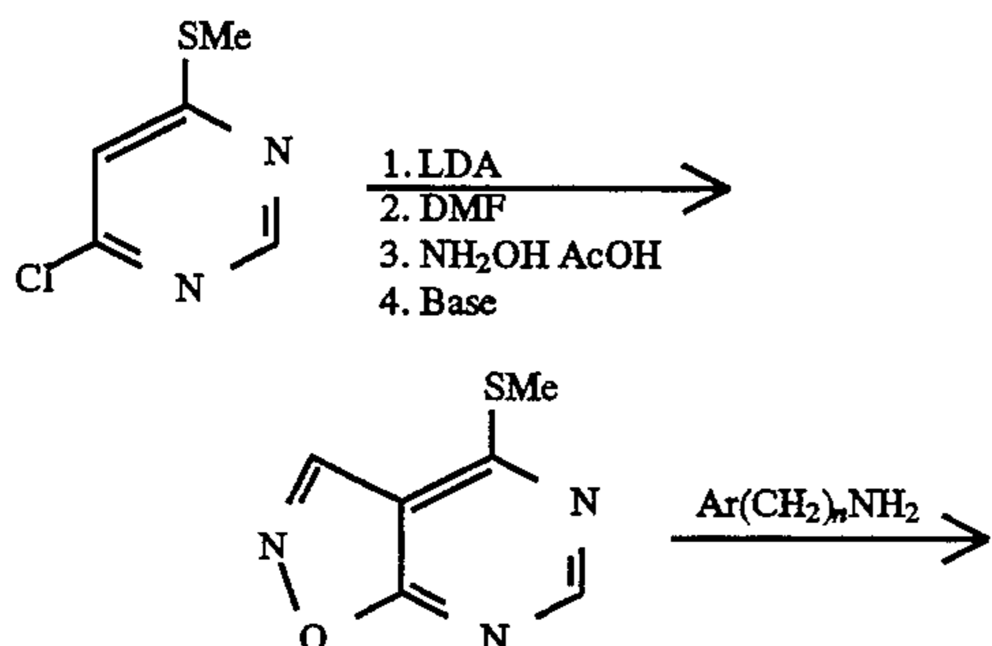
Scheme 28. Synthesis of Preferred Group 47; [5,4-d] ring fusion.
