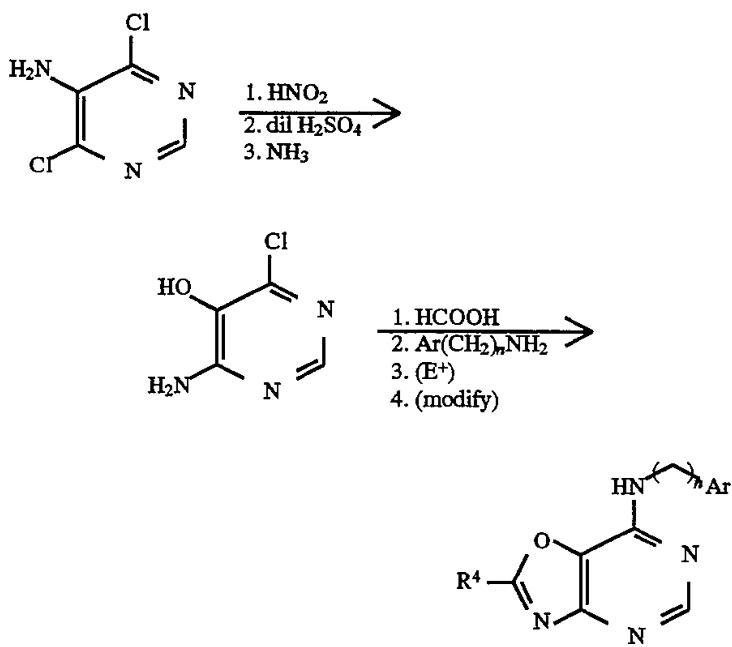
Scheme 26. Synthesis of Preferred Group 45; [4,5-d] ring fusion.
