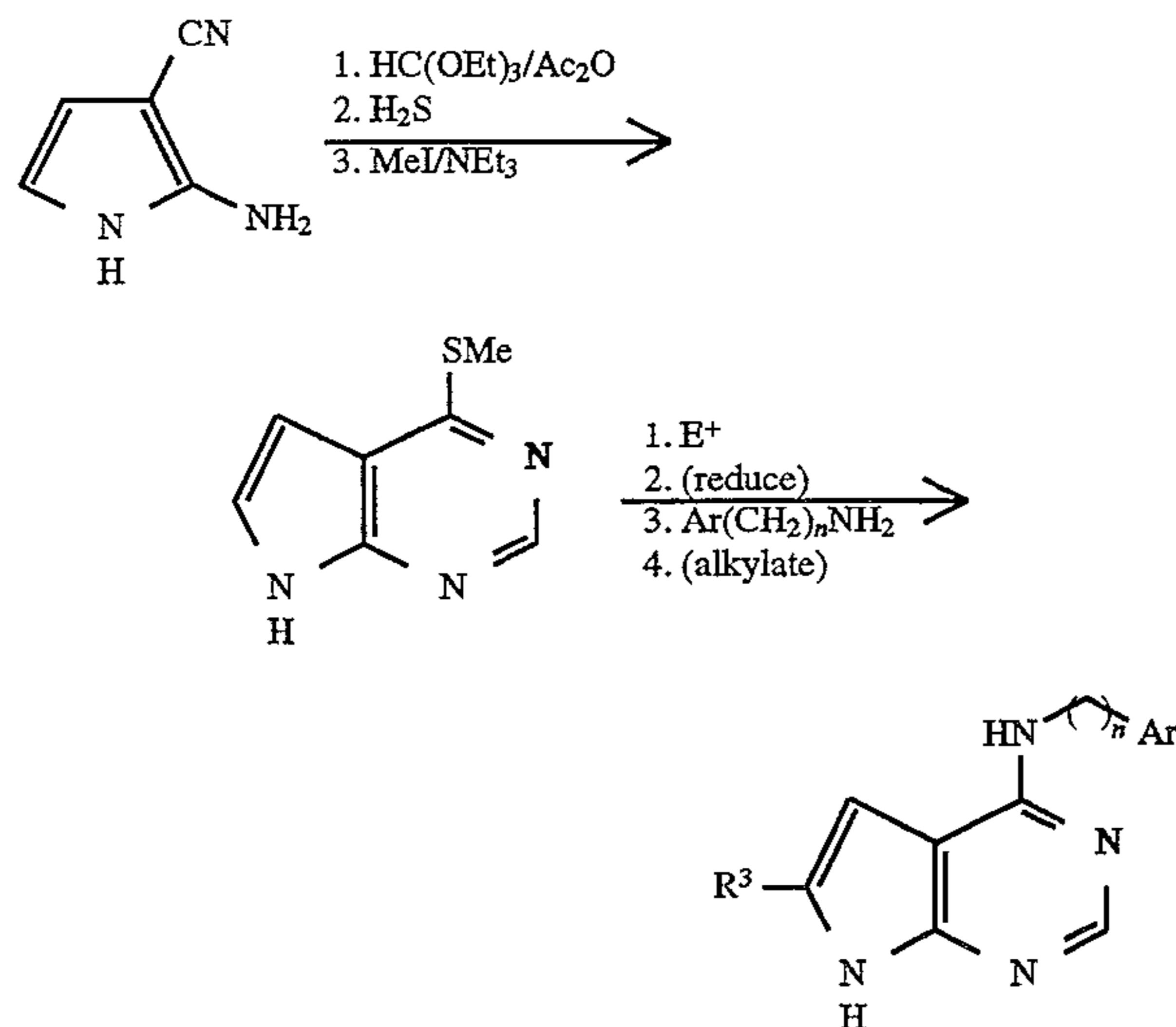
Scheme 21. Synthesis of Preferred Group 43; [2,3-d] ring fusion.
