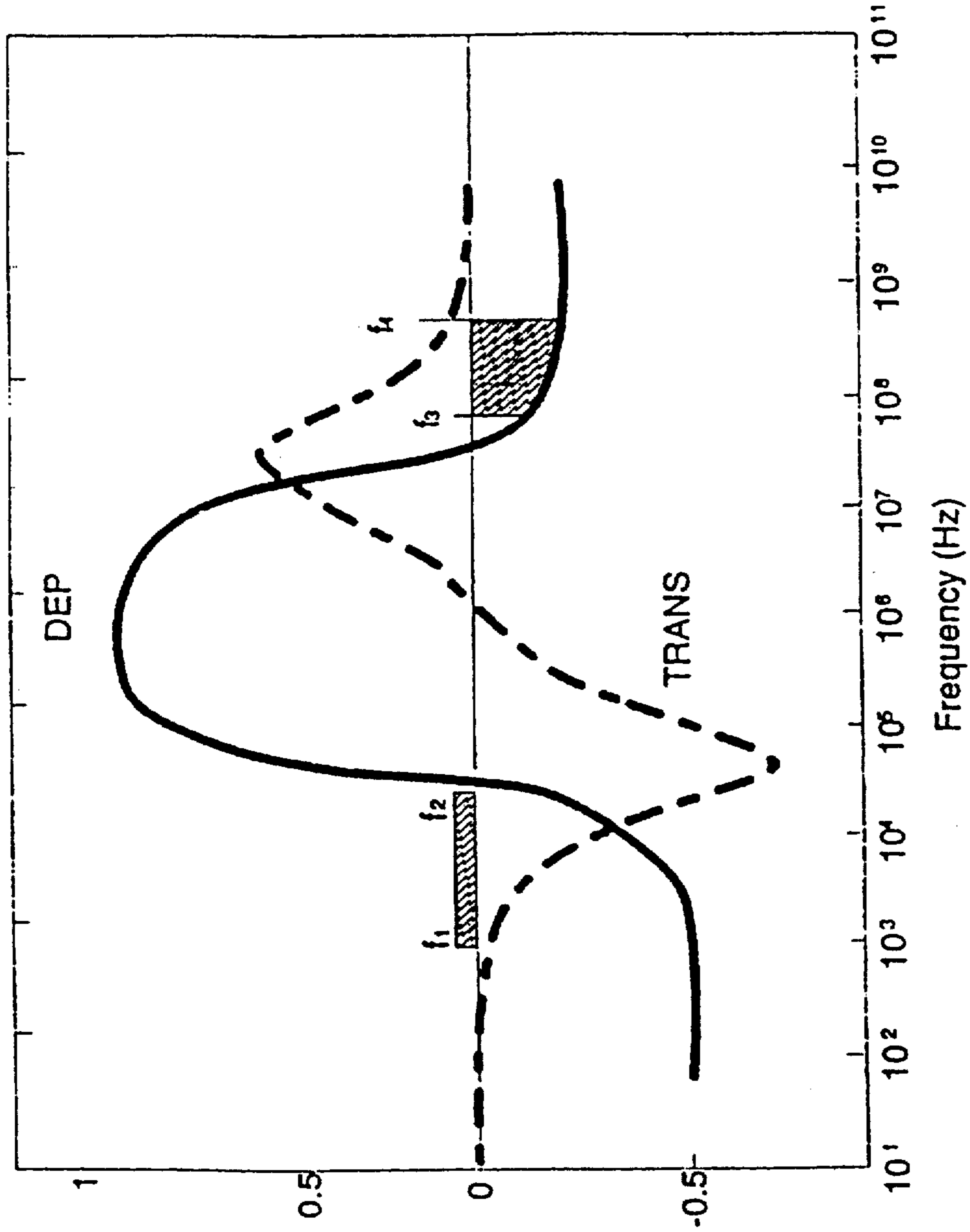
Dielectrophoresis and Electrorotation Spectra (arbitrary units)
