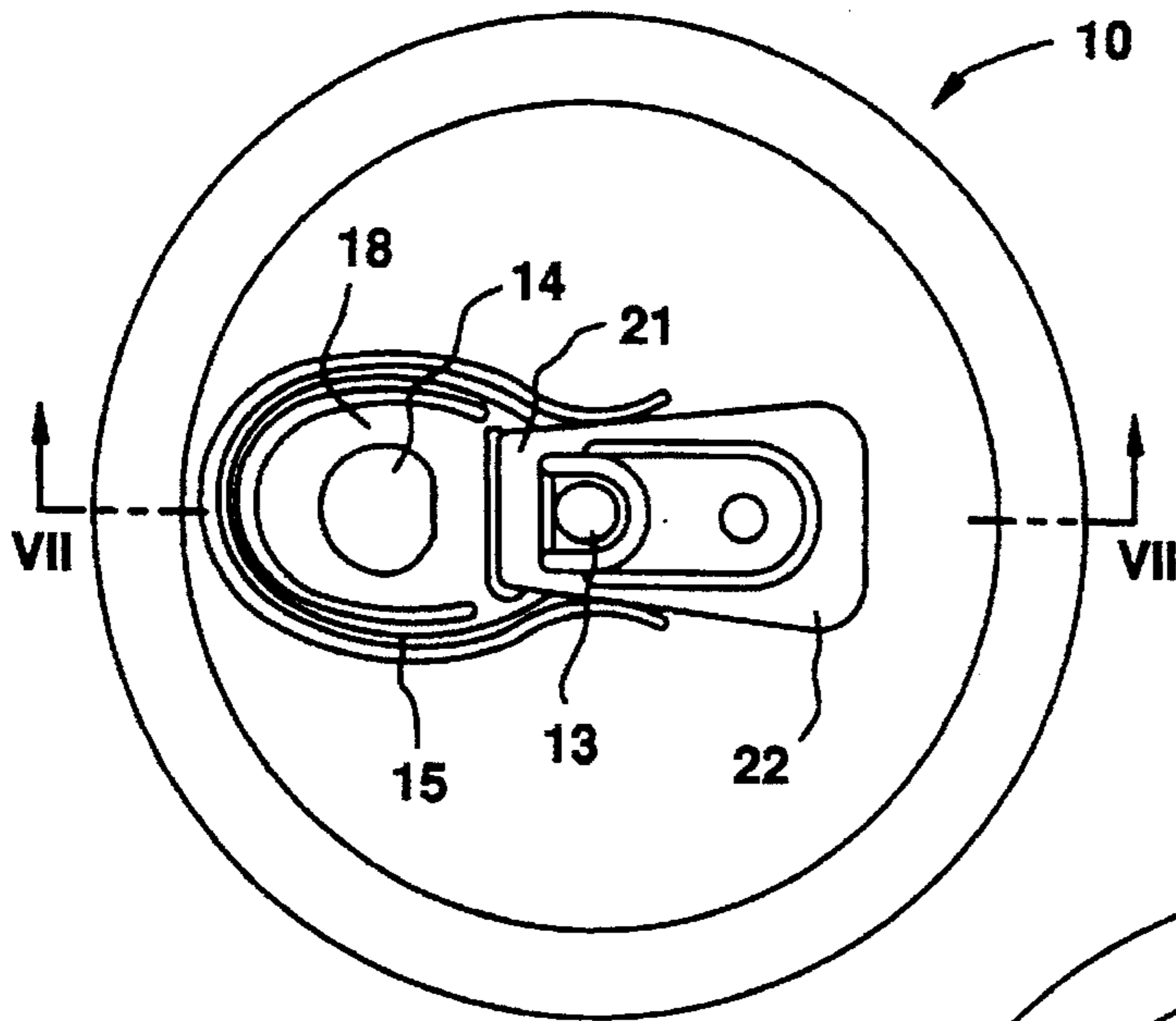
FIG.5 PRIOR ART
