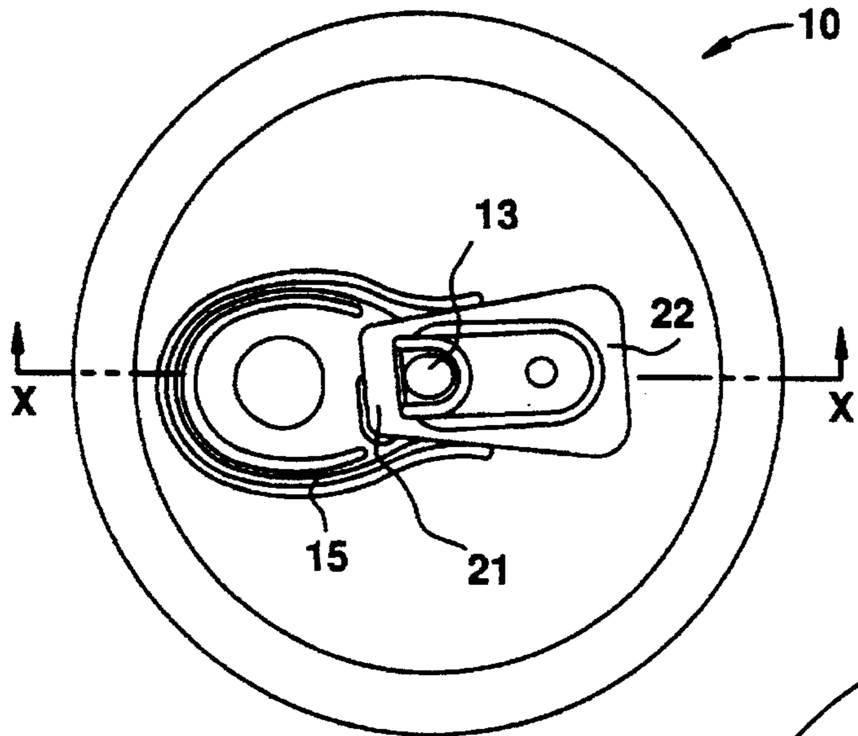
FIG. 8 PRIOR ART
